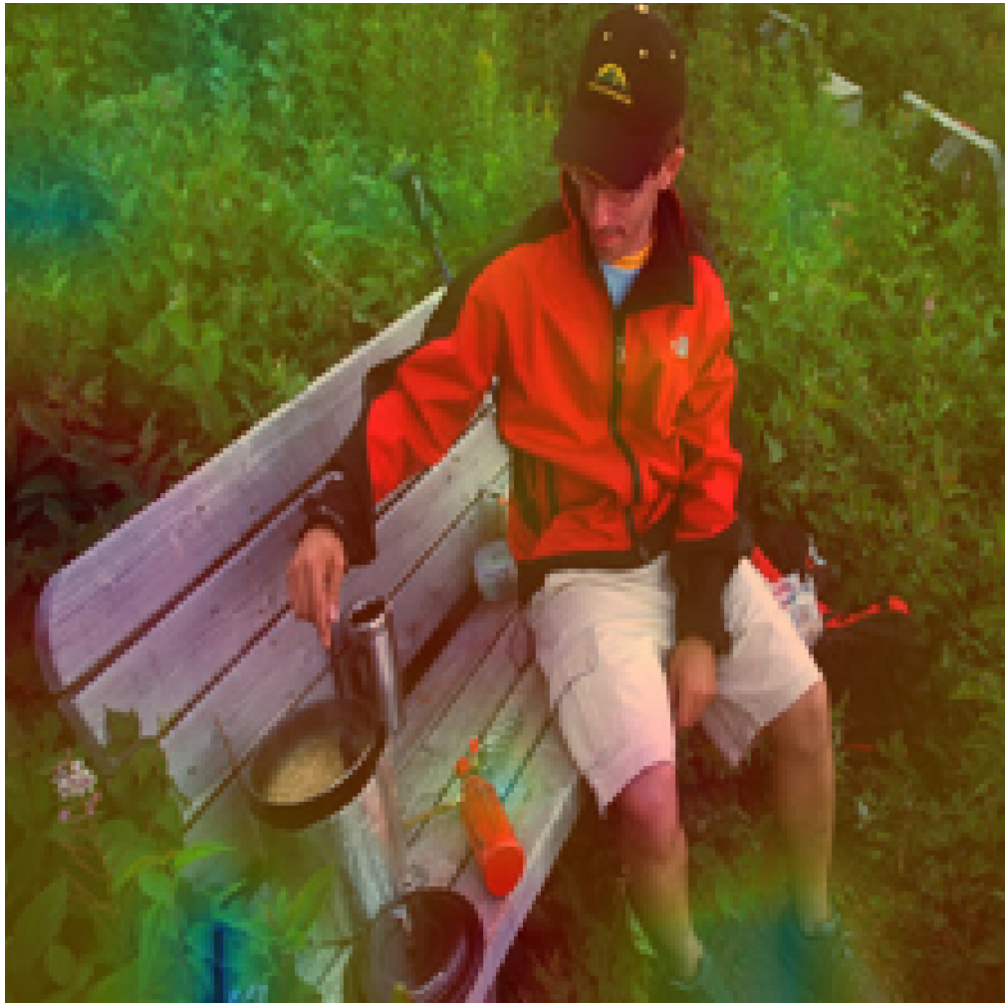
Head 9
