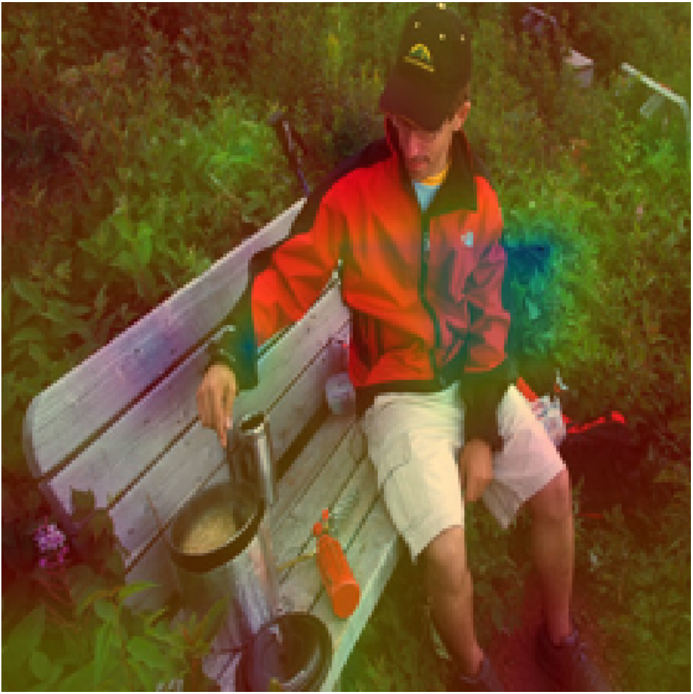
Head 12
