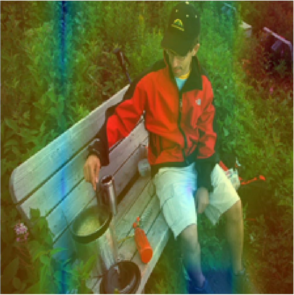
Head 11
