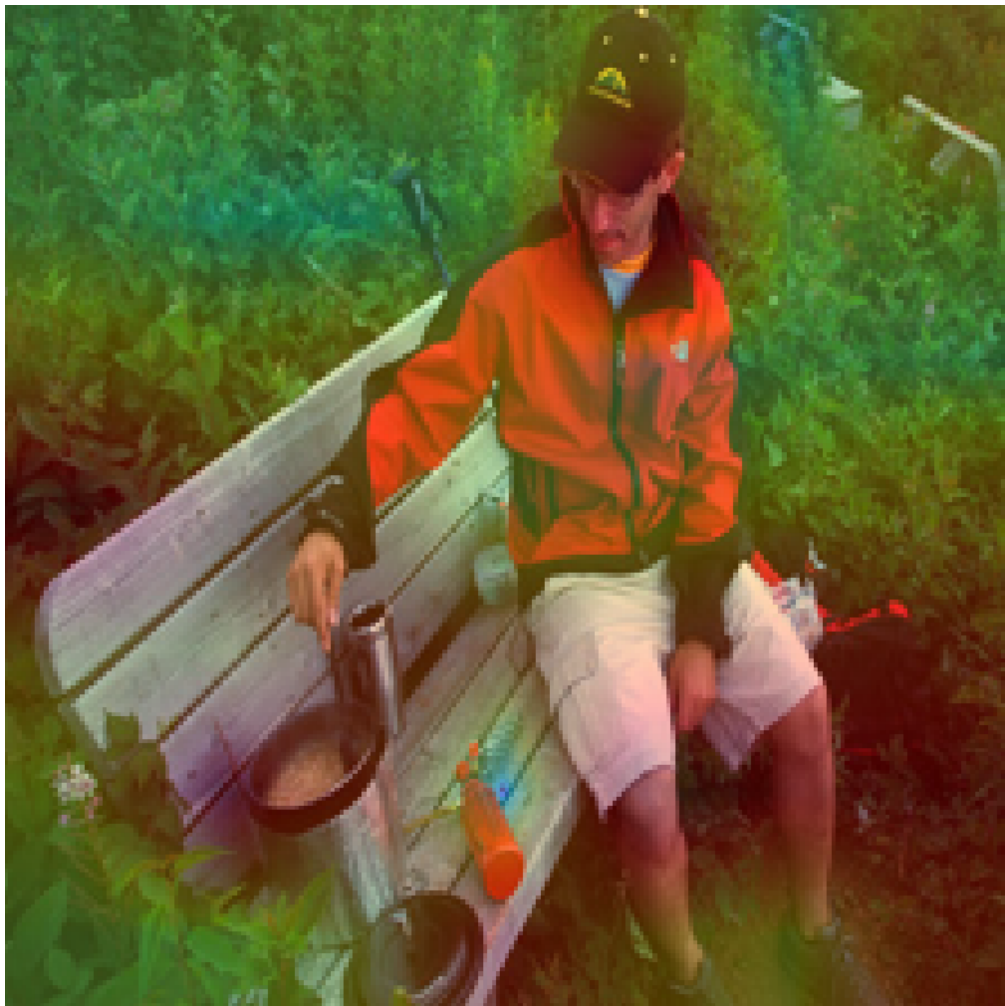
Head 5
