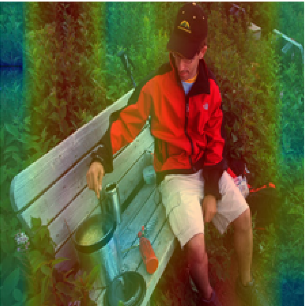
Head 7
