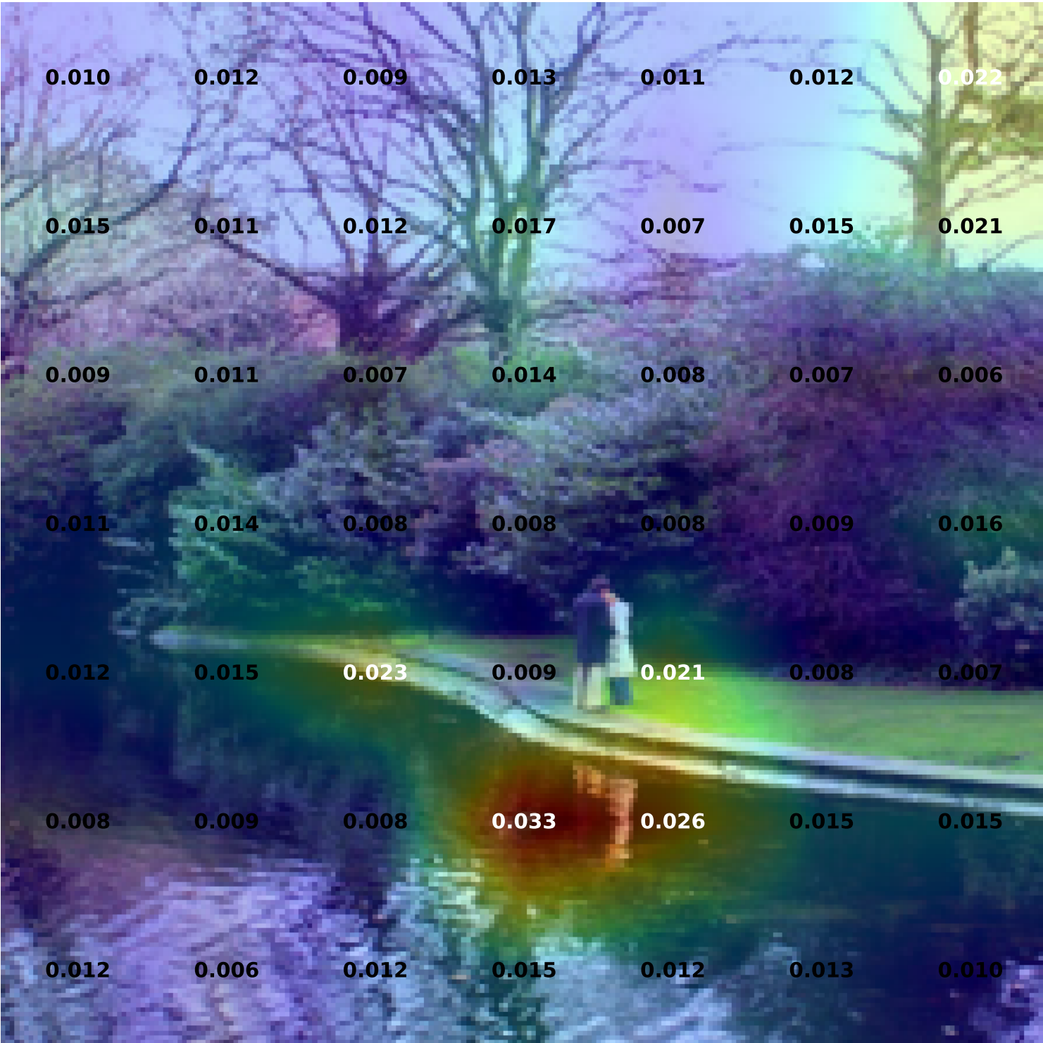
3637013_c675de7705 [vanilla] — Layer 1, Head 1 CLS attention overlay (values) \mu = 0.01245 \sigma = 0.005357 (49 patches)
