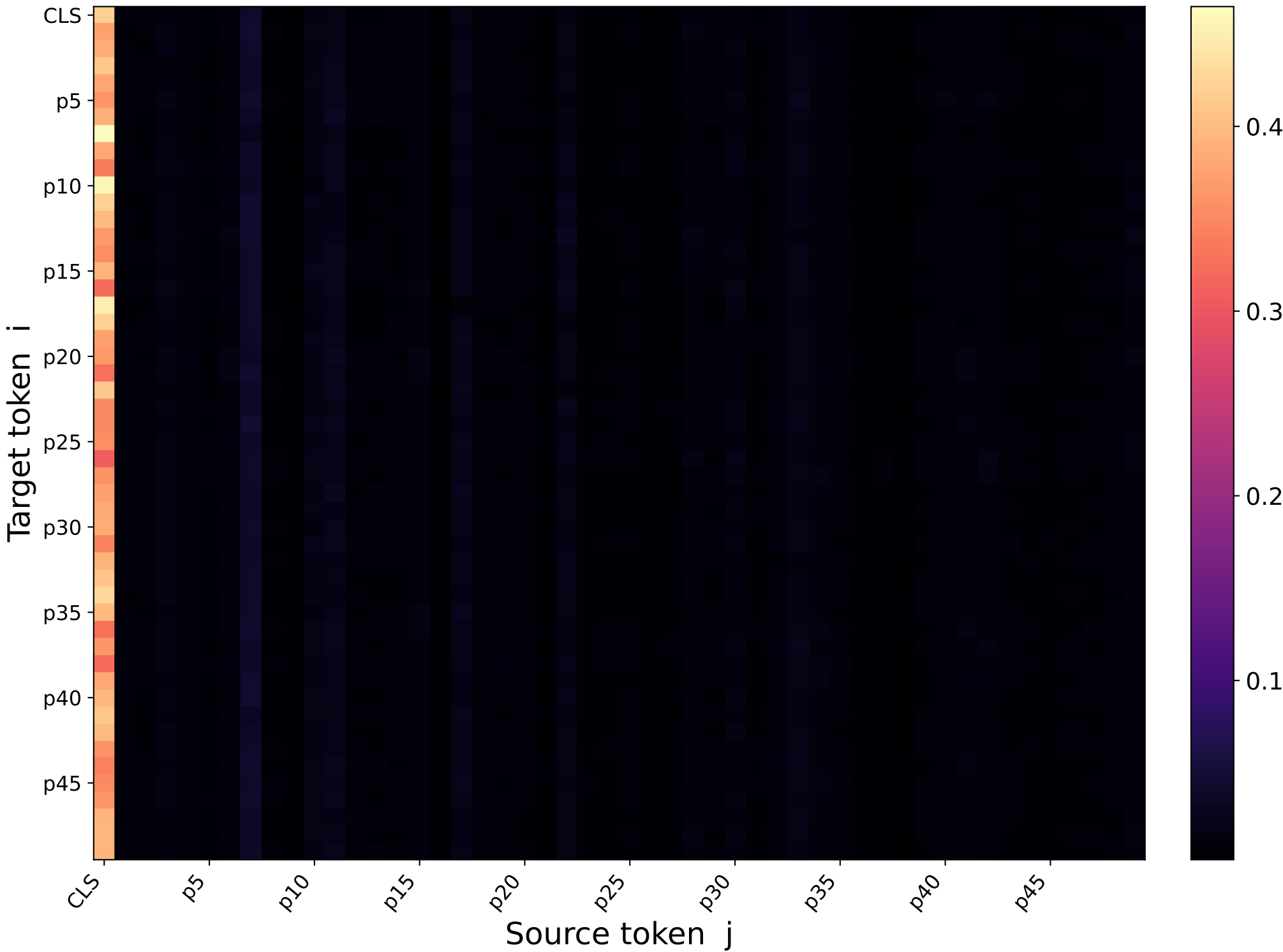
36422830_55c844bc2d [vanilla] — Layer 1, Head 1 attention matrix \mu = 0.02000 \sigma = 0.052054
