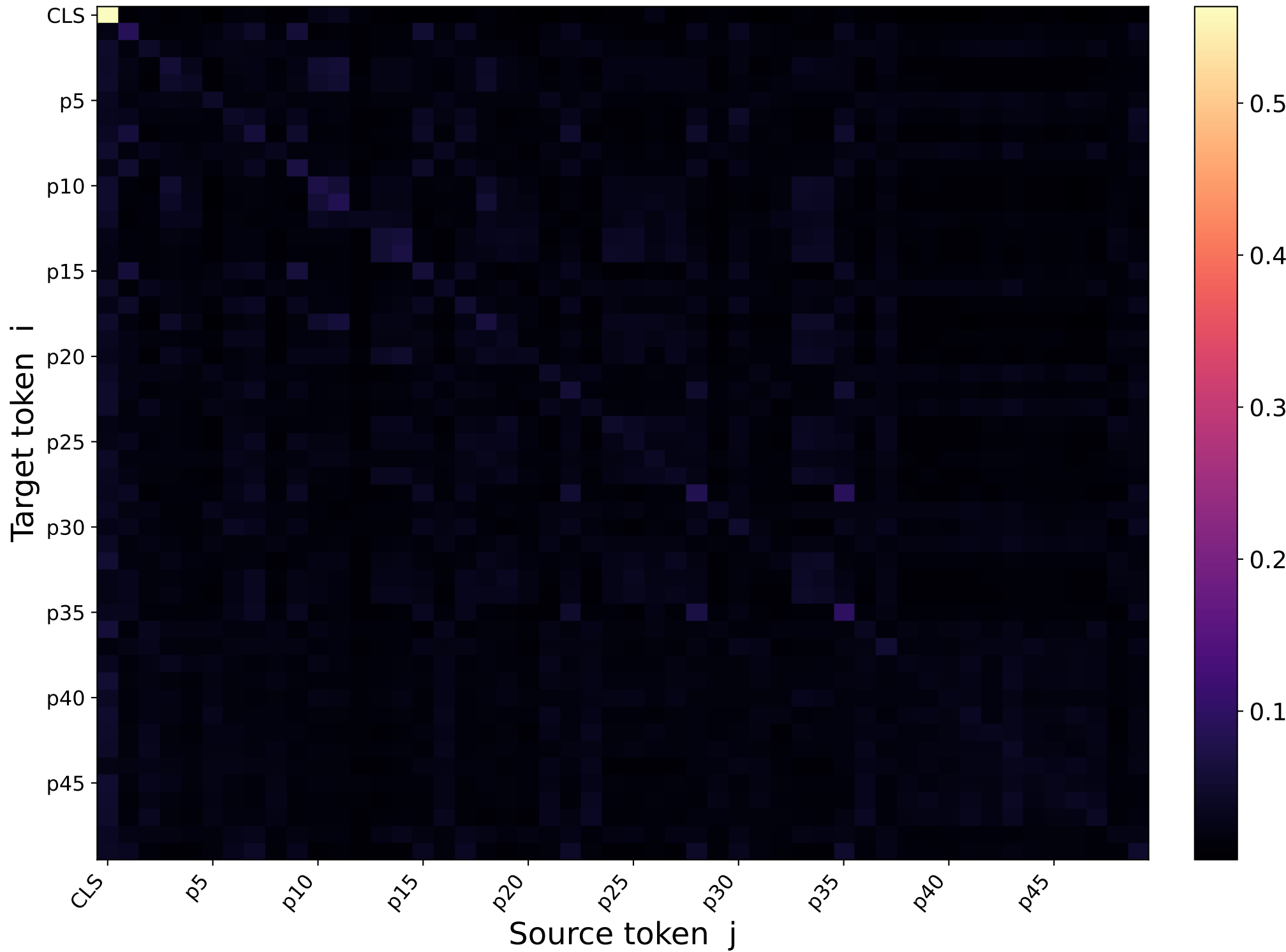
36422830_55c844bc2d [vanilla] — Last-layer mean attention matrix \mu = 0.02000 \sigma = 0.014843
