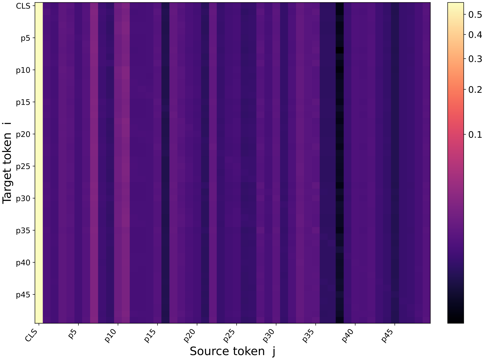
36422830_55c844bc2d Step 1 — Final per-head rollout (Head 1) \mu = 0.02000 \sigma = 0.077638
