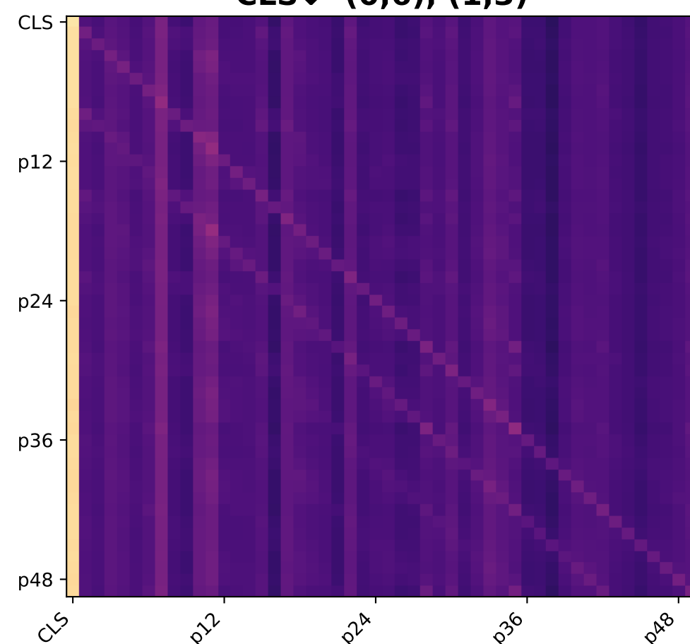
Layer 7 CLS↓ (0.6), (1.3)
