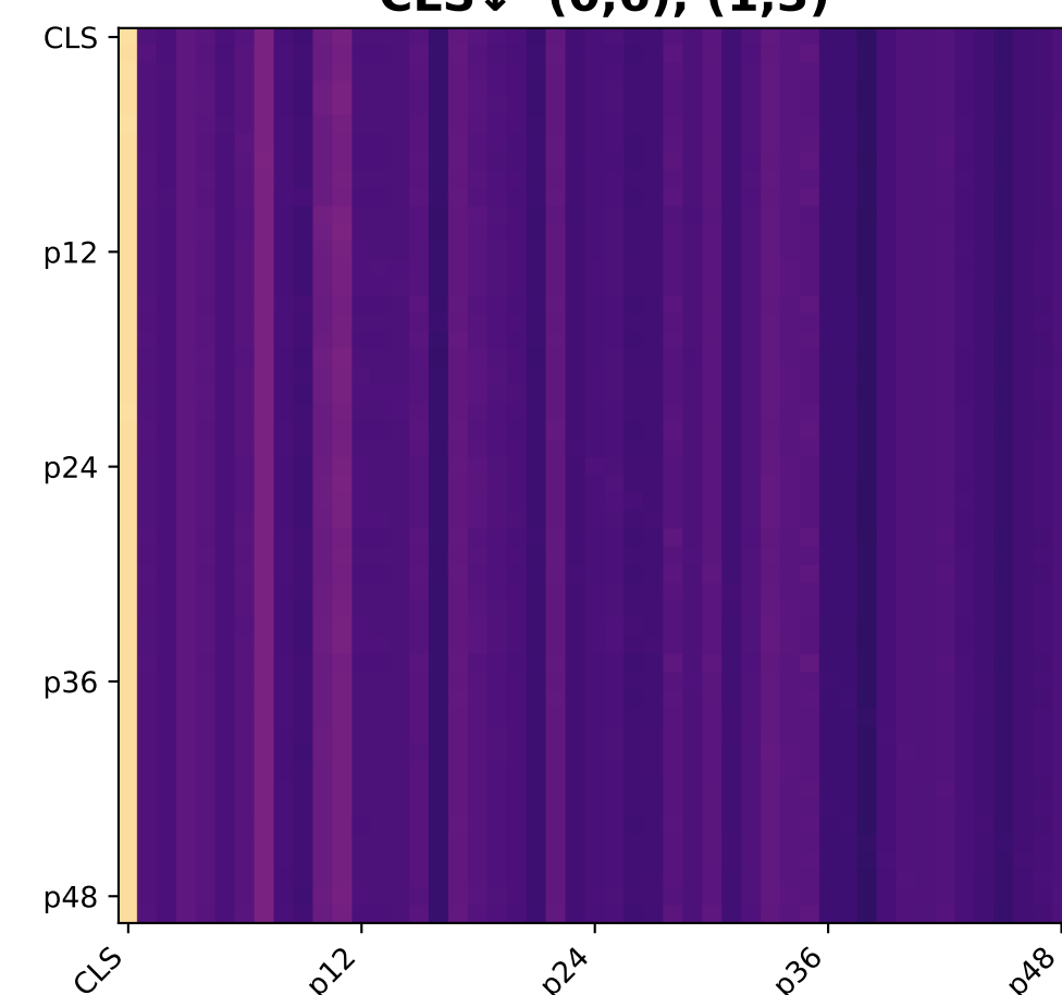
Layer 12 CISL (0.6) (1.3)
