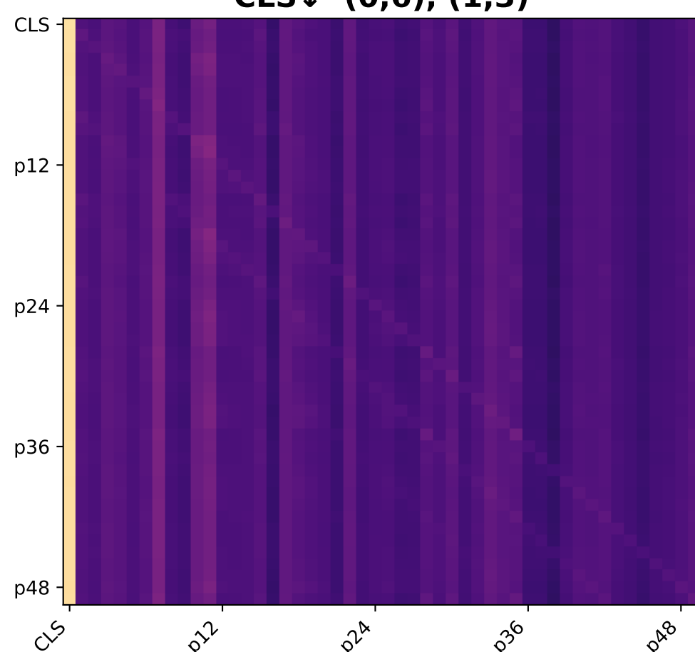
Layer 9 CLS, (0.6) (1.3)
