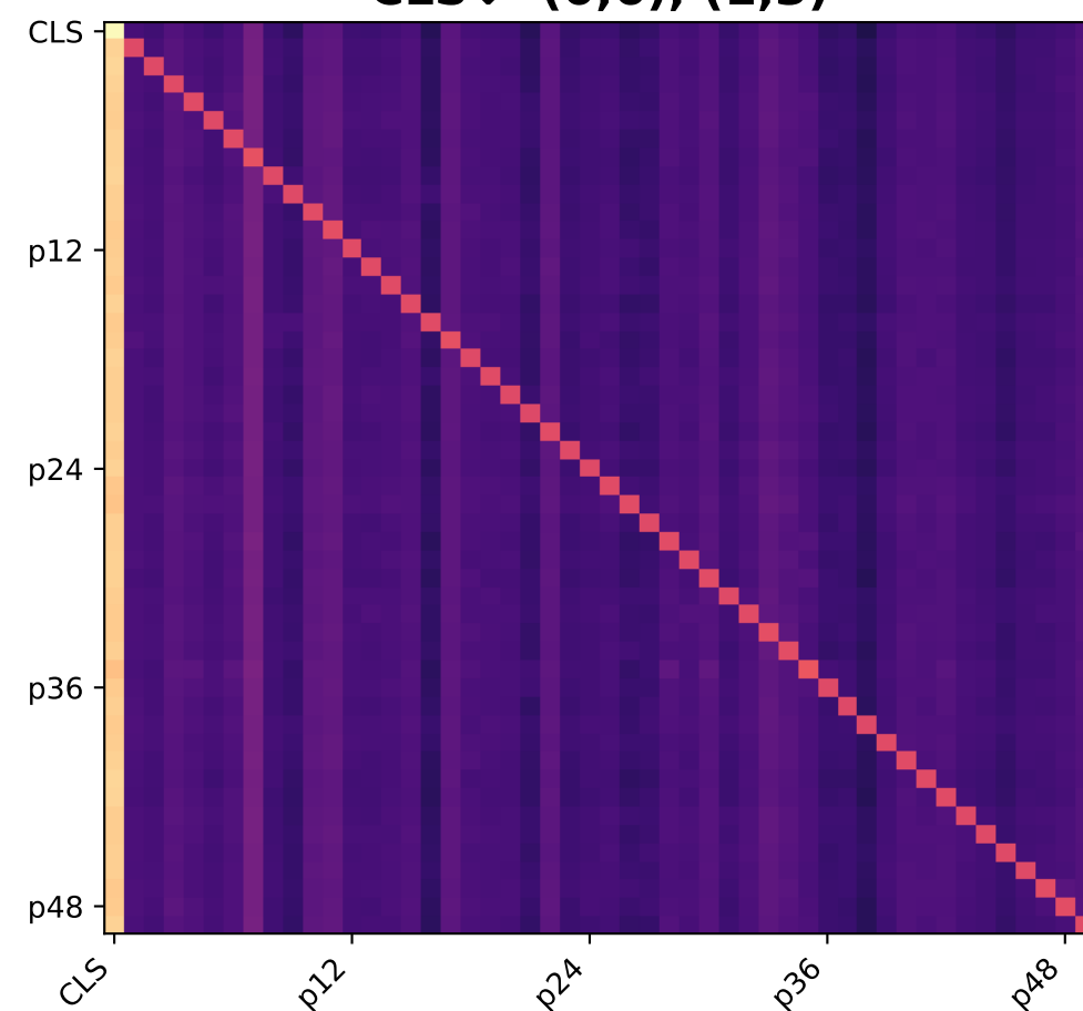
Layer 3 CLS↓ (0.6), (1.3)
