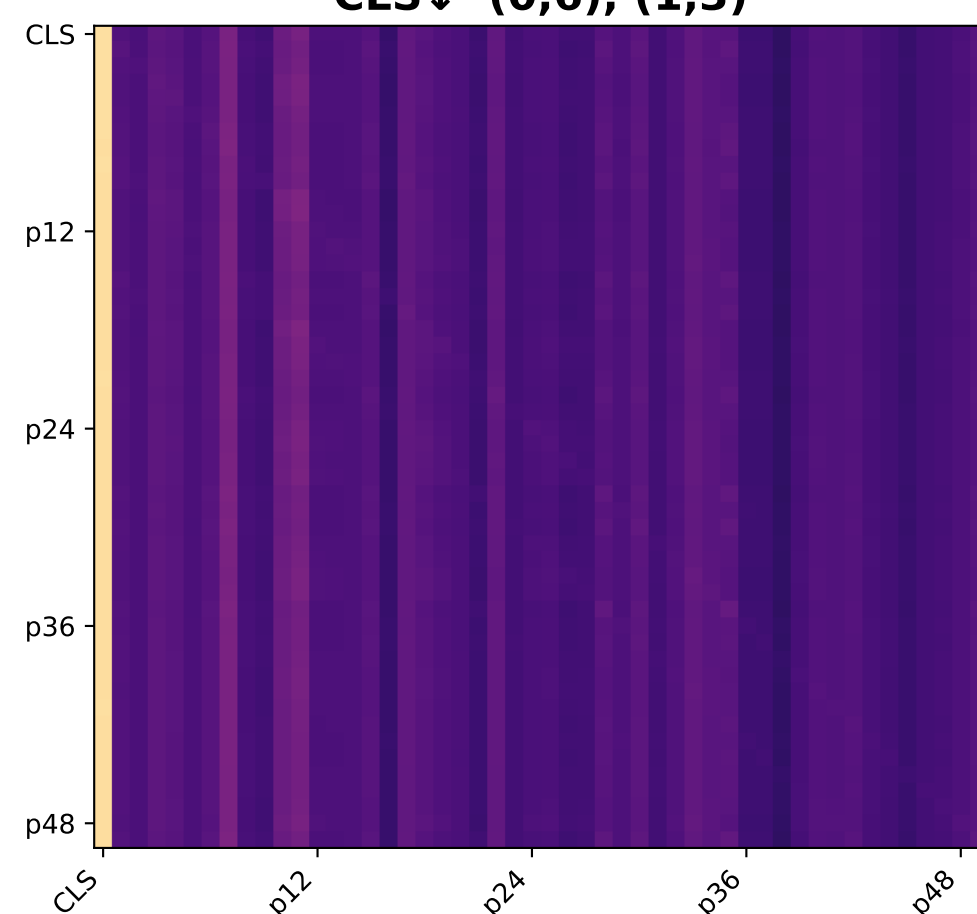
Layer 11 CLS: (0.6) (1.3)
