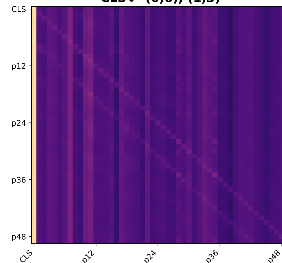
Layer 8 CLS↓ (0.6), (1.3)
