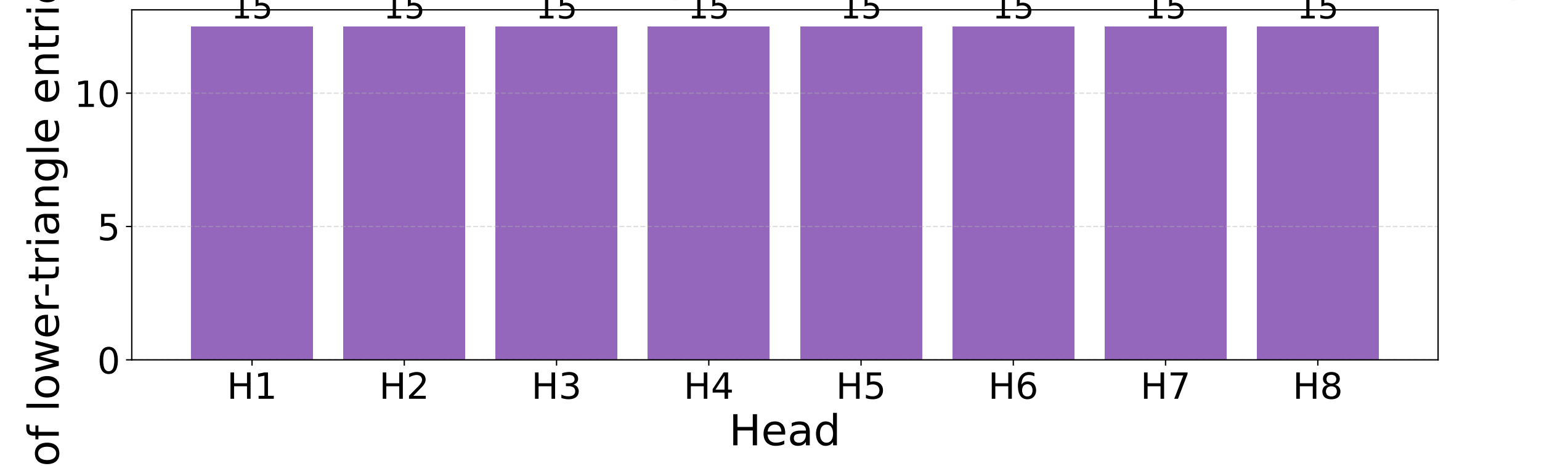
$\S 8$ Step 2 — Mask sparsity per head (K=0.3, lower-tri only)
