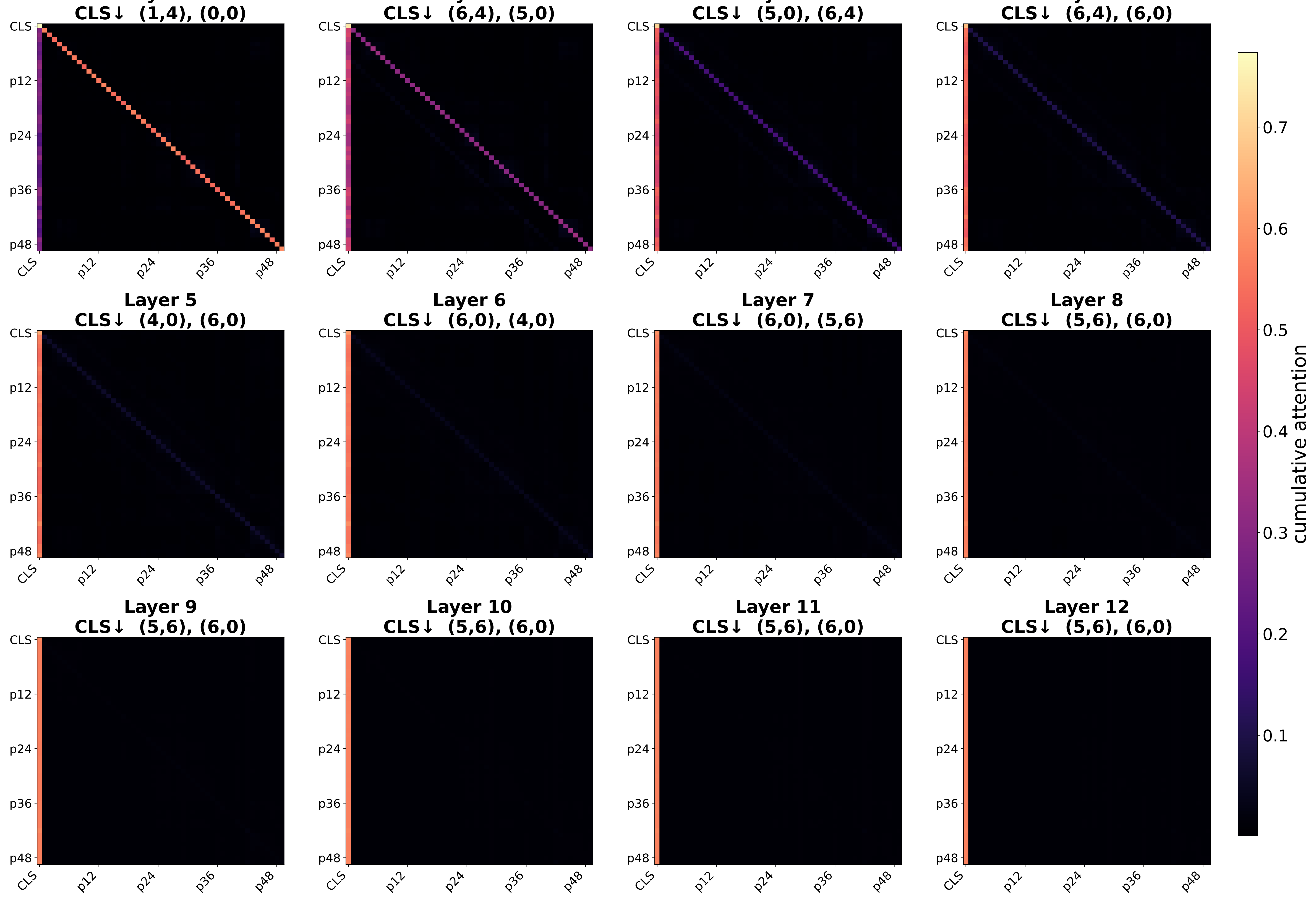
17273391_55cfc7d3d4 — heads-averaged Cumulative attention rollout matrix per layer (50×50: 1 CLS + 7×7 patches)
