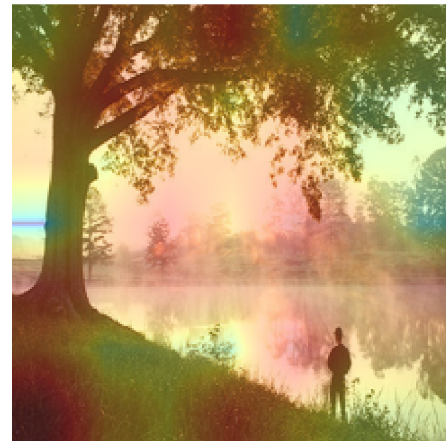
Head 12
