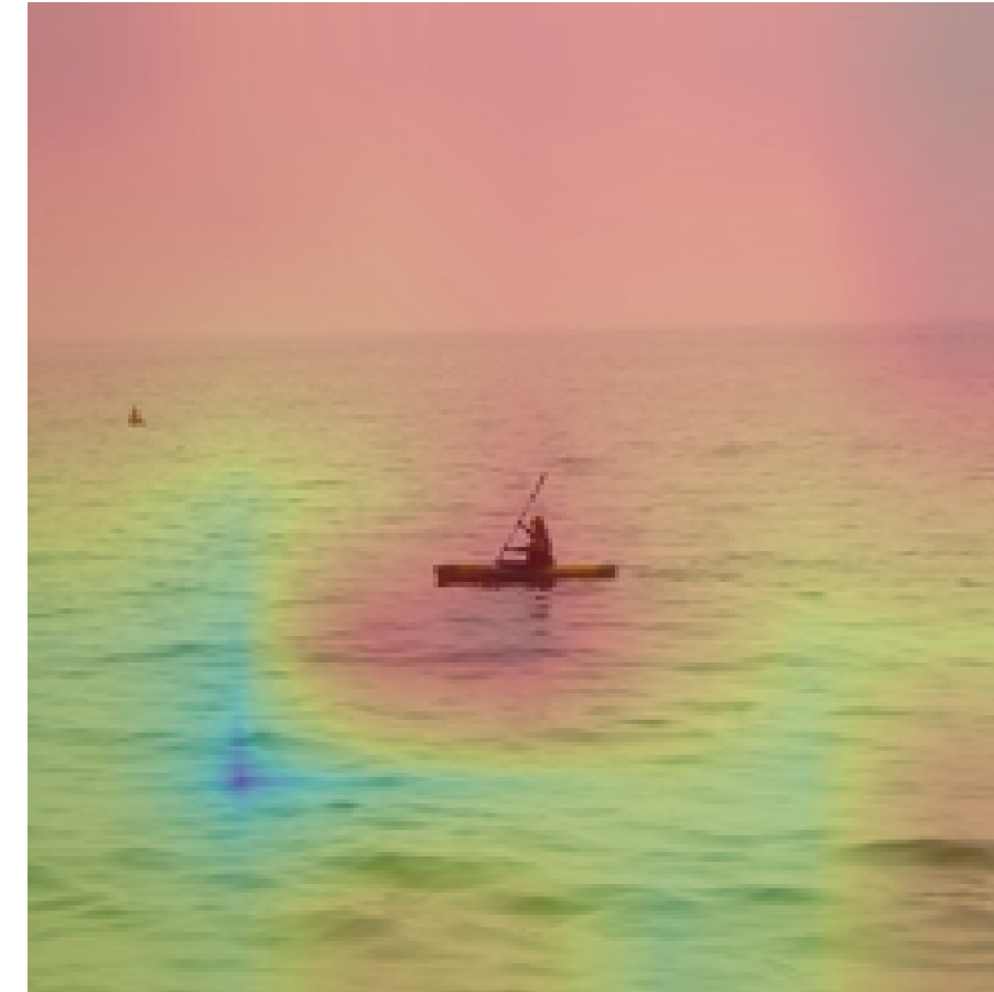
Head 11
