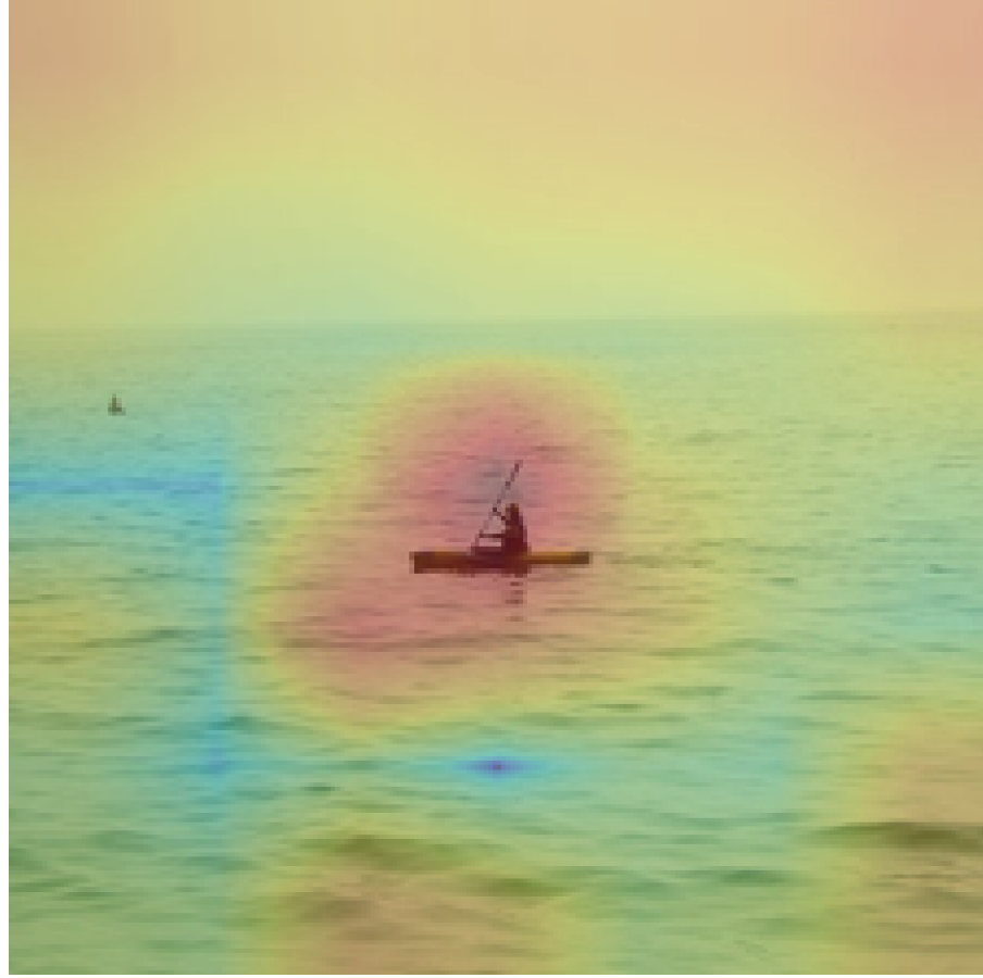
Head 5
