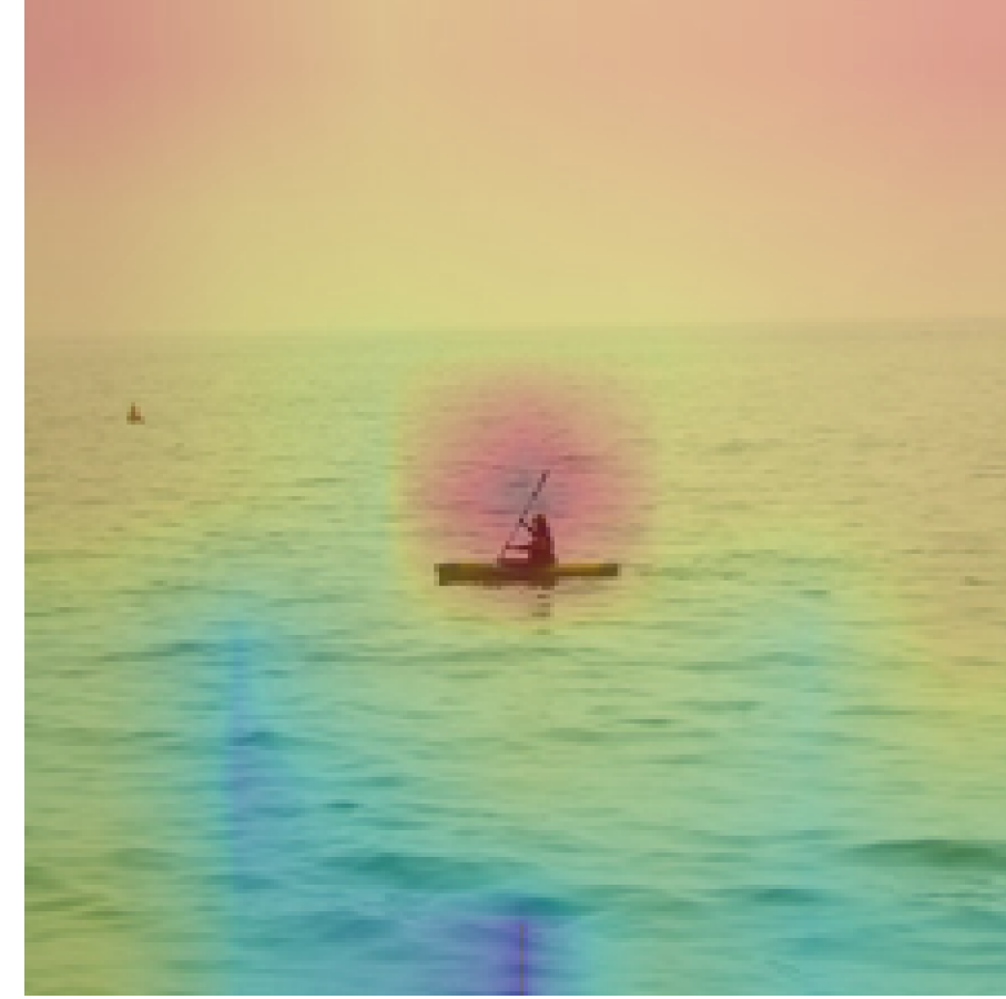
Head 6
