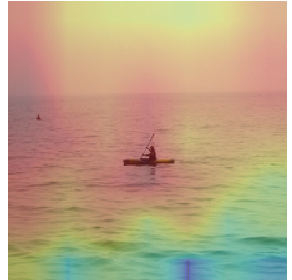
Head 12
