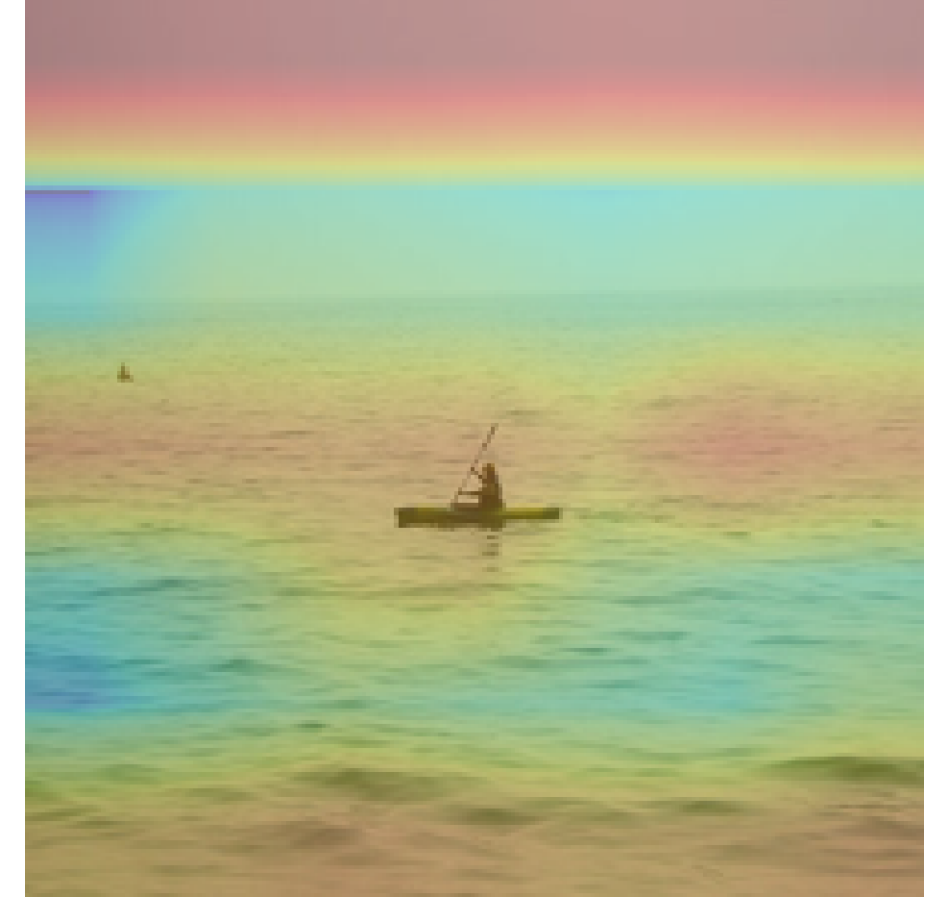
Head 8
