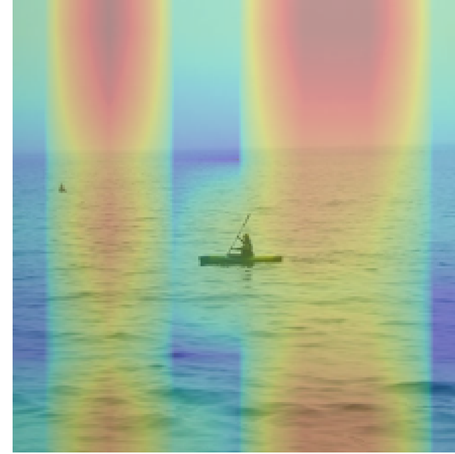
Head 7
