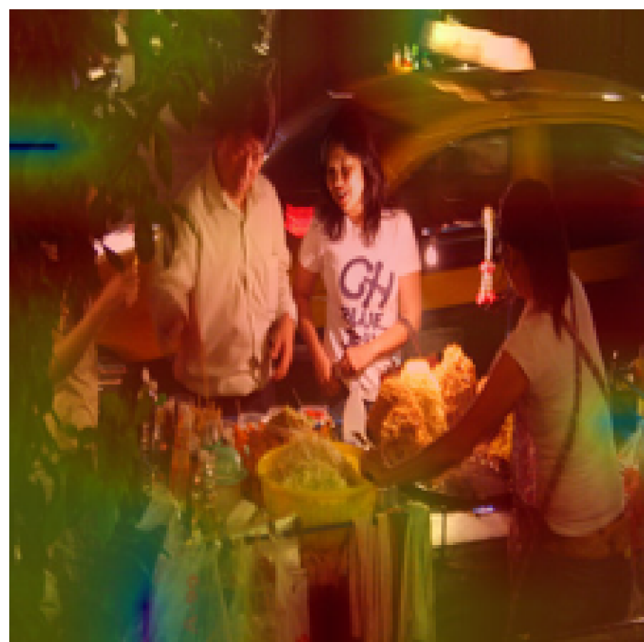
Head 9
