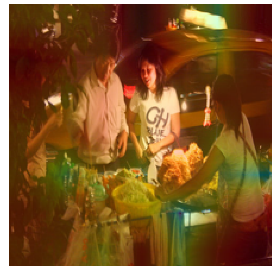
Head 12
