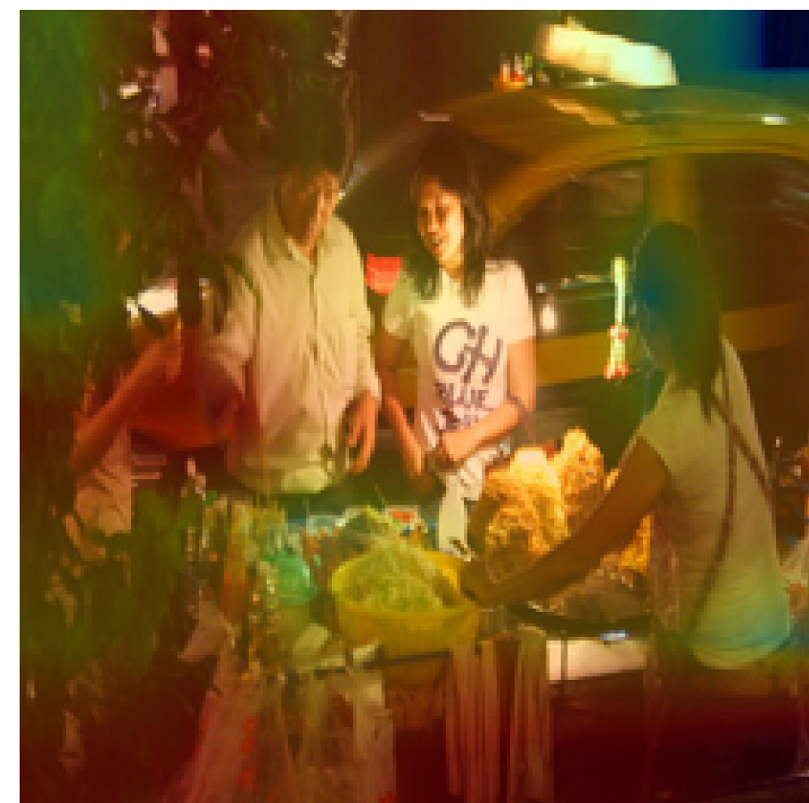
Head 10
