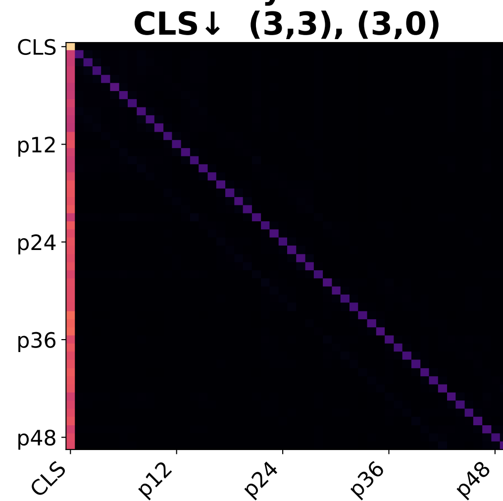
35506150_cbdh630f4f — heads-averaged \overline{\text{Layer}_2} Cumulative attention rollout matrix per layer (50×50: 1 CLS + 7×7 patches)
