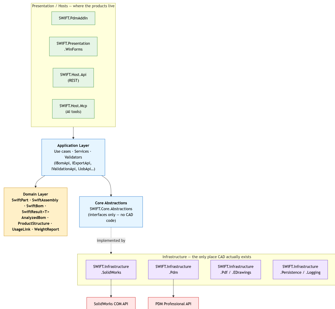
Figure 4: Inside the engine: a Clean Architecture in which the domain vocabulary ( SwiftPart , SwiftAssembly , SwiftBom , SwiftResult<T> ) is the single source of truth. Hosts at the top (PDM Add-in, WinForms, REST API, MCP server) all consume the same application services, and the only place that touches the raw SolidWorks and PDM APIs is the Infrastructure layer at the bottom. Replacing a CAD vendor means writing one new adapter — never touching the domain or any product above it.
