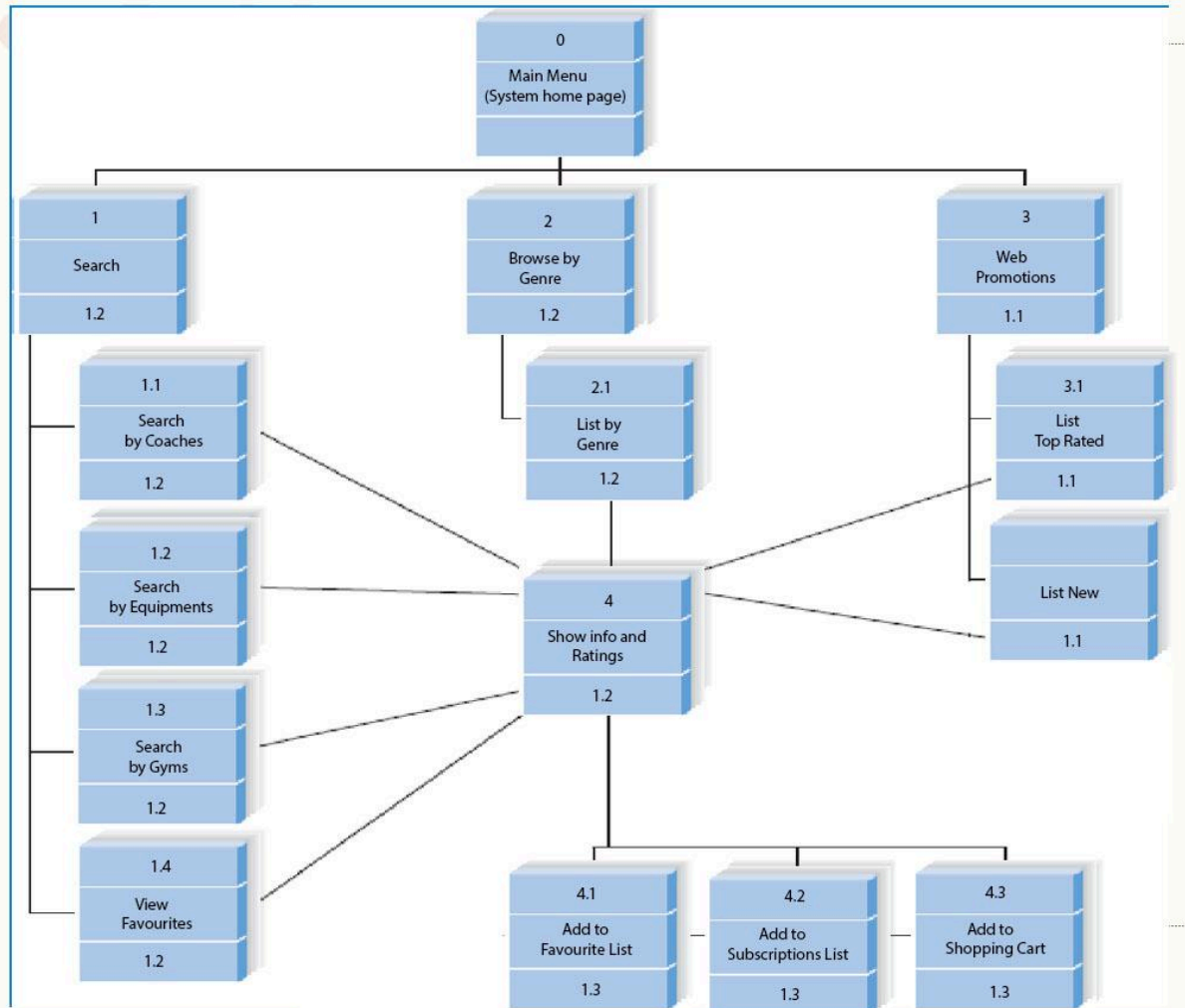
System For Exercises Interface structure diagram (ISD)
