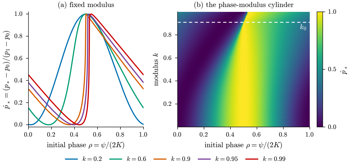
Figure 4: The normalized first conjugate root \hat{p}_* = (p_* - p_0)/(p_1 - p_0) against the phase \psi/(2K) . (a) Five fixed-modulus profiles, k = 0.2, 0.6, 0.9, 0.95, 0.99 . (b) The phase-modulus cylinder, \psi/(2K) horizontal, k vertical, colored by \hat{p}_* ; the dashed line is the critical modulus k_0 . The color scale is normalized separately at each modulus by the exact endpoints.
