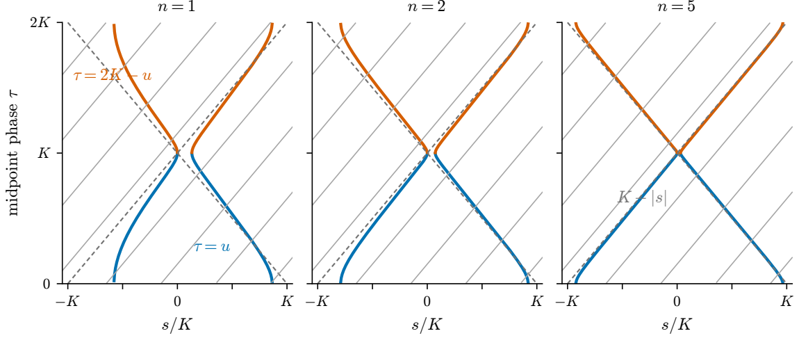
Figure 3: The zero curve of cells n = 1, 2, 5 at k = 0.8 in the strip, against s = p - 2nK in units of K : the branch \tau = u (blue) and its mirror \tau = 2K - u (orange) on the two brackets of Theorem 4.1, the broken lines \tau = K \mp |s| of Theorem 5.1(ii) (dashed), and four geodesics, each wrapped modulo 2K , drawn as lines of slope one. Each line meets the curve once on each bracket; with n the curve straightens onto the broken line and the intersections move to s = \frac{1}{2}(K - \psi) \bmod K .
