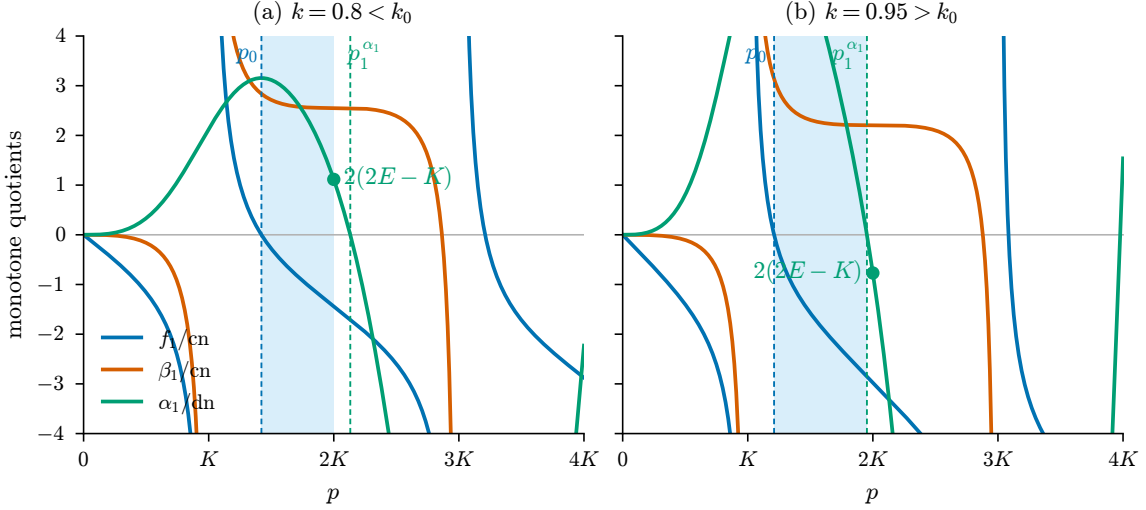
Figure 1: The three cell-wise monotone quotients of Lemma 3.1(ii) for k = 0.8 < k_0 (a) and k = 0.95 > k_0 (b), against p in units of K ; the poles at odd multiples of K are cut at \pm 4 . The shaded band is the bracket [p_0, p_1] . The dot is \alpha_1(2K) = 2(2E - K) : positive in (a), so p_1^{\alpha_1} > 2K and p_1 = 2K ; negative in (b), so p_1 = p_1^{\alpha_1} < 2K .
