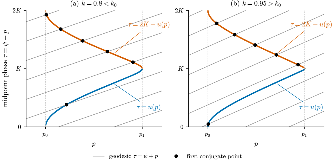
Figure 2: The one-cover in the (p, \tau) strip for k = 0.8 (a) and k = 0.95 (b). The zero set of J_2 is the curve \tau = u(p) , of slope at least one, and its mirror \tau = 2K - u(p) , of slope at most minus one, for p_0 \leq p \leq p_1 . Geodesics are the lines \tau = \psi + p of slope one, wrapped modulo 2K and drawn for six initial phases; each meets the curve exactly once, at the marked point.
