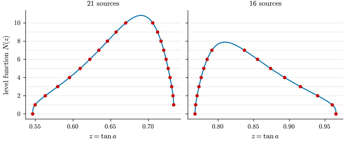
Figure 1: The level function N(z) of (7) for the target (39/5, -52/5, 3/10) , that is R = 13 and \theta = 3/10 , on its two admissible components, against z = \tan a . The horizontal lines are the integer levels and the dots the 37 integer crossings (21 and 16), one rotating source each, in agreement with (21). When a maximum crosses an integer level as the target varies, the corresponding sources merge in a fold (Proposition 2.2); a noninteger critical level alone does not represent a source of this target.
