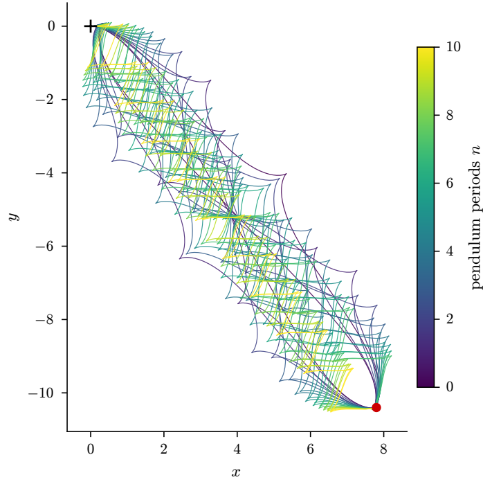
Figure 4: The 37 rotating geodesics from the identity (cross) to (39/5, -52/5, 3/10) (dot), coloured by the period index n of (4), the number of pendulum periods.
