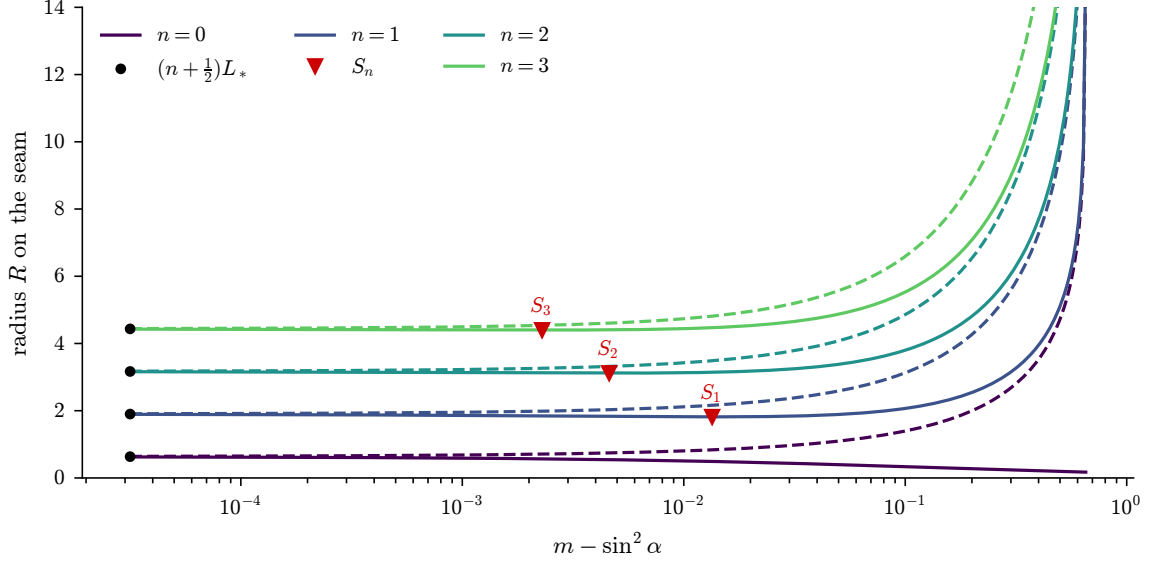
Figure 2: The seam branches R_n^{\text{short}} (solid) and R_n^{\text{long}} (dashed) of (26), n = 0, \dots, 3 , at \alpha = \pi/5 , against m - \sin^2 \alpha (logarithmic axis). For n \geq 1 , the short branch dips to its minimum S_n (triangles); the n = 0 short branch decreases. Both branches meet at H_n = (n + \frac{1}{2})L_* as m \rightarrow \sin^2 \alpha (dots).
