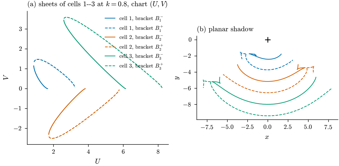
Figure 3: The sheets of the first three cells at k = 0.8 , both mirror branches: (a) in the half-angle chart, solid for B_n^- and dashed for B_n^+ ; (b) their planar shadow. Each bracket sheet is a fold surface; its S = 0 seam is a cusp edge for B_n^- and a fold for B_n^+ , and its C = 0 seam is the cusp edge at 2nK or the fold at p_n^\alpha (Theorem 9.1).
