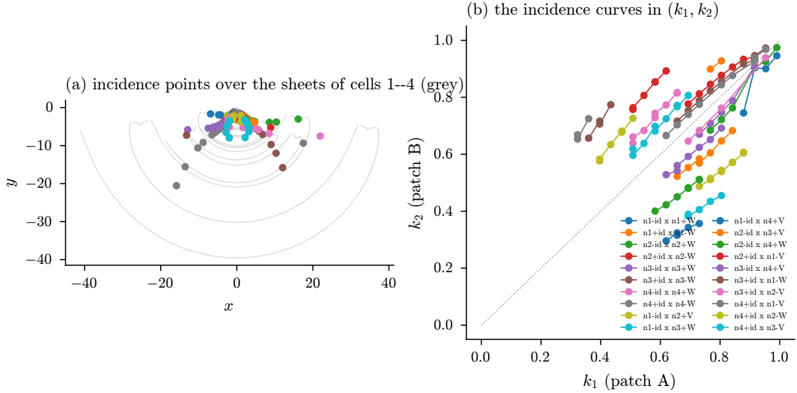
Figure 4: Incidences between the sheets of cells 1–4. (a) The accepted intersection points in the planar shadow, over the sheets in grey; (b) the same points in the (k_1, k_2) plane of the moduli of the two patches, in the order of the label ( patch A , patch B on the axes); each unordered pair appears twice, mirrored in the diagonal, and each color serves two pairs (see the legend). The sampled traces are monotone, and the trace with the left sheet first lies below the diagonal: the left sheet has the larger modulus at these points. Labels: n1-id \times n2+V is F(1, -) \cap gF(2, +) ; the token after each cell index and bracket sign names the element of G applied to that patch, id the identity (the fundamental patch itself), V the reflection V \mapsto -V and W the reflection W \mapsto -W .
