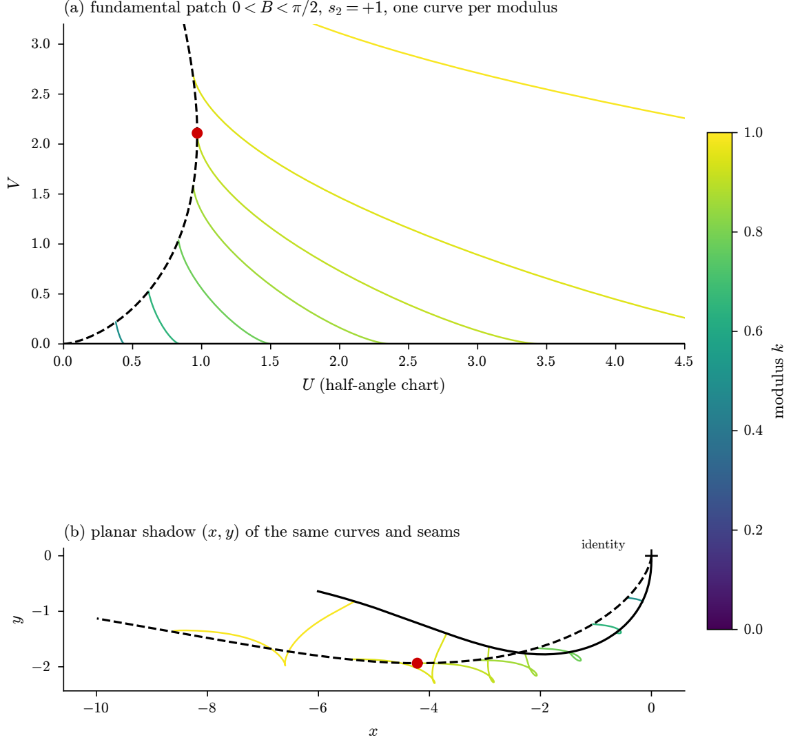
Figure 2: The first caustic. (a) The fundamental patch 0 < B < \pi/2 , s_2 = +1 , in the half-angle chart (U, V) for seven moduli (color), with the Maxwell seam B = 0 (solid, the cusp edge, V = 0 ) and the upper seam B = \pi/2 (dashed) across all moduli, and the D_4^+ point at k_0 . (b) The planar shadow (x, y) of the same curves and seams; each curve is the projection of the first conjugate points of the geodesics of one modulus.
