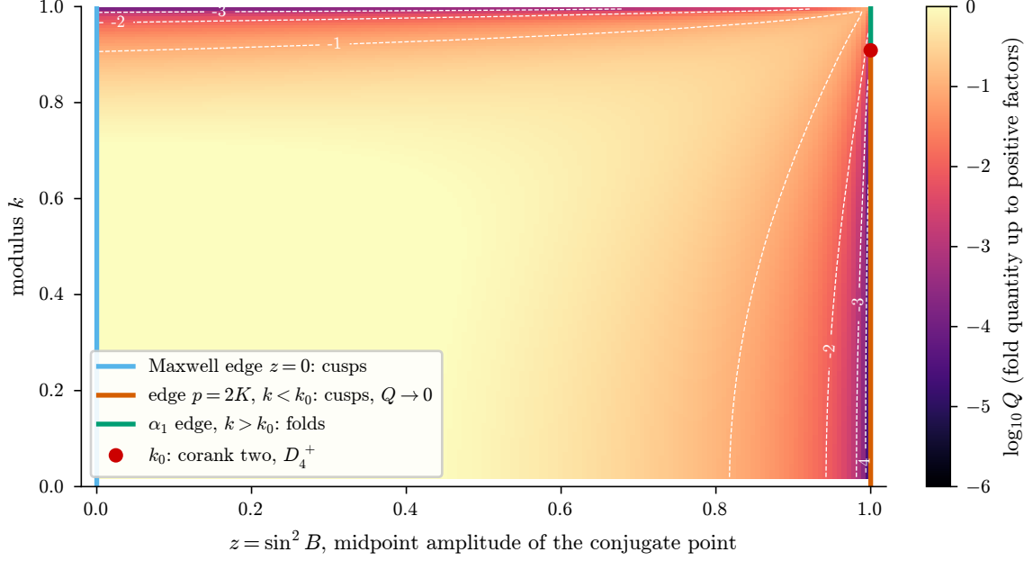
Figure 1: The fold quantity on the source rectangle of the first sheet, z = \sin^2 B = r against k : \log_{10} Q (color and white contour labels). Q is positive inside and tends to zero at the edge p = 2K for k \leq k_0 , where the kernel derivative of J_2 must vanish because that edge is a cusp edge, and along the separatrix k \rightarrow 1 . At the Maxwell edge z = 0 it is the factor S = \sqrt{z} in (14), not Q , that vanishes. The \alpha_1 edge above k_0 carries Q > 0 : it is a fold.
