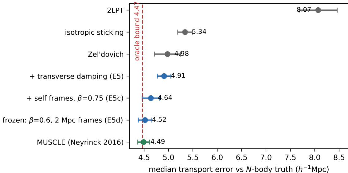
Model ladder (held-out seeds)
