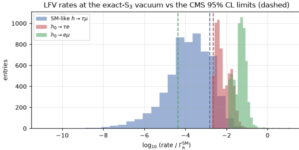
Figure 2: LFV branching ratios of the SM-like state over all points and \mu_3^\ell values, and of h_0 ’s e\tau , e\mu rate ratios, against the CMS 95% CL limits (dashed). The SM-like h \rightarrow \tau\mu straddles its limit.
