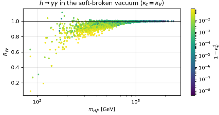
Figure 3: R_{\gamma\gamma} against the lighter charged-Higgs mass, coloured by the non-vacuum admixture.
