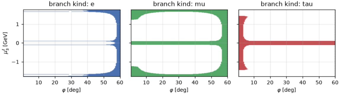
Figure 1: Where a lepton fit exists, by branch kind (which lepton the e_+ entry A grows into; “e” is the draft’s branch). At \varphi = 60^\circ the whole \mu_3 axis is allowed. Away from it the draft-type branch survives on about 5% of the axis, near \pm m_\tau .
