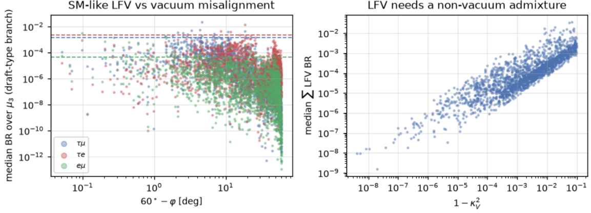
Figure 2: Left: SM-like LFV rates (median over \mu_3 , draft-type branch) against the vacuum misalignment, with the CMS limits dashed. Right: the total LFV rate against the non-vacuum admixture 1 - \kappa_V^2 ; the correlation is 0.88 in log.
