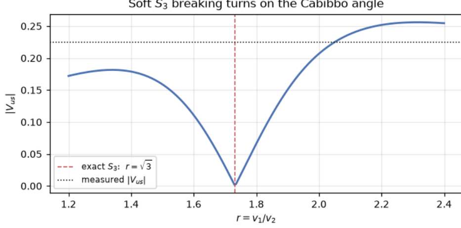
Figure 1: |V_{us}| against the vacuum ratio r at fixed Yukawas. It vanishes exactly at the exact- S_3 vacuum ( |V_{us}| = 4.6 \times 10^{-17} at r = \sqrt{3} ) and grows linearly away from it: the ratio of its values at r = \sqrt{3} + 0.05 and \sqrt{3} + 0.025 is 1.999.
