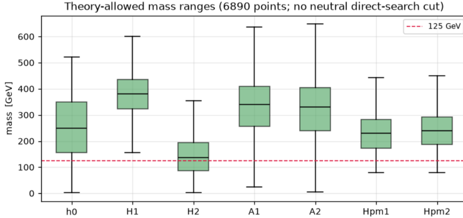
Figure 3: Theory-allowed mass ranges for the seven physical scalars over the 6890 points that pass boundedness, unitarity, no tachyons and m_{H^\pm} > 80 GeV, before the 125 GeV and neutral-state cuts below.
