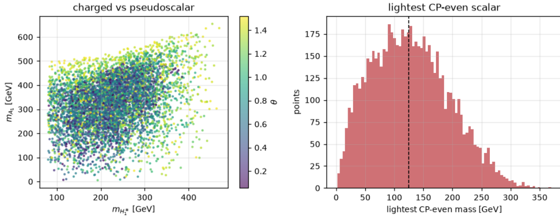
Figure 4: Correlations across the theory-allowed region (the 6890 points of Fig. 3).
