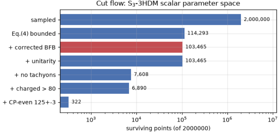
Figure 2: Cut flow over the 2 \times 10^6 -point scan, up to the theory cuts and a mass-only 125 GeV condition. The coupling-based rows that replace the last bar are in the table above.
