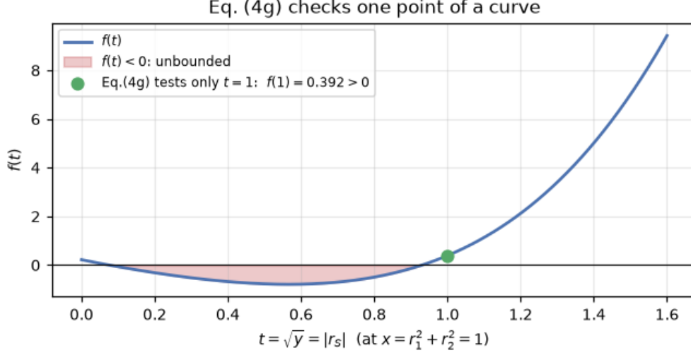
Figure 1: The quartic (3) at the counterexample point (4). Eq. (4g) tests only t = 1 , where f(1) = 0.392 > 0 and the condition passes; the curve dips to -0.789 at t = 0.565 , so the potential is unbounded below along a real neutral direction.
