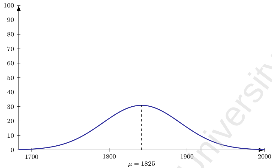
Figure 139: Flight 6E 083 (DEL-DMM), dep 2055. Model M1 entry-time distribution: Normal, mean 150 min before departure ( \mu = 1825 ), SD 30 min; area = 232 pax (LF = 1).
