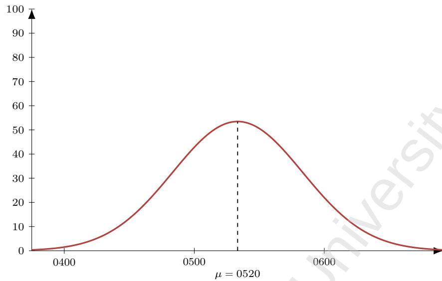
Figure 61: Flight SU 233 (DEL-SVO), dep 0750. Model M1 entry-time distribution: Normal, mean 150 min before departure ( \mu = 0520 ), SD 30 min; area = 402 pax (LF = 1).
