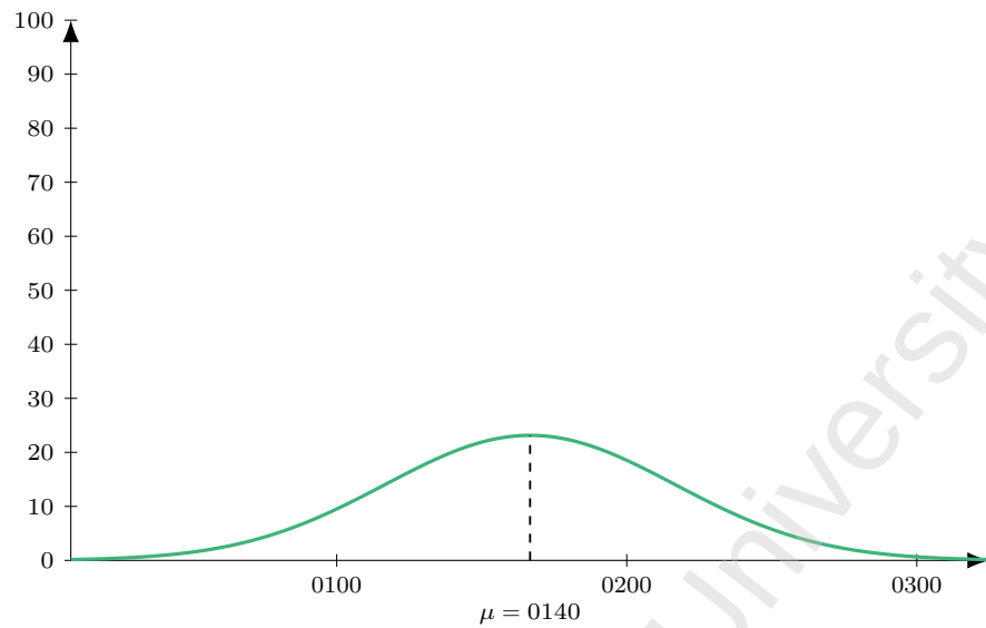
Figure 34: Flight FZ 442 (DEL-DXB), dep 0410. Model M1 entry-time distribution: Normal, mean 150 min before departure ( \mu = 0140 ), SD 30 min; area = 174 pax (LF = 1).
