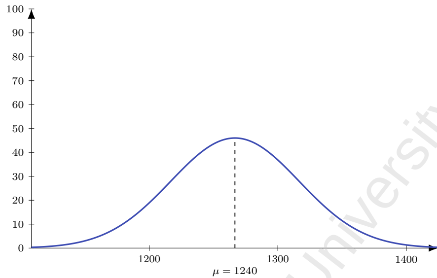
Figure 111: Flight RQ 4402 (DEL-KBL), dep 1510. Model M1 entry-time distribution: Normal, mean 150 min before departure ( \mu = 1240 ), SD 30 min; area = 346 pax (LF = 1).
