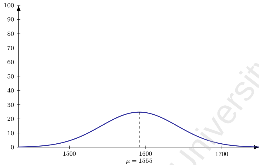
Figure 126: Flight 6E 1169 (DEL-CMB), dep 1825. Model M1 entry-time distribution: Normal, mean 150 min before departure ( \mu = 1555 ), SD 30 min; area = 186 pax (LF = 1).
