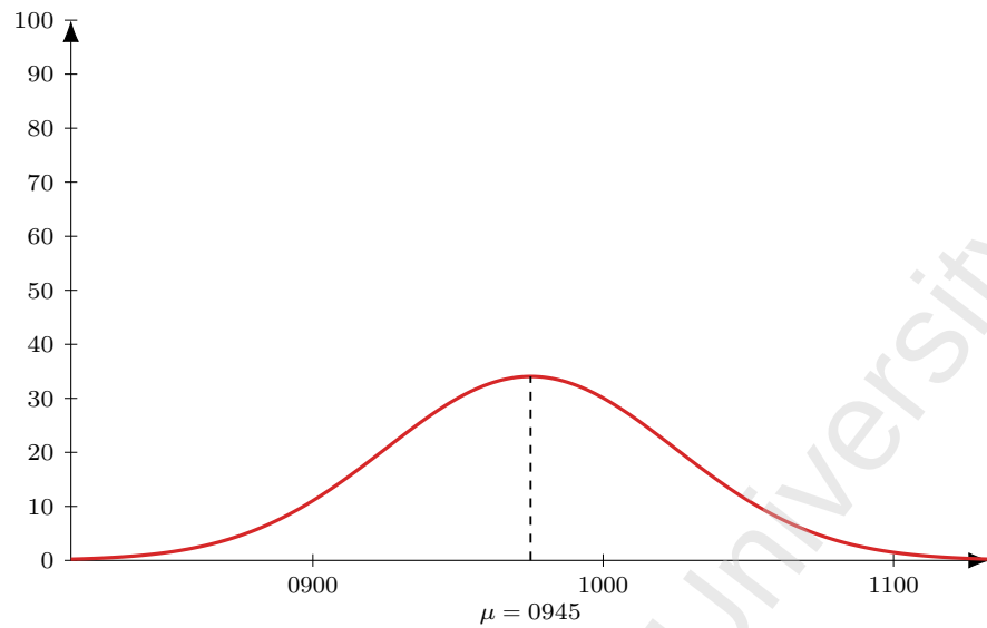
Figure 95: Flight AI 157 (DEL-CPH), dep 1215. Model M1 entry-time distribution: Normal, mean 150 min before departure ( \mu = 0945 ), SD 30 min; area = 256 pax (LF = 1).
