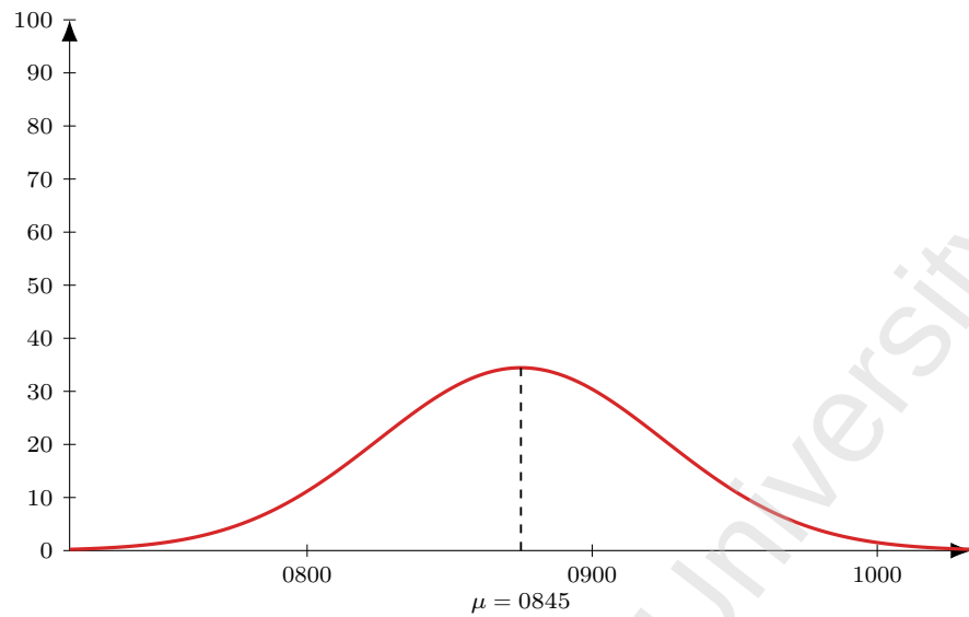
Figure 87: Flight AI 155 (DEL-AMS), dep 1115. Model M1 entry-time distribution: Normal, mean 150 min before departure ( \mu = 0845 ), SD 30 min; area = 259 pax (LF = 1).
