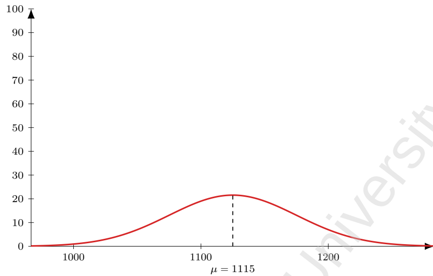
Figure 105: Flight AI 2243 (DEL-RUH), dep 1345. Model M1 entry-time distribution: Normal, mean 150 min before departure ( \mu = 1115 ), SD 30 min; area = 162 pax (LF = 1).
