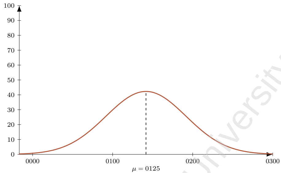
Figure 33: Flight KL 872 (DEL-AMS), dep 0355. Model M1 entry-time distribution: Normal, mean 150 min before departure ( \mu = 0125 ), SD 30 min; area = 318 pax (LF = 1).
