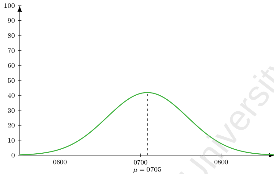
Figure 72: Flight ET 689 (DEL-ADD), dep 0935. Model M1 entry-time distribution: Normal, mean 150 min before departure ( \mu = 0705 ), SD 30 min; area = 315 pax (LF = 1).
