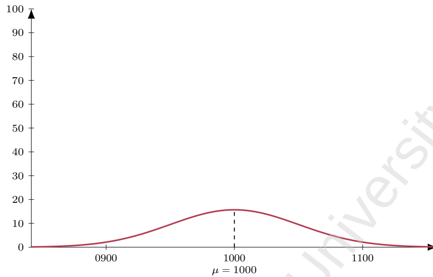
Figure 98: Flight KB 201 (DEL-PBH), dep 1230. Model M1 entry-time distribution: Normal, mean 150 min before departure ( \mu = 1000 ), SD 30 min; area = 118 pax (LF = 1).
