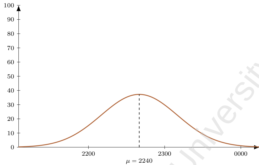
Figure 12: Flight CX 694 (DEL-HKG), dep 0110. Model M1 entry-time distribution: Normal, mean 150 min before departure ( \mu = 2240 ), SD 30 min; area = 280 pax (LF = 1).
