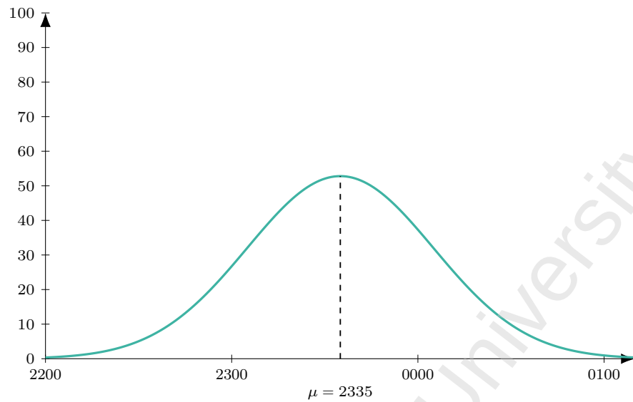
Figure 21: Flight VS 303 (DEL-LHR), dep 0205. Model M1 entry-time distribution: Normal, mean 150 min before departure ( \mu = 2335 ), SD 30 min; area = 397 pax (LF = 1).
