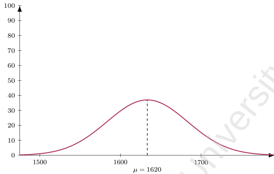
Figure 131: Flight KE 498 (DEL-ICN), dep 1850. Model M1 entry-time distribution: Normal, mean 150 min before departure ( \mu = 1620 ), SD 30 min; area = 278 pax (LF = 1).
