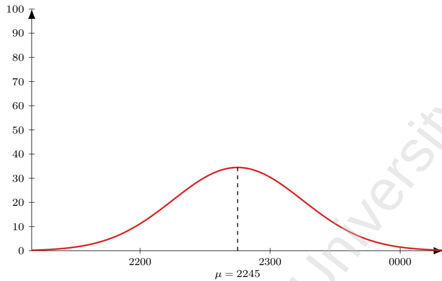
Figure 14: Flight AI 308 (DEL-MEL), dep 0115. Model M1 entry-time distribution: Normal, mean 150 min before departure ( \mu = 2245 ), SD 30 min; area = 259 pax (LF = 1).
