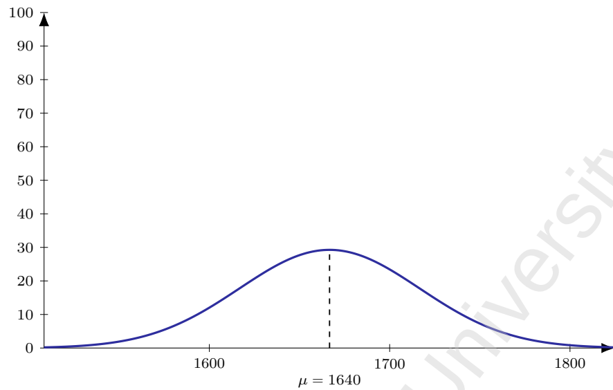
Figure 133: Flight 6E 1463 (DEL-DXB), dep 1910. Model M1 entry-time distribution: Normal, mean 150 min before departure ( \mu = 1640 ), SD 30 min; area = 220 pax (LF = 1).
