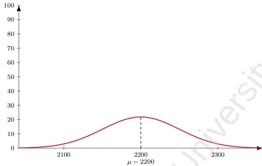
Figure 6: Flight AI 2336 (DEL-BKK), dep 0030. Model M1 entry-time distribution: Normal, mean 150 min before departure ( \mu = 2200 ), SD 30 min; area = 164 pax (LF = 1).
