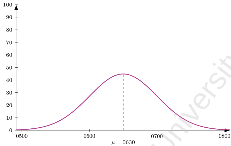
Figure 68: Flight SQ 401 (DEL-SIN), dep 0900. Model M1 entry-time distribution: Normal, mean 150 min before departure ( \mu = 0630 ), SD 30 min; area = 337 pax (LF = 1).
