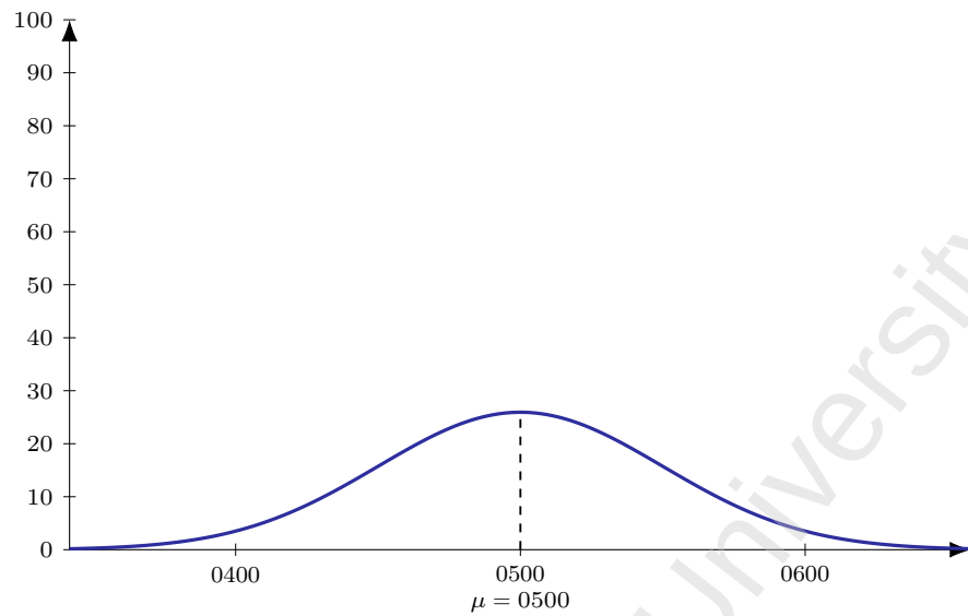
Figure 56: Flight 6E 1901 (DEL-ATH), dep 0730. Model M1 entry-time distribution: Normal, mean 150 min before departure ( \mu = 0500 ), SD 30 min; area = 195 pax (LF = 1).
