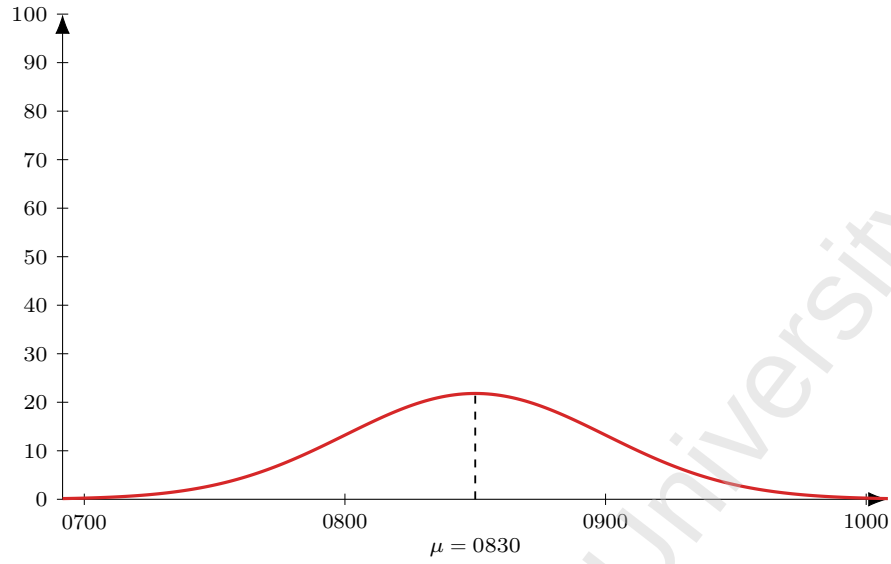
Figure 82: Flight AI 2332 (DEL-BKK), dep 1100. Model M1 entry-time distribution: Normal, mean 150 min before departure ( \mu = 0830 ), SD 30 min; area = 164 pax (LF = 1).
