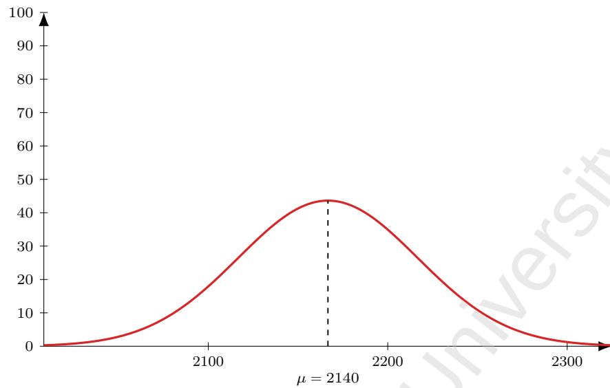
Figure 4: Flight AI 187 (DEL-VIE-YYZ), dep 0010. Model M1 entry-time distribution: Normal, mean 150 min before departure ( \mu = 2140 ), SD 30 min; area = 328 pax (LF = 1).
