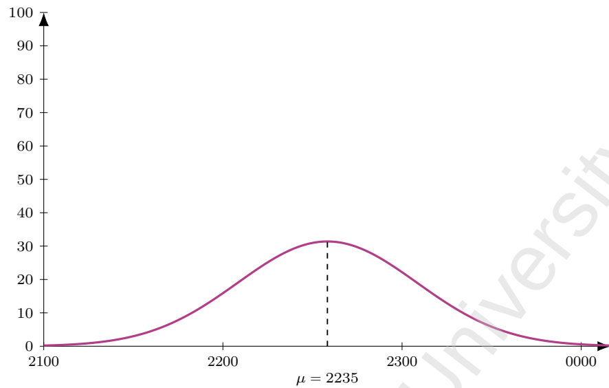
Figure 11: Flight LX 147 (DEL-ZRH), dep 0105. Model M1 entry-time distribution: Normal, mean 150 min before departure ( \mu = 2235 ), SD 30 min; area = 236 pax (LF = 1).
