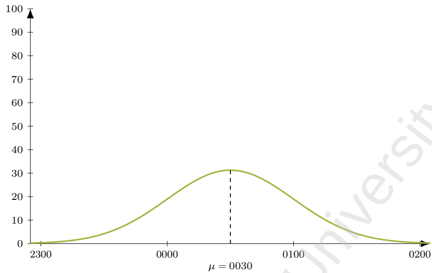
Figure 27: Flight KU 382 (DEL-KWI), dep 0300. Model M1 entry-time distribution: Normal, mean 150 min before departure ( \mu = 0030 ), SD 30 min; area = 235 pax (LF = 1).
