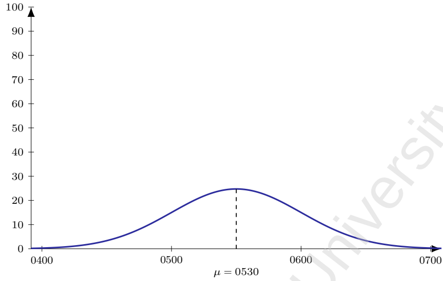
Figure 62: Flight 6E 1151 (DEL-KTM), dep 0800. Model M1 entry-time distribution: Normal, mean 150 min before departure ( \mu = 0530 ), SD 30 min; area = 186 pax (LF = 1).
