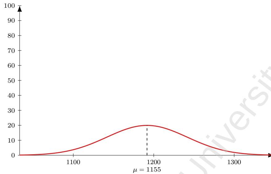
Figure 107: Flight AI 219 (DEL-KTM), dep 1425. Model M1 entry-time distribution: Normal, mean 150 min before departure ( \mu = 1155 ), SD 30 min; area = 150 pax (LF = 1).
