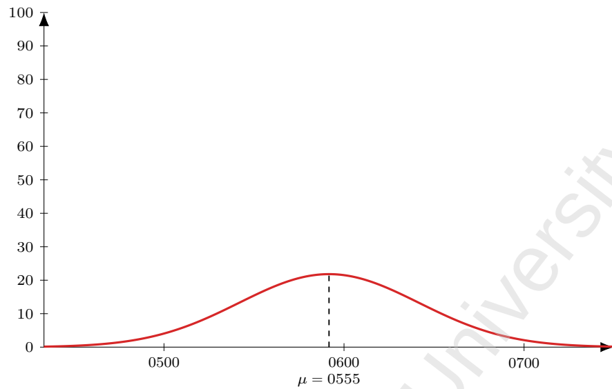
Figure 64: Flight AI 2355 (DEL-BKK), dep 0825. Model M1 entry-time distribution: Normal, mean 150 min before departure ( \mu = 0555 ), SD 30 min; area = 164 pax (LF = 1).
