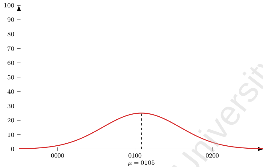
Figure 31: Flight AI 2115 (DEL-SIN), dep 0335. Model M1 entry-time distribution: Normal, mean 150 min before departure ( \mu = 0105 ), SD 30 min; area = 188 pax (LF = 1).
