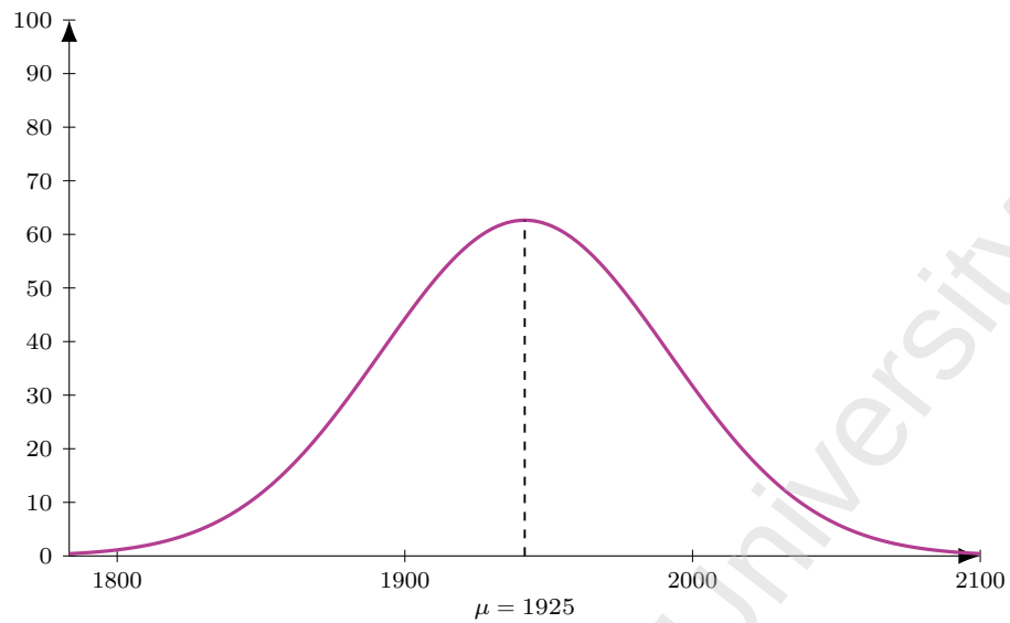
Figure 149: Flight SQ 403 (DEL-SIN), dep 2155. Model M1 entry-time distribution: Normal, mean 150 min before departure ( \mu = 1925 ), SD 30 min; area = 471 pax (LF = 1).
