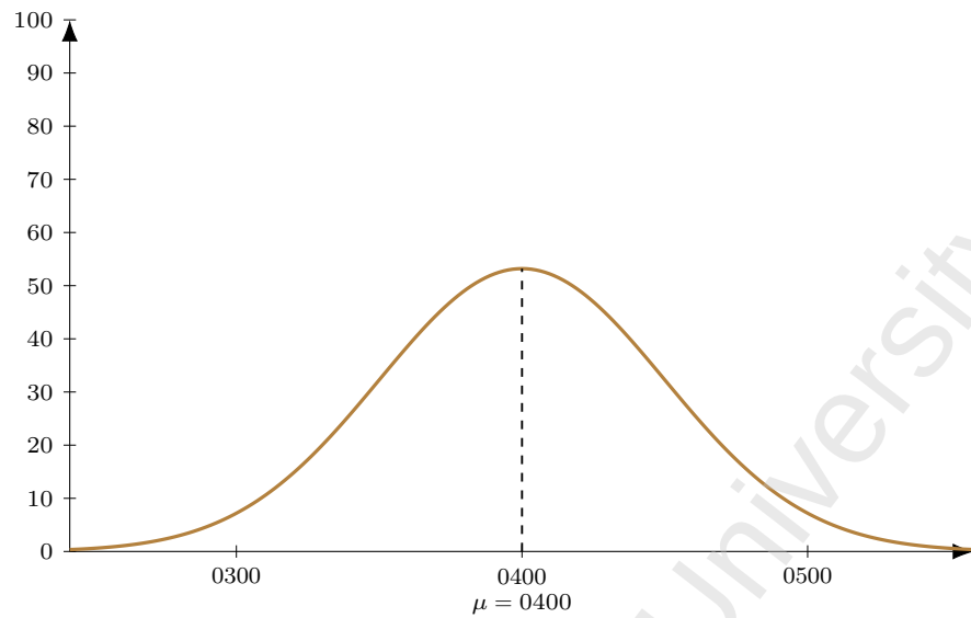
Figure 51: Flight TK 717 (DEL-IST), dep 0630. Model M1 entry-time distribution: Normal, mean 150 min before departure ( \mu = 0400 ), SD 30 min; area = 400 pax (LF = 1).
