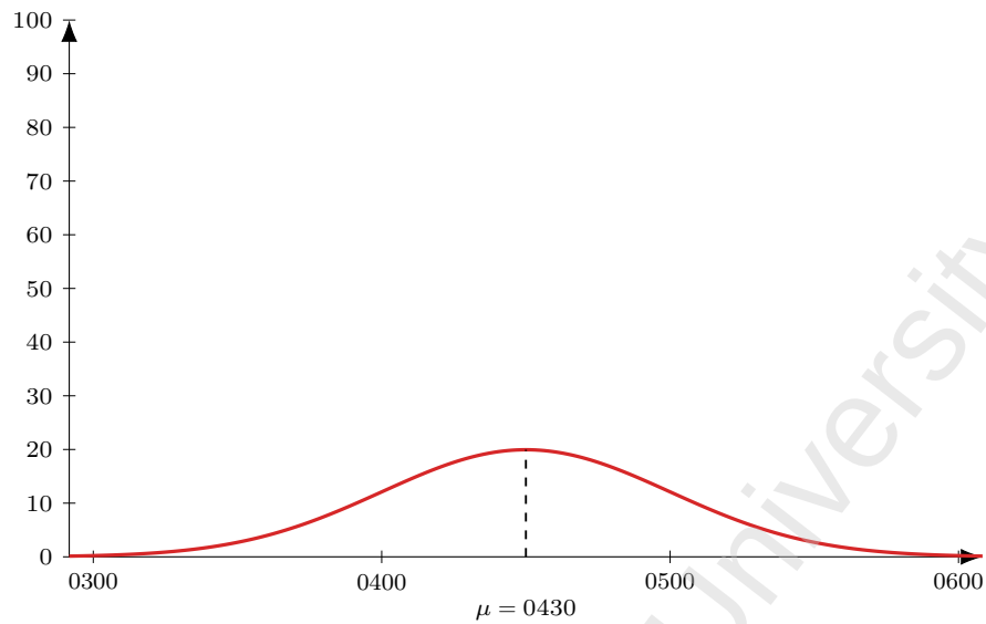
Figure 55: Flight AI 213 (DEL-KTM), dep 0700. Model M1 entry-time distribution: Normal, mean 150 min before departure ( \mu = 0430 ), SD 30 min; area = 150 pax (LF = 1).
