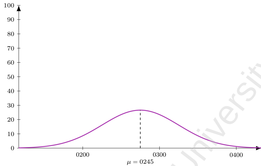
Figure 48: Flight UL 192 (DEL-CMB), dep 0515. Model M1 entry-time distribution: Normal, mean 150 min before departure ( \mu = 0245 ), SD 30 min; area = 200 pax (LF = 1).
