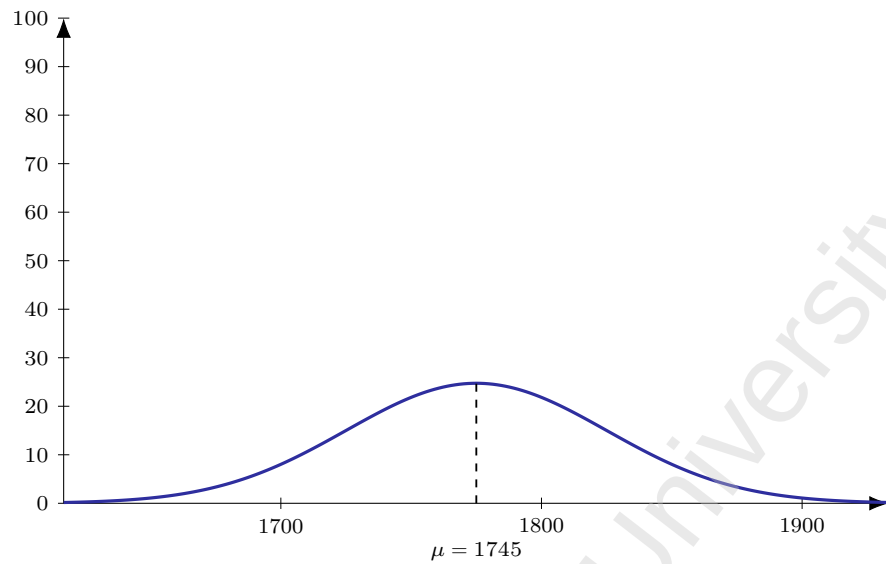
Figure 136: Flight 6E 1231 (DEL-KWI), dep 2015. Model M1 entry-time distribution: Normal, mean 150 min before departure ( \mu = 1745 ), SD 30 min; area = 186 pax (LF = 1).
