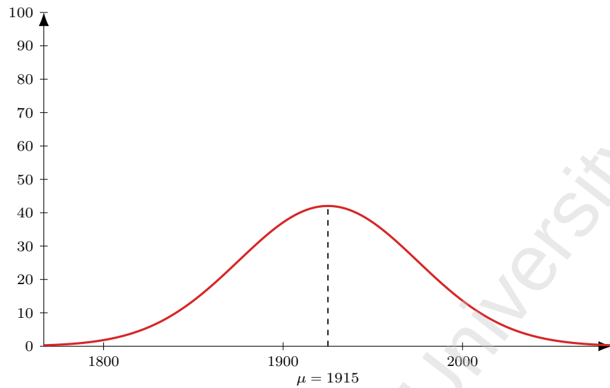
Figure 147: Flight AI 101 (DEL-FCO-JFK), dep 2145. Model M1 entry-time distribution: Normal, mean 150 min before departure ( \mu = 1915 ), SD 30 min; area = 316 pax (LF = 1).
