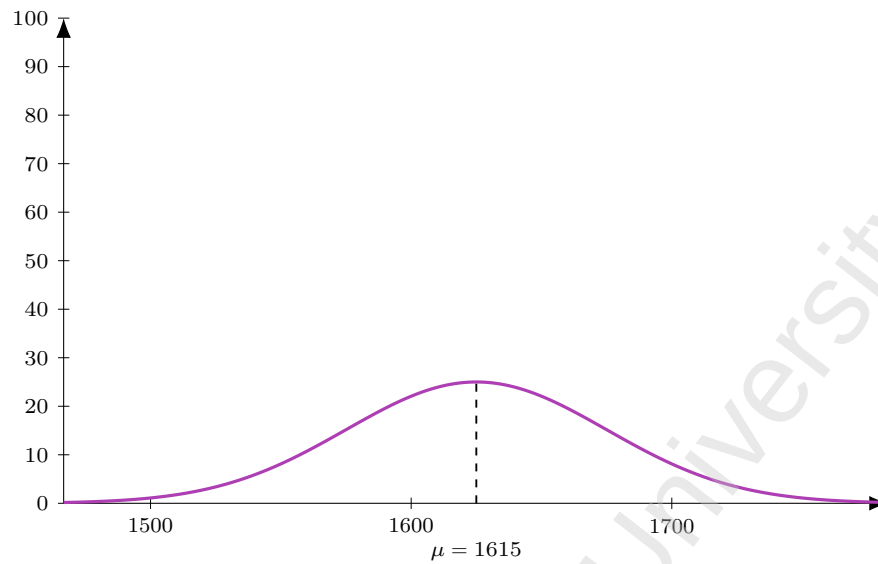
Figure 129: Flight UL 196 (DEL-CMB), dep 1845. Model M1 entry-time distribution: Normal, mean 150 min before departure ( \mu = 1615 ), SD 30 min; area = 188 pax (LF = 1).
