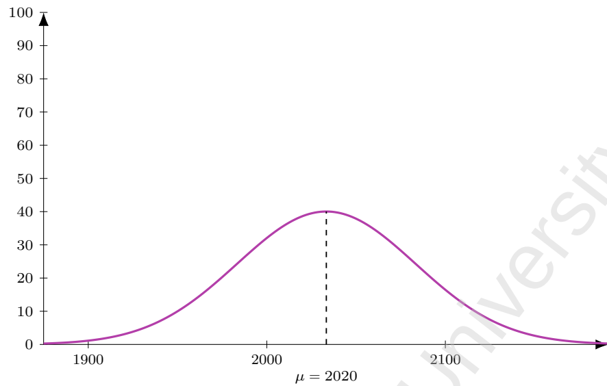
Figure 157: Flight CA 948 (DEL-PEK), dep 2250. Model M1 entry-time distribution: Normal, mean 150 min before departure ( \mu = 2020 ), SD 30 min; area = 301 pax (LF = 1).
