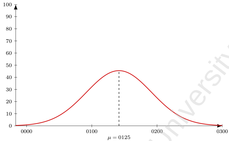
Figure 32: Flight AI 185 (DEL-YVR), dep 0355. Model M1 entry-time distribution: Normal, mean 150 min before departure ( \mu = 0125 ), SD 30 min; area = 342 pax (LF = 1).
