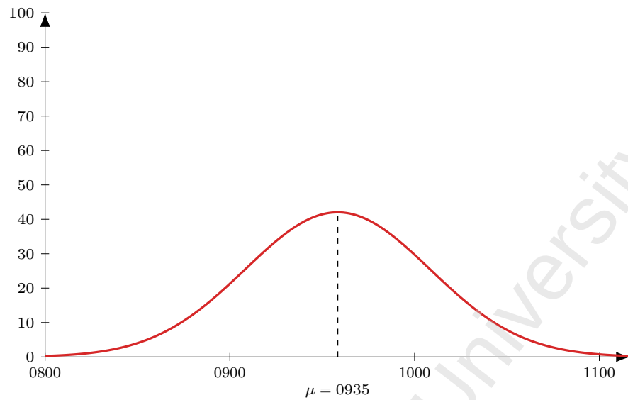
Figure 92: Flight AI 2017 (DEL-LHR), dep 1205. Model M1 entry-time distribution: Normal, mean 150 min before departure ( \mu = 0935 ), SD 30 min; area = 316 pax (LF = 1).
