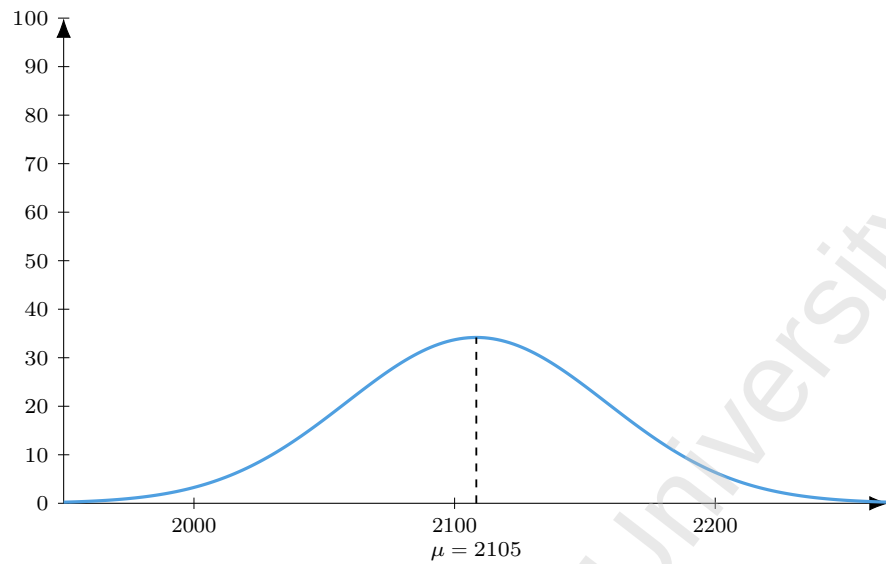
Figure 164: Flight UA 083 (DEL-EWR), dep 2335. Model M1 entry-time distribution: Normal, mean 150 min before departure ( \mu = 2105 ), SD 30 min; area = 257 pax (LF = 1).
