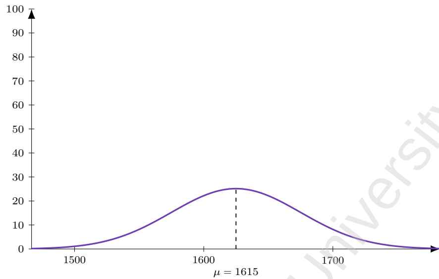
Figure 130: Flight SG 5105 (DEL-DXB), dep 1845. Model M1 entry-time distribution: Normal, mean 150 min before departure ( \mu = 1615 ), SD 30 min; area = 189 pax (LF = 1).
