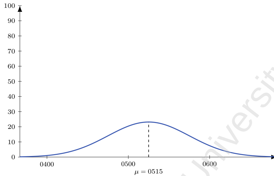
Figure 59: Flight J9 410 (DEL-KWI), dep 0745. Model M1 entry-time distribution: Normal, mean 150 min before departure ( \mu = 0515 ), SD 30 min; area = 174 pax (LF = 1).
