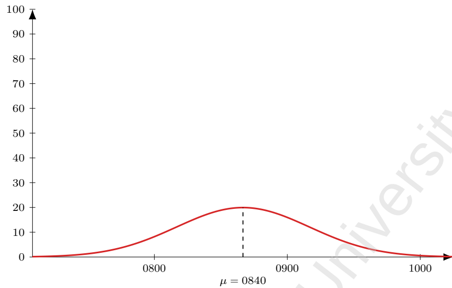
Figure 84: Flight AI 237 (DEL-DAC), dep 1110. Model M1 entry-time distribution: Normal, mean 150 min before departure ( \mu = 0840 ), SD 30 min; area = 150 pax (LF = 1).
