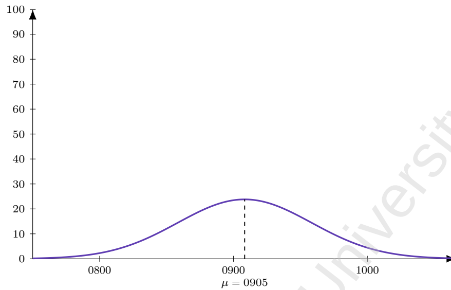
Figure 89: Flight KC 908 (DEL-ALA), dep 1135. Model M1 entry-time distribution: Normal, mean 150 min before departure ( \mu = 0905 ), SD 30 min; area = 179 pax (LF = 1).
