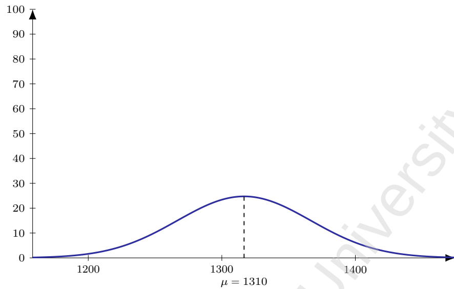
Figure 113: Flight 6E 1081 (DEL-HKT), dep 1540. Model M1 entry-time distribution: Normal, mean 150 min before departure ( \mu = 1310 ), SD 30 min; area = 186 pax (LF = 1).
