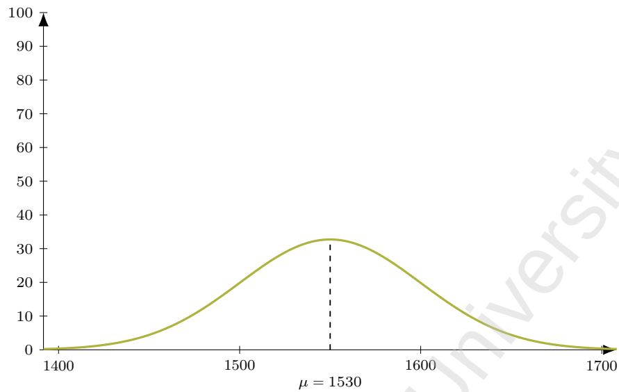
Figure 123: Flight NH 838 (DEL-HND), dep 1800. Model M1 entry-time distribution: Normal, mean 150 min before departure ( \mu = 1530 ), SD 30 min; area = 246 pax (LF = 1).
