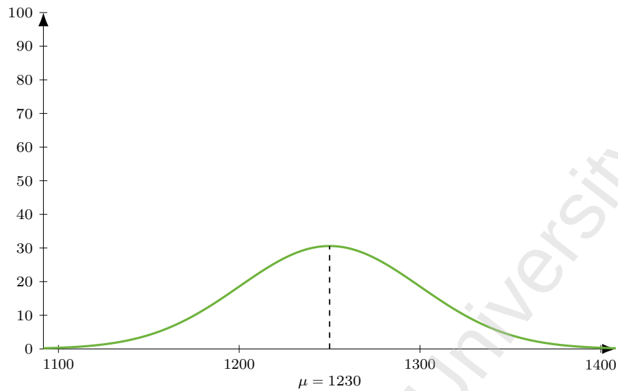
Figure 110: Flight FG 312 (DEL-KBL), dep 1500. Model M1 entry-time distribution: Normal, mean 150 min before departure ( \mu = 1230 ), SD 30 min; area = 230 pax (LF = 1).
