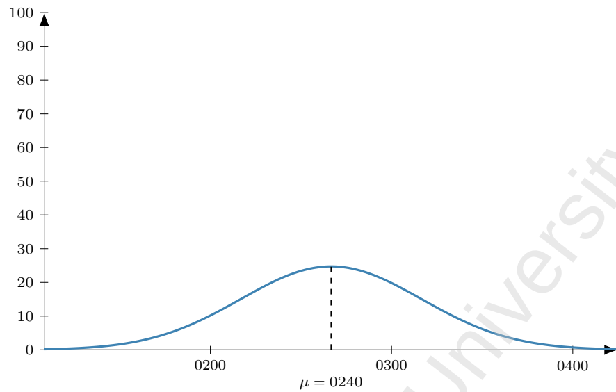
Figure 46: Flight J2 058 (DEL-GYD), dep 0510. Model M1 entry-time distribution: Normal, mean 150 min before departure ( \mu = 0240 ), SD 30 min; area = 186 pax (LF = 1).
