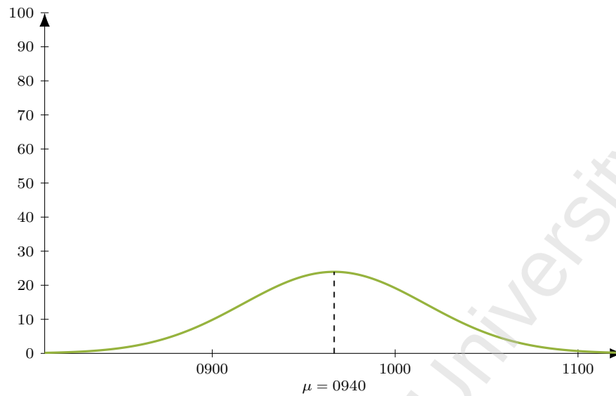
Figure 93: Flight C6 558 (DEL-TAS), dep 1210. Model M1 entry-time distribution: Normal, mean 150 min before departure ( \mu = 0940 ), SD 30 min; area = 180 pax (LF = 1).
