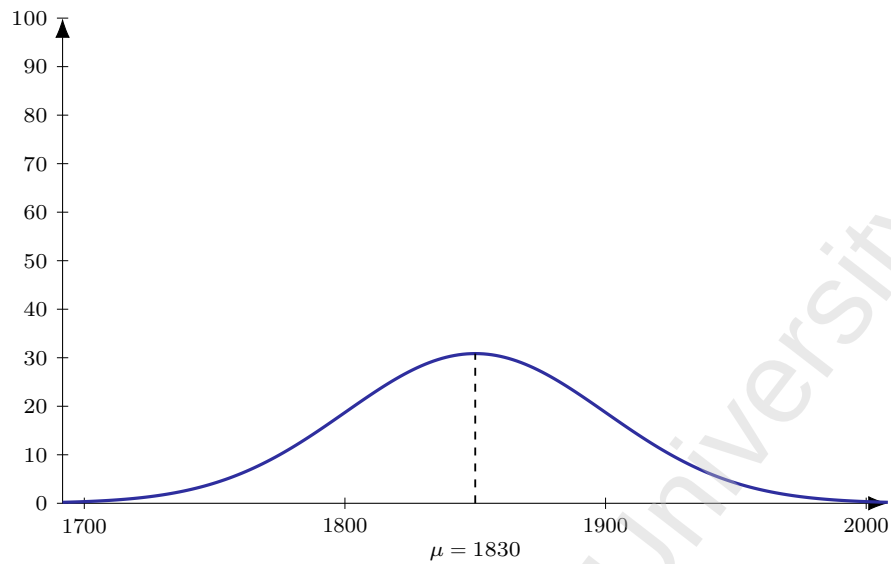
Figure 141: Flight 6E 1405 (DEL-AUH), dep 2100. Model M1 entry-time distribution: Normal, mean 150 min before departure ( \mu = 1830 ), SD 30 min; area = 232 pax (LF = 1).
