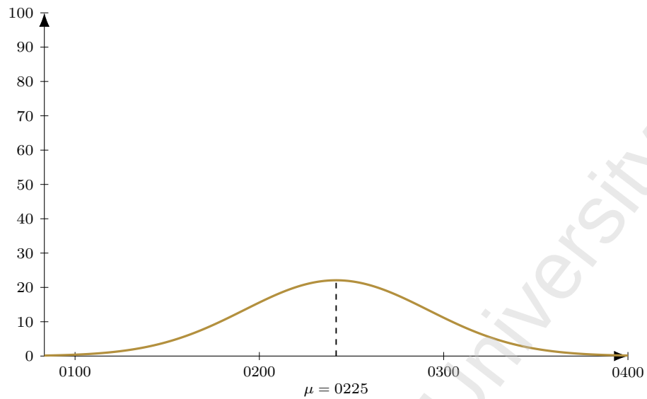
Figure 43: Flight GF 131 (DEL-BAH), dep 0455. Model M1 entry-time distribution: Normal, mean 150 min before departure ( \mu = 0225 ), SD 30 min; area = 166 pax (LF = 1).
