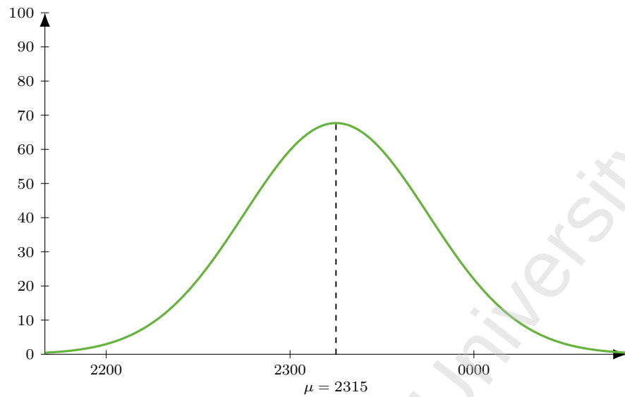
Figure 19: Flight LH 763 (DEL-MUC), dep 0145. Model M1 entry-time distribution: Normal, mean 150 min before departure ( \mu = 2315 ), SD 30 min; area = 509 pax (LF = 1).
