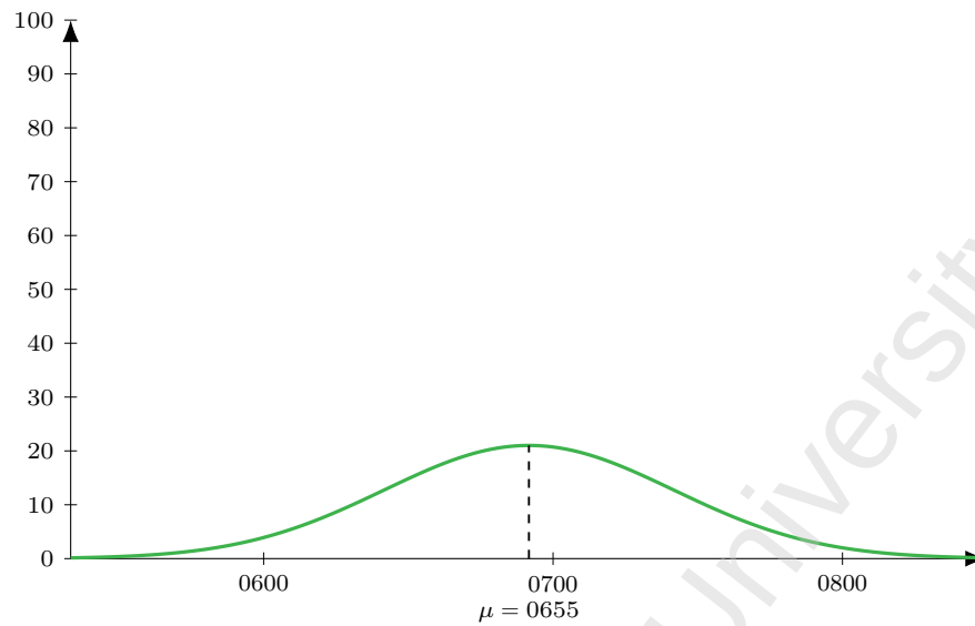
Figure 70: Flight EY 213 (DEL-AUH), dep 0925. Model M1 entry-time distribution: Normal, mean 150 min before departure ( \mu = 0655 ), SD 30 min; area = 158 pax (LF = 1).
