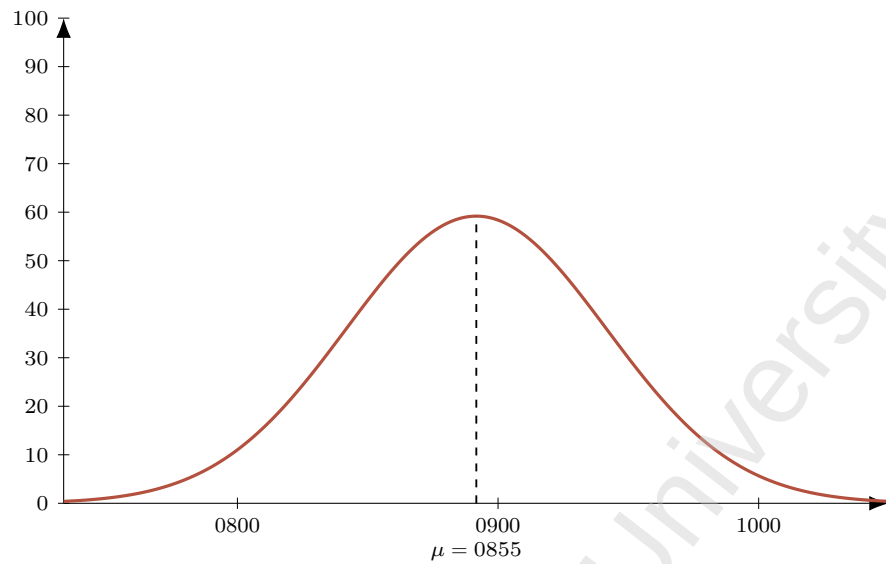
Figure 88: Flight SV 757 (DEL-JED), dep 1125. Model M1 entry-time distribution: Normal, mean 150 min before departure ( \mu = 0855 ), SD 30 min; area = 445 pax (LF = 1).
