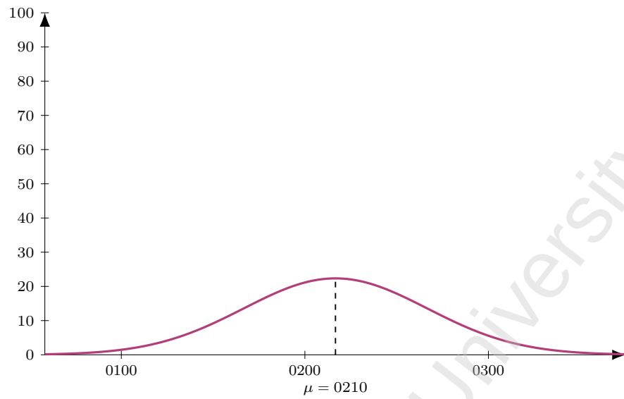
Figure 41: Flight G9 464 (DEL-SHJ), dep 0440. Model M1 entry-time distribution: Normal, mean 150 min before departure ( \mu = 0210 ), SD 30 min; area = 168 pax (LF = 1).
