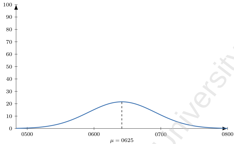
Figure 67: Flight WY 242 (DEL-MCT), dep 0855. Model M1 entry-time distribution: Normal, mean 150 min before departure ( \mu = 0625 ), SD 30 min; area = 162 pax (LF = 1).
