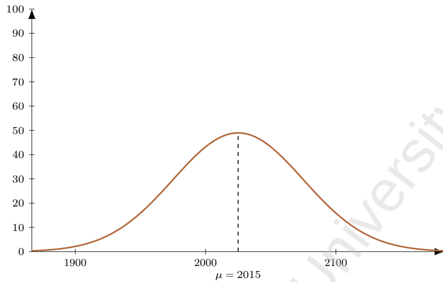
Figure 155: Flight CX 698 (DEL-HKG), dep 2245. Model M1 entry-time distribution: Normal, mean 150 min before departure ( \mu = 2015 ), SD 30 min; area = 368 pax (LF = 1).
