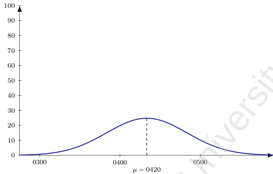
Figure 54: Flight 6E 1069 (DEL-KBV), dep 0650. Model M1 entry-time distribution: Normal, mean 150 min before departure ( \mu = 0420 ), SD 30 min; area = 186 pax (LF = 1).
