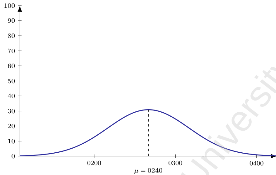
Figure 47: Flight 6E 1073 (DEL-HKT), dep 0510. Model M1 entry-time distribution: Normal, mean 150 min before departure ( \mu = 0240 ), SD 30 min; area = 232 pax (LF = 1).
