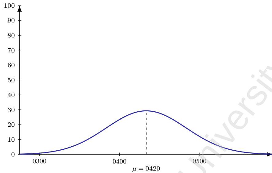
Figure 53: Flight 6E 1063 (DEL-BKK), dep 0650. Model M1 entry-time distribution: Normal, mean 150 min before departure ( \mu = 0420 ), SD 30 min; area = 220 pax (LF = 1).
