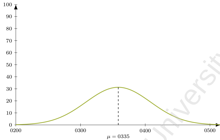
Figure 49: Flight KU 384 (DEL-KWI), dep 0605. Model M1 entry-time distribution: Normal, mean 150 min before departure ( \mu = 0335 ), SD 30 min; area = 235 pax (LF = 1).
