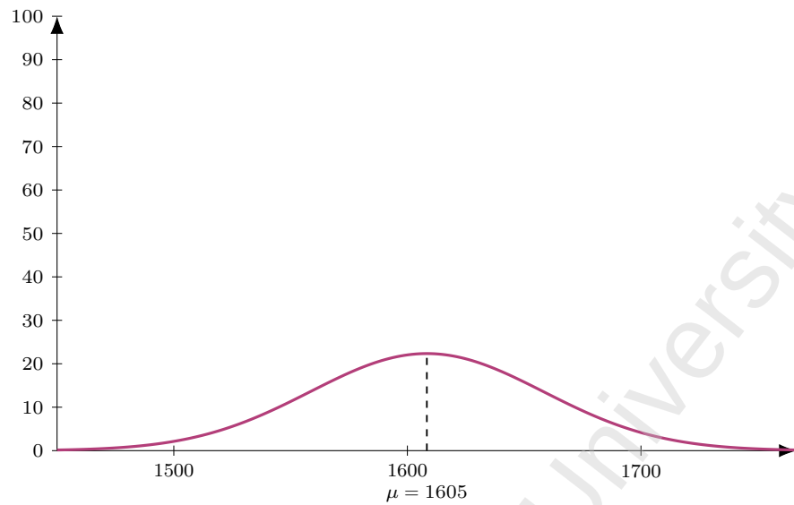
Figure 127: Flight G9 466 (DEL-SHJ), dep 1835. Model M1 entry-time distribution: Normal, mean 150 min before departure ( \mu = 1605 ), SD 30 min; area = 168 pax (LF = 1).
