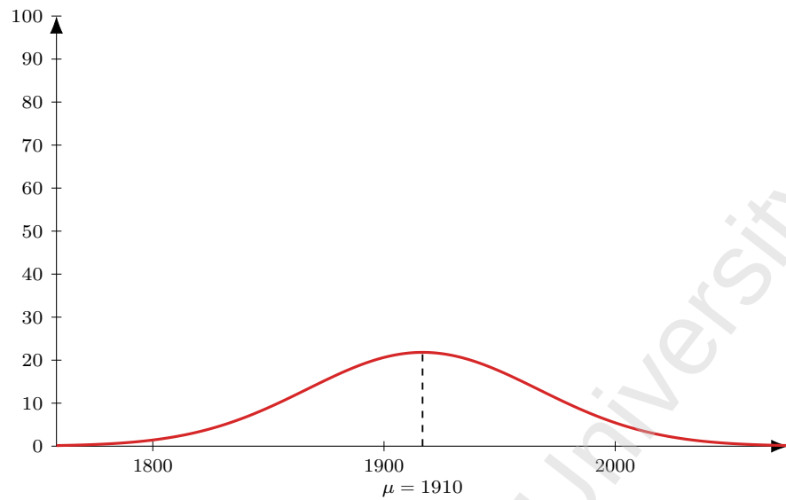
Figure 146: Flight AI 2386 (DEL-KUL), dep 2140. Model M1 entry-time distribution: Normal, mean 150 min before departure ( \mu = 1910 ), SD 30 min; area = 164 pax (LF = 1).
