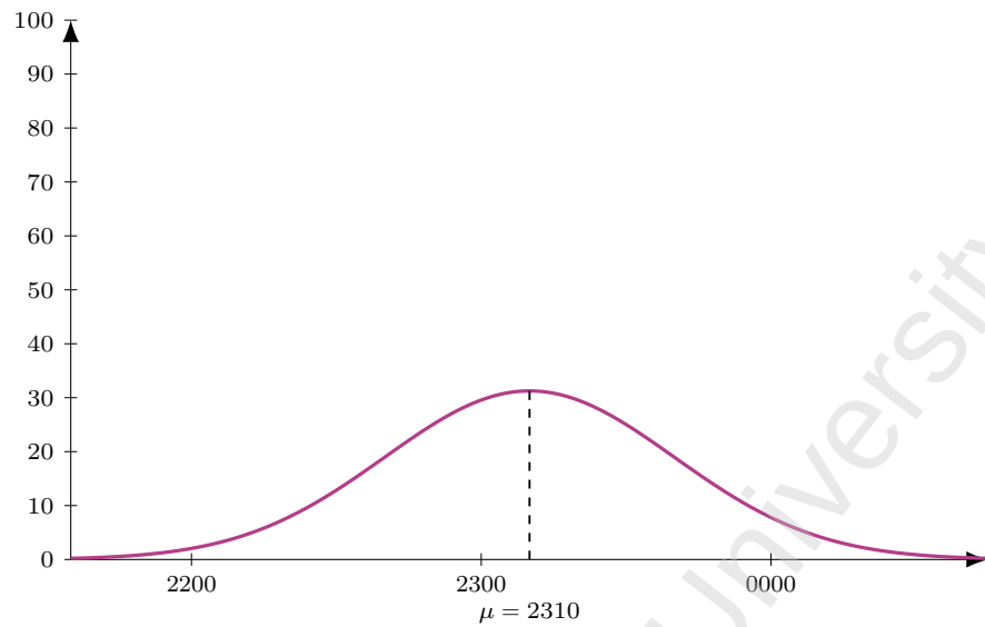
Figure 18: Flight LX 2647 (DEL-ZRH), dep 0140. Model M1 entry-time distribution: Normal, mean 150 min before departure ( \mu = 2310 ), SD 30 min; area = 235 pax (LF = 1).
