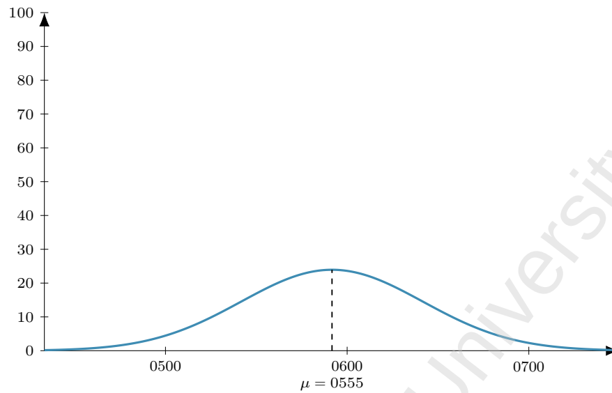
Figure 65: Flight IX 179 (DEL-AUH), dep 0825. Model M1 entry-time distribution: Normal, mean 150 min before departure ( \mu = 0555 ), SD 30 min; area = 180 pax (LF = 1).
