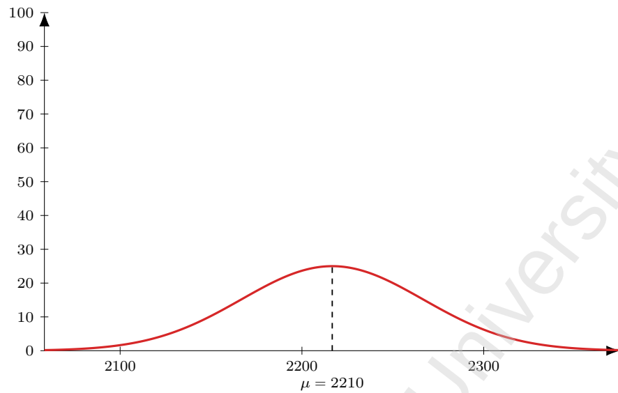
Figure 7: Flight AI 2118 (DEL-SIN), dep 0040. Model M1 entry-time distribution: Normal, mean 150 min before departure ( \mu = 2210 ), SD 30 min; area = 188 pax (LF = 1).
