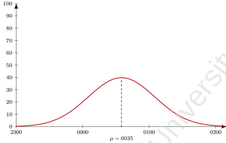
Figure 28: Flight AI 2025 (DEL-FRA), dep 0305. Model M1 entry-time distribution: Normal, mean 150 min before departure ( \mu = 0035 ), SD 30 min; area = 299 pax (LF = 1).
