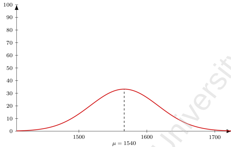
Figure 124: Flight AI 358 (DEL-HND), dep 1810. Model M1 entry-time distribution: Normal, mean 150 min before departure ( \mu = 1540 ), SD 30 min; area = 250 pax (LF = 1).
