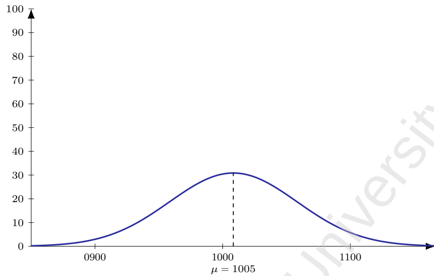
Figure 99: Flight 6E 1103 (DEL-DAC), dep 1235. Model M1 entry-time distribution: Normal, mean 150 min before departure ( \mu = 1005 ), SD 30 min; area = 232 pax (LF = 1).
