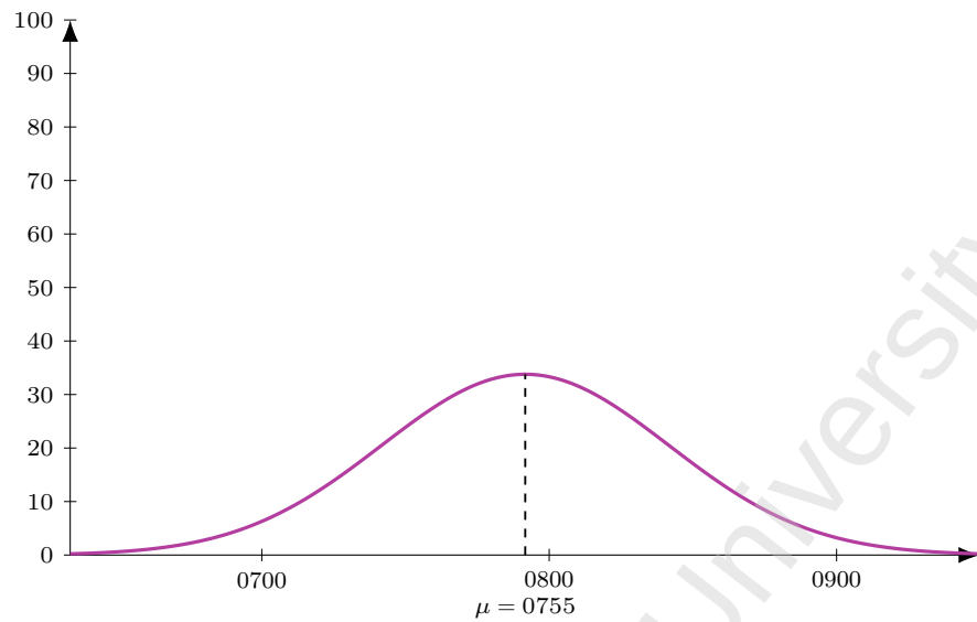
Figure 75: Flight QR 571 (DEL-DOH), dep 1025. Model M1 entry-time distribution: Normal, mean 150 min before departure ( \mu = 0755 ), SD 30 min; area = 254 pax (LF = 1).
