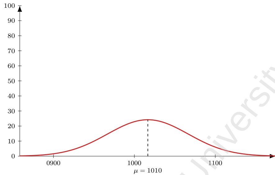
Figure 100: Flight AI 281 (DEL-CMB), dep 1240. Model M1 entry-time distribution: Normal, mean 150 min before departure ( \mu = 1010 ), SD 30 min; area = 182 pax (LF = 1).
