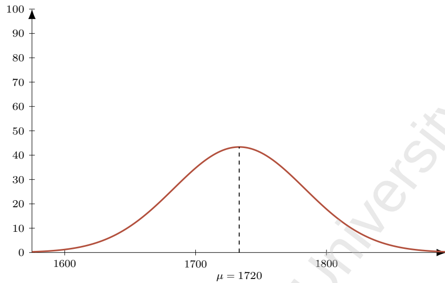
Figure 134: Flight SV 9651 (DEL-MED), dep 1950. Model M1 entry-time distribution: Normal, mean 150 min before departure ( \mu = 1720 ), SD 30 min; area = 326 pax (LF = 1).
