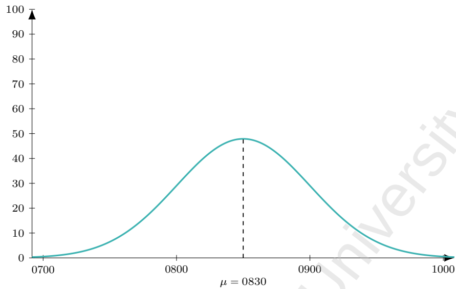
Figure 83: Flight EK 511 (DEL-DXB), dep 1100. Model M1 entry-time distribution: Normal, mean 150 min before departure ( \mu = 0830 ), SD 30 min; area = 360 pax (LF = 1).
