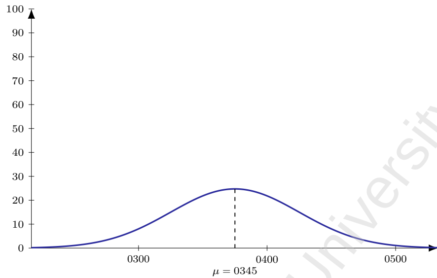
Figure 50: Flight 6E 1721 (DEL-HKG), dep 0615. Model M1 entry-time distribution: Normal, mean 150 min before departure ( \mu = 0345 ), SD 30 min; area = 186 pax (LF = 1).
