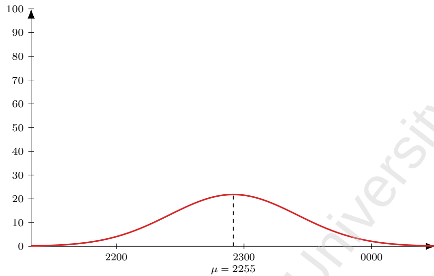
Figure 16: Flight AI 2378 (DEL-HKT), dep 0125. Model M1 entry-time distribution: Normal, mean 150 min before departure ( \mu = 2255 ), SD 30 min; area = 164 pax (LF = 1).
