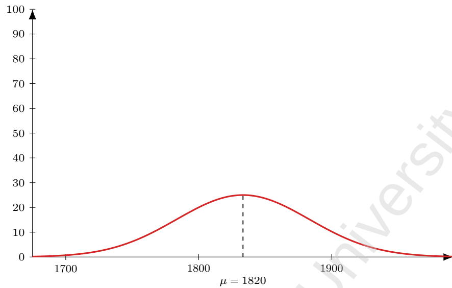
Figure 138: Flight AI 2145 (DEL-DPS), dep 2050. Model M1 entry-time distribution: Normal, mean 150 min before departure ( \mu = 1820 ), SD 30 min; area = 188 pax (LF = 1).
