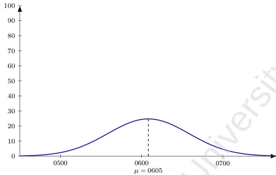
Figure 66: Flight 6E 1461 (DEL-DXB), dep 0835. Model M1 entry-time distribution: Normal, mean 150 min before departure ( \mu = 0605 ), SD 30 min; area = 186 pax (LF = 1).
