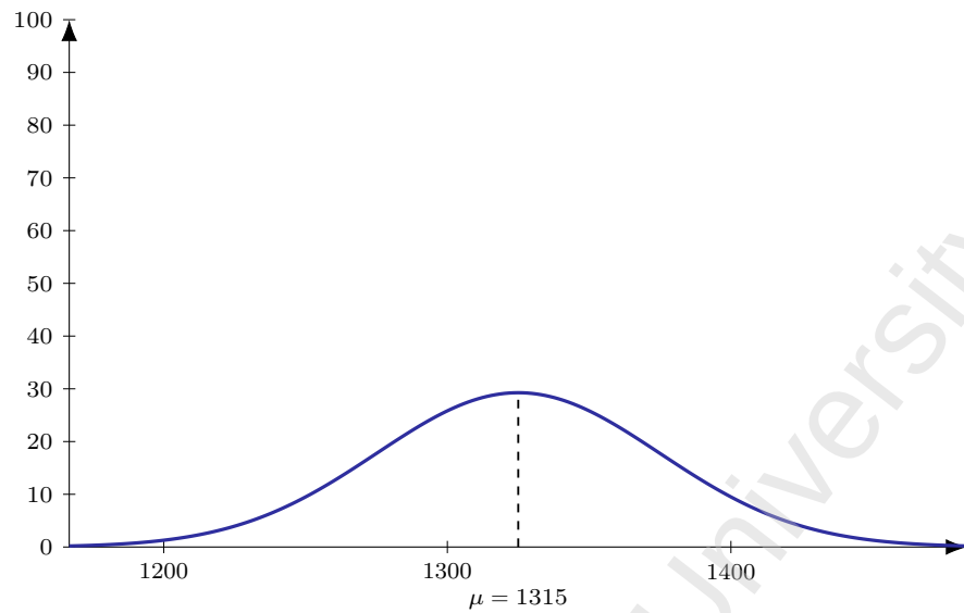
Figure 114: Flight 6E 1053 (DEL-BKK), dep 1545. Model M1 entry-time distribution: Normal, mean 150 min before departure ( \mu = 1315 ), SD 30 min; area = 220 pax (LF = 1).
