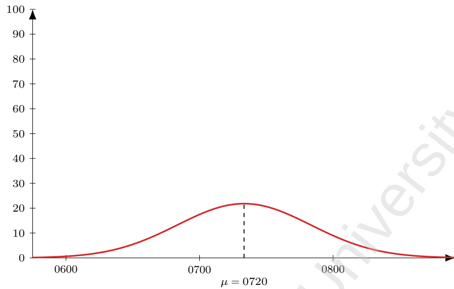
Figure 73: Flight AI 917 (DEL-DXB), dep 0950. Model M1 entry-time distribution: Normal, mean 150 min before departure ( \mu = 0720 ), SD 30 min; area = 164 pax (LF = 1).
