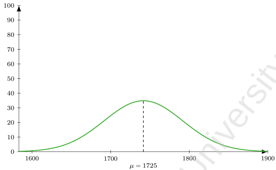
Figure 135: Flight MU 564 (DEL-PVG), dep 1955. Model M1 entry-time distribution: Normal, mean 150 min before departure ( \mu = 1725 ), SD 30 min; area = 262 pax (LF = 1).
