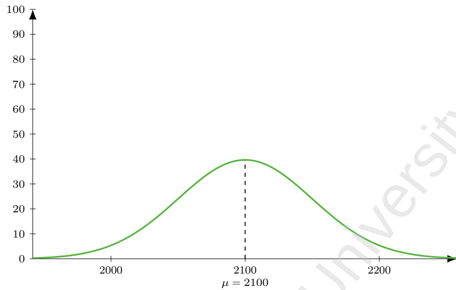
Figure 162: Flight TG 316 (DEL-BKK), dep 2330. Model M1 entry-time distribution: Normal, mean 150 min before departure ( \mu = 2100 ), SD 30 min; area = 298 pax (LF = 1).
