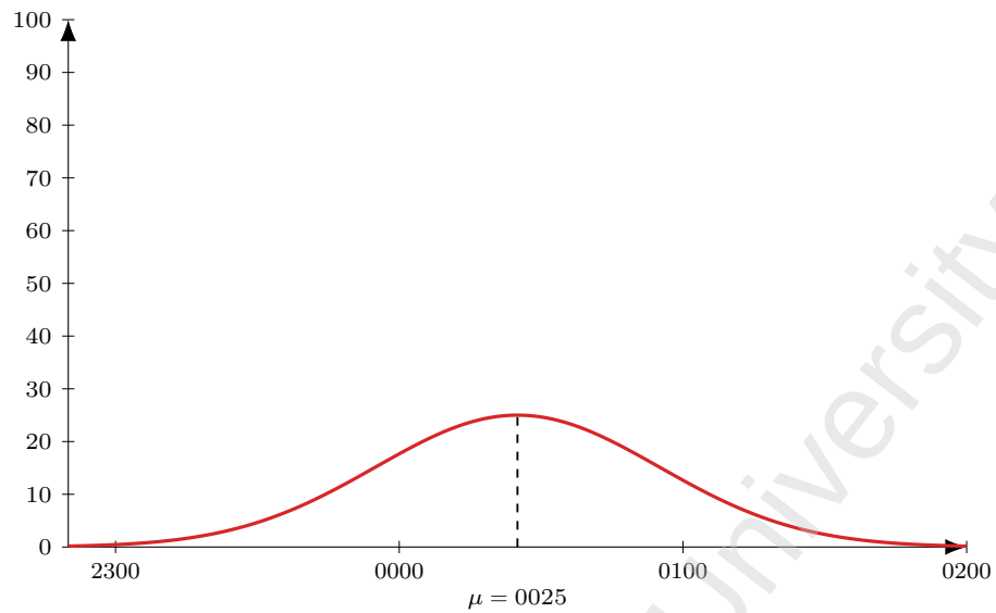
Figure 25: Flight AI 2147 (DEL-DPS), dep 0255. Model M1 entry-time distribution: Normal, mean 150 min before departure ( \mu = 0025 ), SD 30 min; area = 188 pax (LF = 1).
