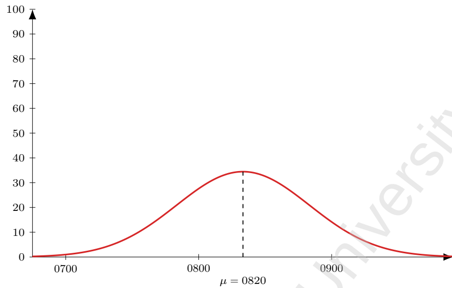
Figure 78: Flight AI 113 (DEL-BHX), dep 1050. Model M1 entry-time distribution: Normal, mean 150 min before departure ( \mu = 0820 ), SD 30 min; area = 259 pax (LF = 1).
