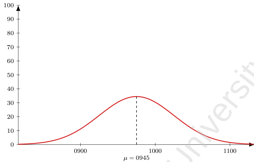
Figure 94: Flight AI 151 (DEL-ZRH), dep 1215. Model M1 entry-time distribution: Normal, mean 150 min before departure ( \mu = 0945 ), SD 30 min; area = 259 pax (LF = 1).
