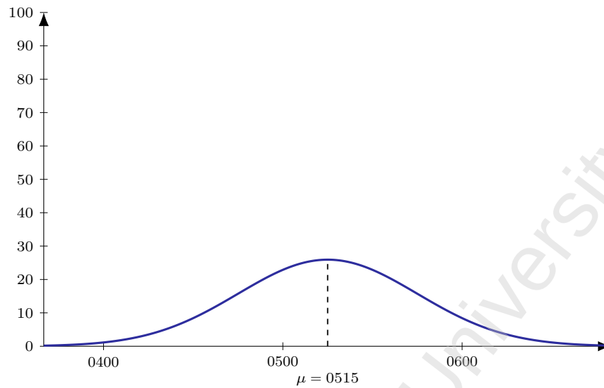
Figure 58: Flight 6E 011 (DEL-IST), dep 0745. Model M1 entry-time distribution: Normal, mean 150 min before departure ( \mu = 0515 ), SD 30 min; area = 195 pax (LF = 1).
