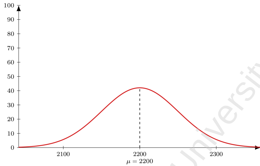
Figure 5: Flight AI 161 (DEL-LHR), dep 0030. Model M1 entry-time distribution: Normal, mean 150 min before departure ( \mu = 2200 ), SD 30 min; area = 316 pax (LF = 1).
