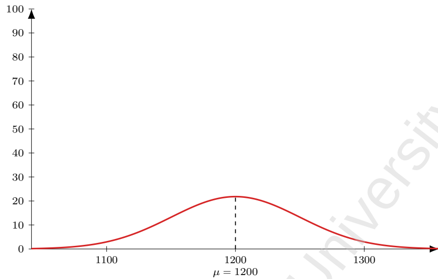
Figure 109: Flight AI 2304 (DEL-BKK), dep 1430. Model M1 entry-time distribution: Normal, mean 150 min before departure ( \mu = 1200 ), SD 30 min; area = 164 pax (LF = 1).
