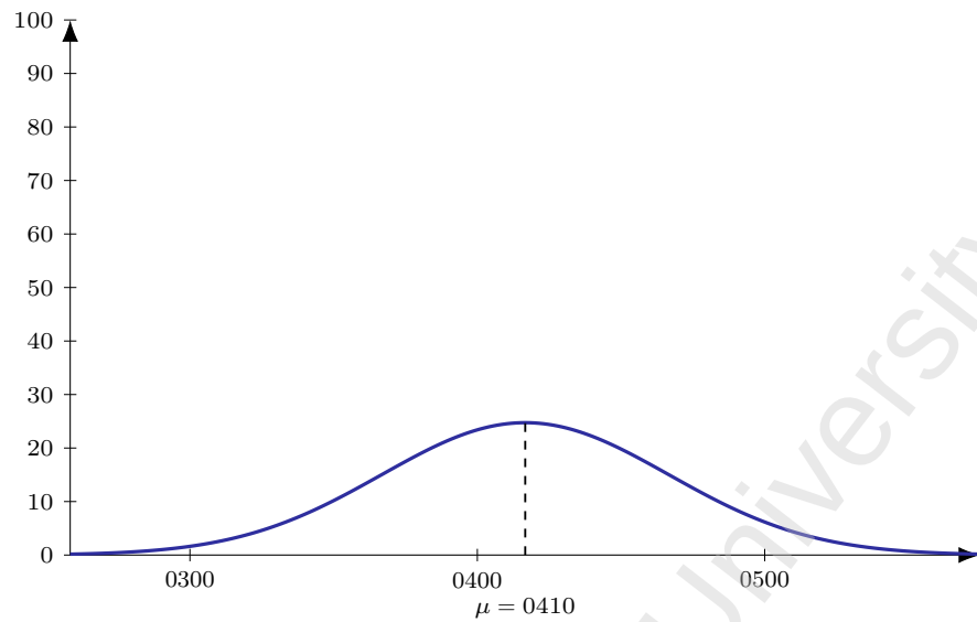
Figure 52: Flight 6E 1611 (DEL-BBI-DPS), dep 0640. Model M1 entry-time distribution: Normal, mean 150 min before departure ( \mu = 0410 ), SD 30 min; area = 186 pax (LF = 1).
