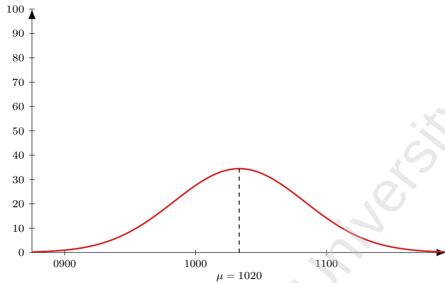
Figure 101: Flight AI 137 (DEL-MXP), dep 1250. Model M1 entry-time distribution: Normal, mean 150 min before departure ( \mu = 1020 ), SD 30 min; area = 259 pax (LF = 1).
