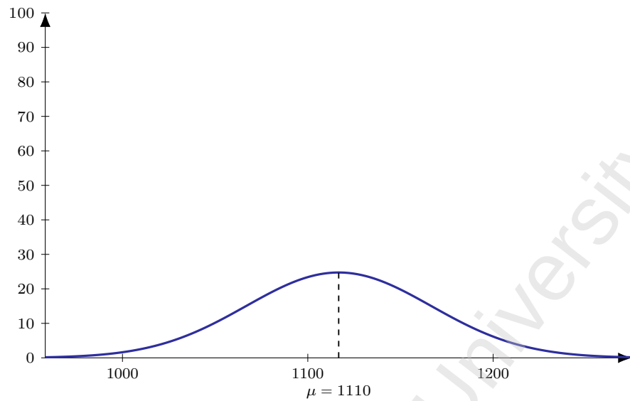
Figure 104: Flight 6E 1155 (DEL-KTM), dep 1340. Model M1 entry-time distribution: Normal, mean 150 min before departure ( \mu = 1110 ), SD 30 min; area = 186 pax (LF = 1).
