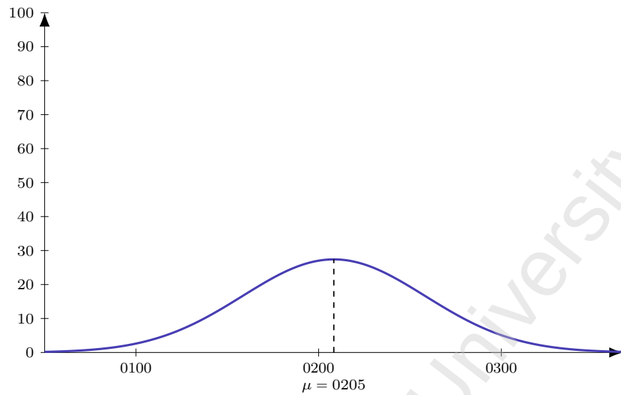
Figure 40: Flight JL 740 (DEL-NRT), dep 0435. Model M1 entry-time distribution: Normal, mean 150 min before departure ( \mu = 0205 ), SD 30 min; area = 206 pax (LF = 1).
