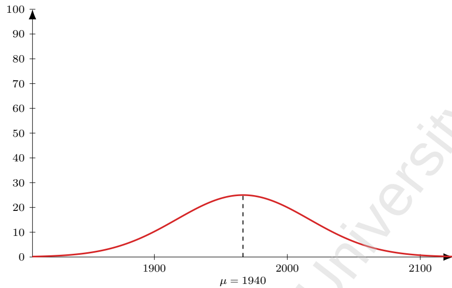
Figure 154: Flight AI 314 (DEL-HKG), dep 2210. Model M1 entry-time distribution: Normal, mean 150 min before departure ( \mu = 1940 ), SD 30 min; area = 188 pax (LF = 1).
