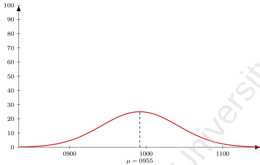
Figure 97: Flight AI 2362 (DEL-MNL), dep 1225. Model M1 entry-time distribution: Normal, mean 150 min before departure ( \mu = 0955 ), SD 30 min; area = 188 pax (LF = 1).
