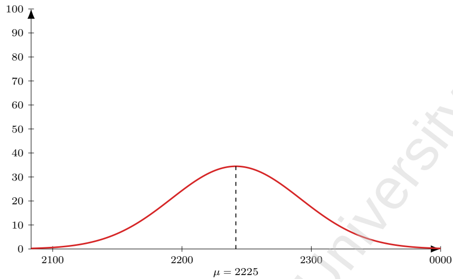
Figure 9: Flight AI 302 (DEL-SYD), dep 0055. Model M1 entry-time distribution: Normal, mean 150 min before departure ( \mu = 2225 ), SD 30 min; area = 259 pax (LF = 1).
