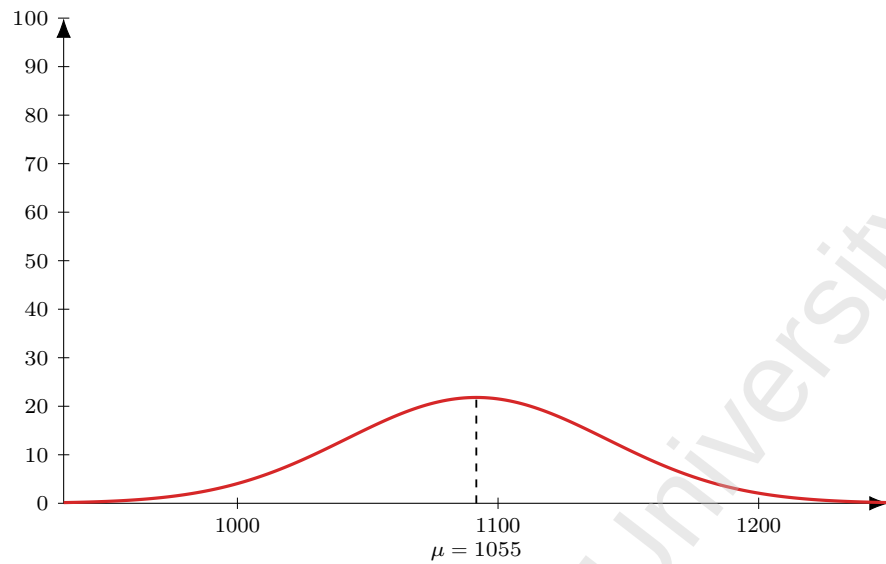
Figure 103: Flight AI 2376 (DEL-HKT), dep 1325. Model M1 entry-time distribution: Normal, mean 150 min before departure ( \mu = 1055 ), SD 30 min; area = 164 pax (LF = 1).
