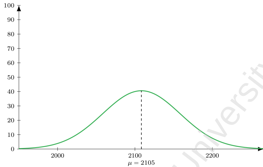
Figure 163: Flight VN 980 (DEL-HAN), dep 2335. Model M1 entry-time distribution: Normal, mean 150 min before departure ( \mu = 2105 ), SD 30 min; area = 305 pax (LF = 1).
