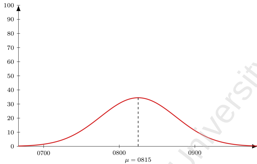
Figure 77: Flight AI 143 (DEL-CDG), dep 1045. Model M1 entry-time distribution: Normal, mean 150 min before departure ( \mu = 0815 ), SD 30 min; area = 259 pax (LF = 1).
