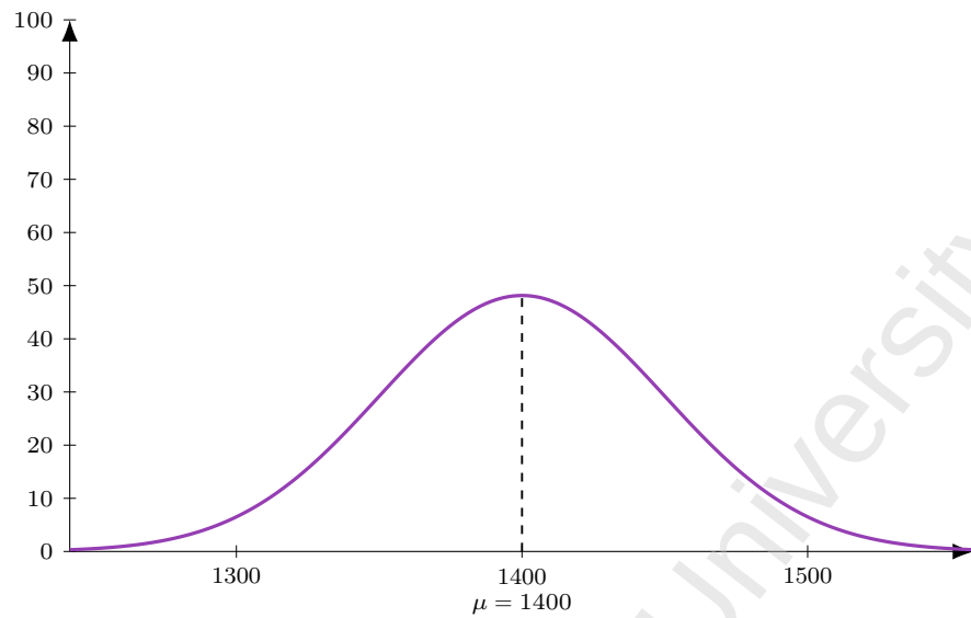
Figure 120: Flight IA 444 (DEL-BGW), dep 1630. Model M1 entry-time distribution: Normal, mean 150 min before departure ( \mu = 1400 ), SD 30 min; area = 362 pax (LF = 1).
