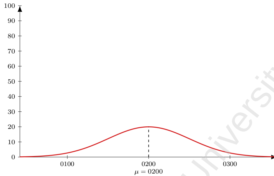
Figure 38: Flight AI 215 (DEL-KTM), dep 0430. Model M1 entry-time distribution: Normal, mean 150 min before departure ( \mu = 0200 ), SD 30 min; area = 150 pax (LF = 1).
