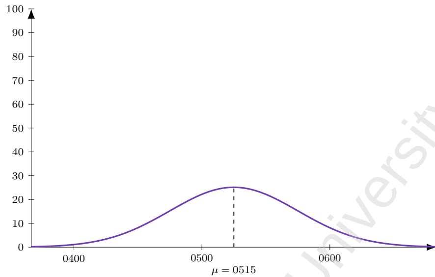
Figure 60: Flight SG 5111 (DEL-DXB), dep 0745. Model M1 entry-time distribution: Normal, mean 150 min before departure ( \mu = 0515 ), SD 30 min; area = 189 pax (LF = 1).
