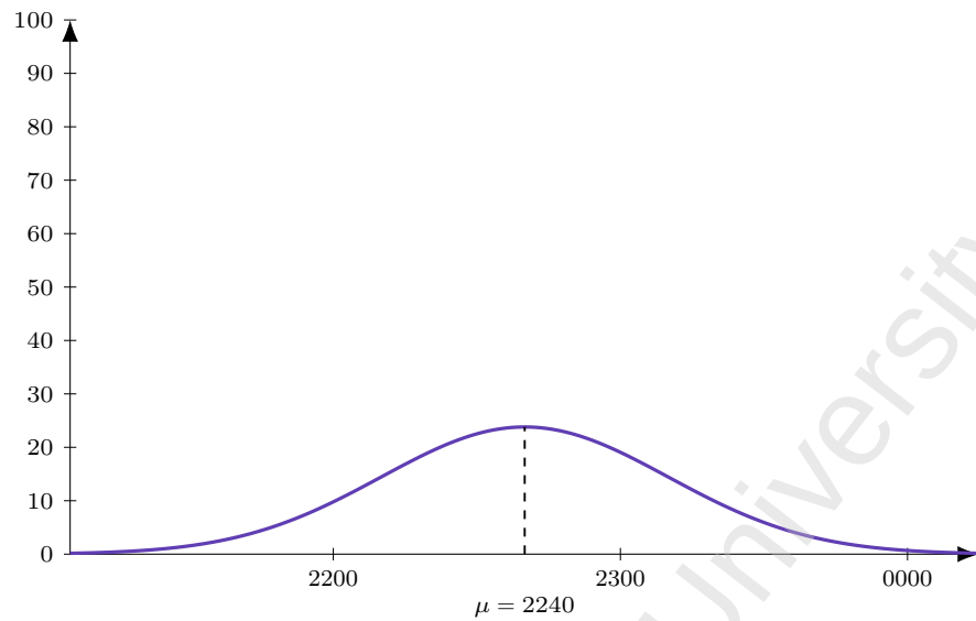
Figure 13: Flight KC 964 (DEL-ALA), dep 0110. Model M1 entry-time distribution: Normal, mean 150 min before departure ( \mu = 2240 ), SD 30 min; area = 179 pax (LF = 1).
