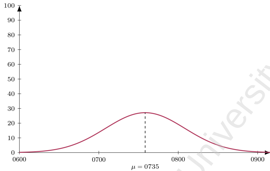
Figure 74: Flight BA 256 (DEL-LHR), dep 1005. Model M1 entry-time distribution: Normal, mean 150 min before departure ( \mu = 0735 ), SD 30 min; area = 204 pax (LF = 1).
