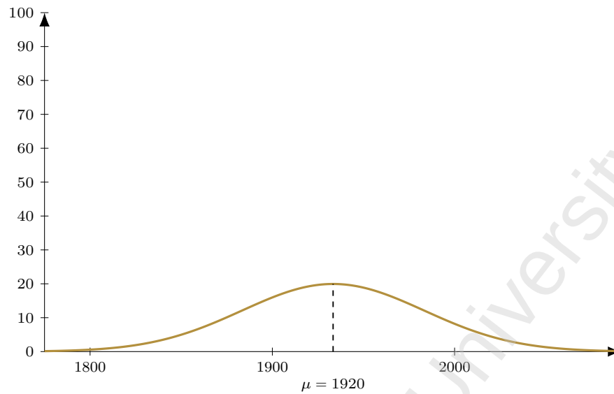
Figure 148: Flight GF 135 (DEL-BAH), dep 2150. Model M1 entry-time distribution: Normal, mean 150 min before departure ( \mu = 1920 ), SD 30 min; area = 150 pax (LF = 1).
