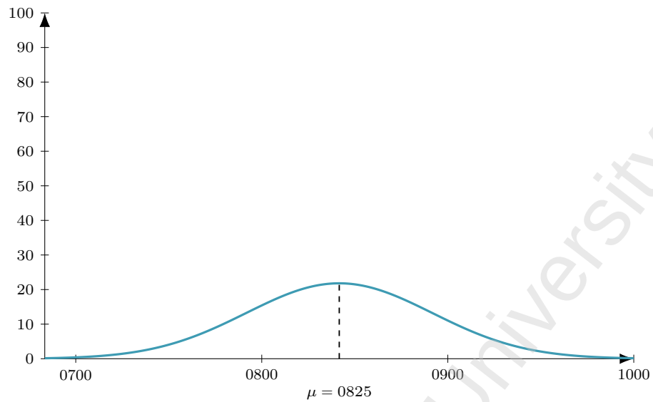
Figure 81: Flight K9 1602 (DEL-BSZ), dep 1055. Model M1 entry-time distribution: Normal, mean 150 min before departure ( \mu = 0825 ), SD 30 min; area = 164 pax (LF = 1).
