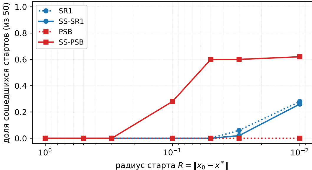
Rosenbrock chained, n = 10 , без Armijo ( \alpha_k \equiv 1 )
