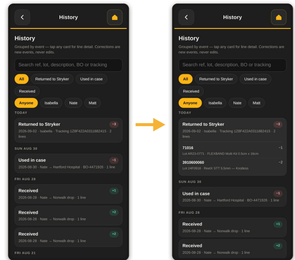
History with the filter chips, and a send-back card expanded to show its lines.
