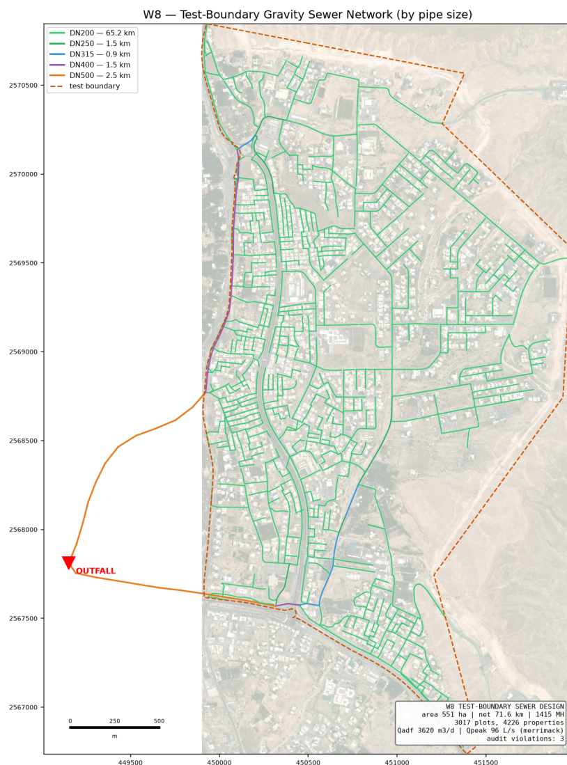
The designed sewer, coloured by pipe size.
