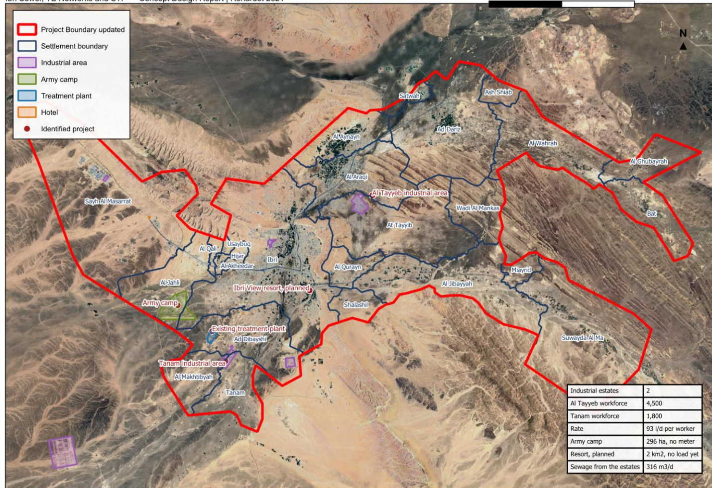
Figure 26 The identified projects and special consumers, with the two industrial estates and the army camp outlined.
