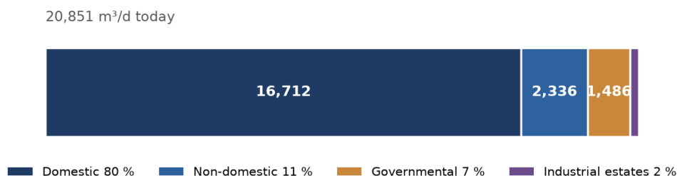
Figure 23 Average sewage flow in 2024 by stream.
