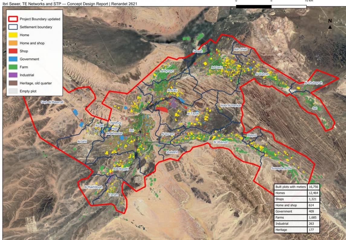
Figure 6 Use of each plot derived from the meters and the satellite. Empty plots are shown in grey.
