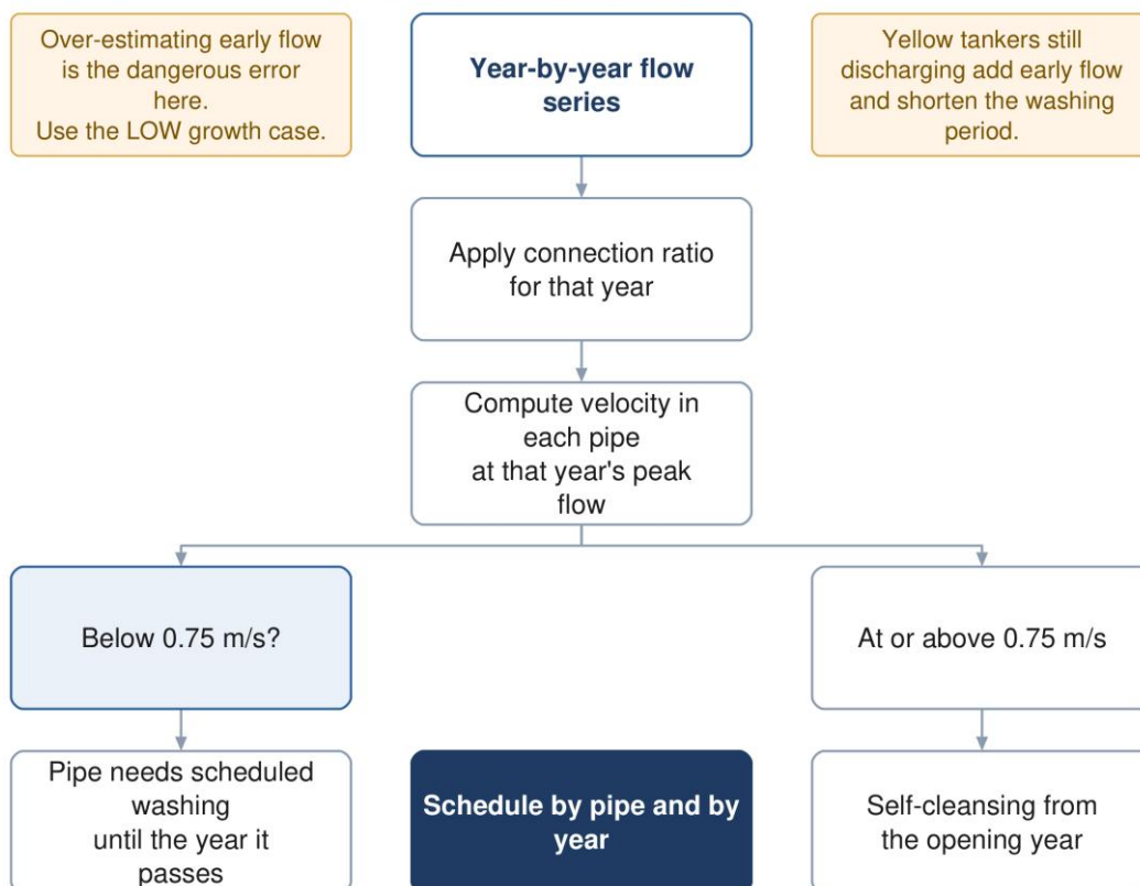
Figure 18 Setting the washing schedule, from the concept methodology. It shows the velocity test only; Sections 12.3 and 12.5 add the tractive test and the three classes. Its tanker note is not applied: no tanker flow is in any design flow until the delivery records are received.
