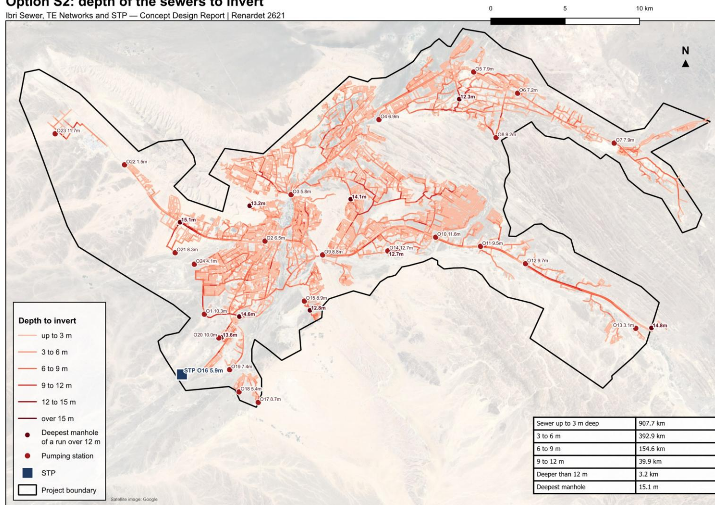
Figure 81. Option S2: depth of the sewers to invert in the 2070 design, the depth of each pumping station's outfall, and the deepest manhole of every run deeper than 12 m.
