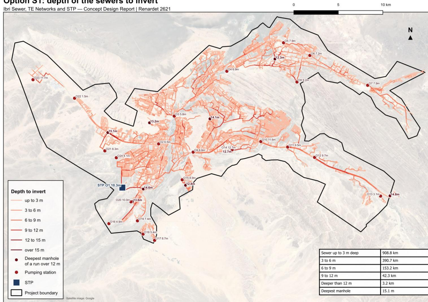
Figure 80. Option S1: depth of the sewers to invert in the 2070 design, the depth of each pumping station's outfall, and the deepest manhole of every run deeper than 12 m.
