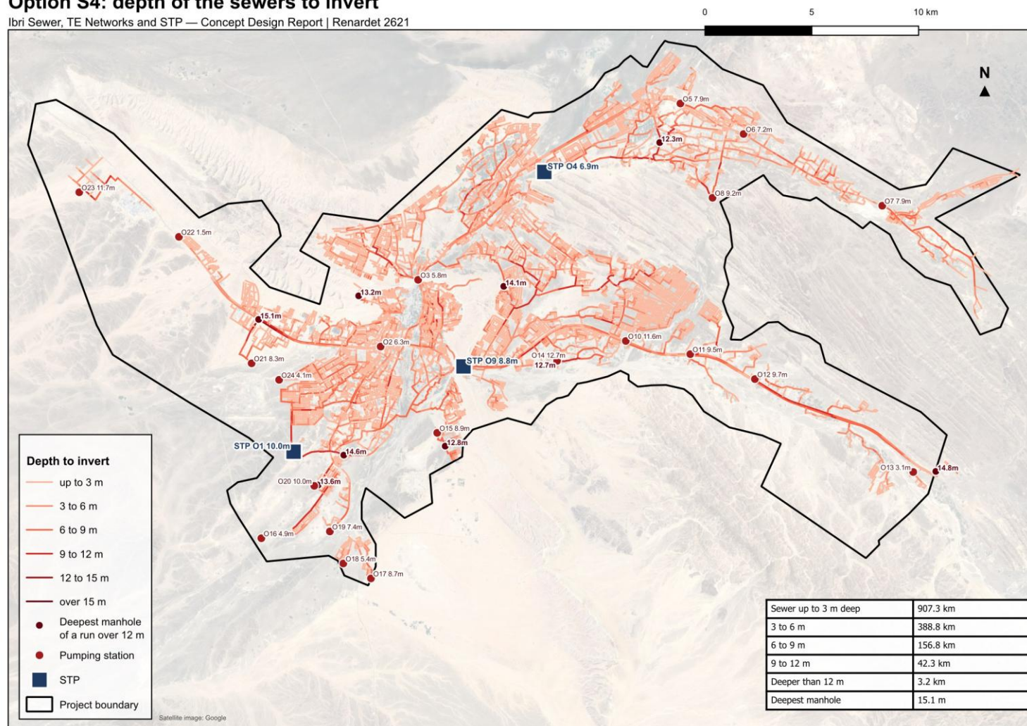
Figure 83. Option S4: depth of the sewers to invert in the 2070 design, the depth of each pumping station's outfall, and the deepest manhole of every run deeper than 12 m.
