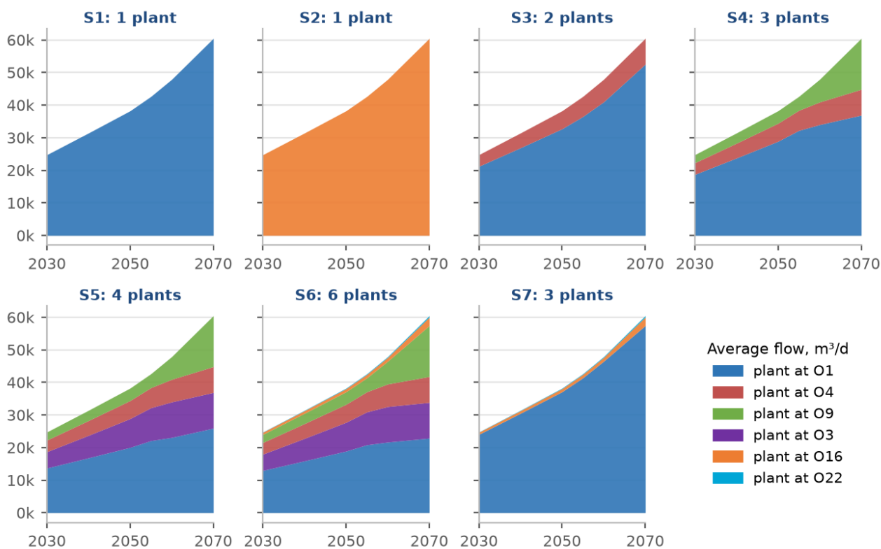
Figure 78. The average flow arriving at each plant, 2030 to 2070, by option.
