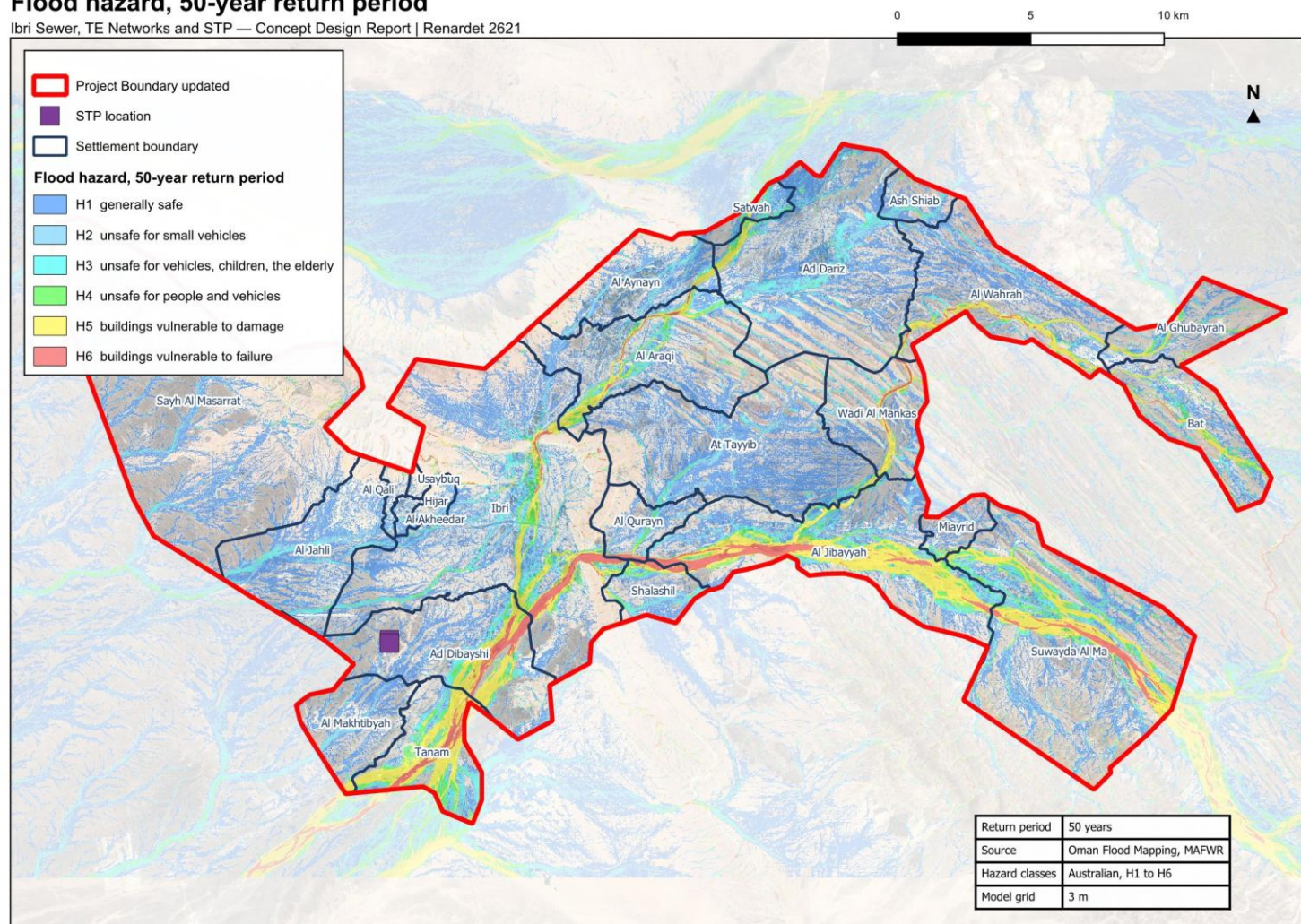
Figure 11. Flood hazard in the study area, 50-year return period. Oman Flood Mapping project, MAFWR; Australian hazard classes.
