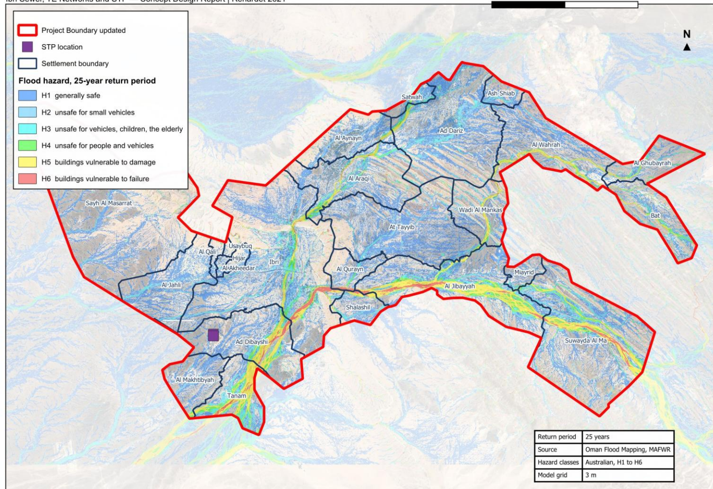
Figure 10. Flood hazard in the study area, 25-year return period. Oman Flood Mapping project, MAFWR; Australian hazard classes.
