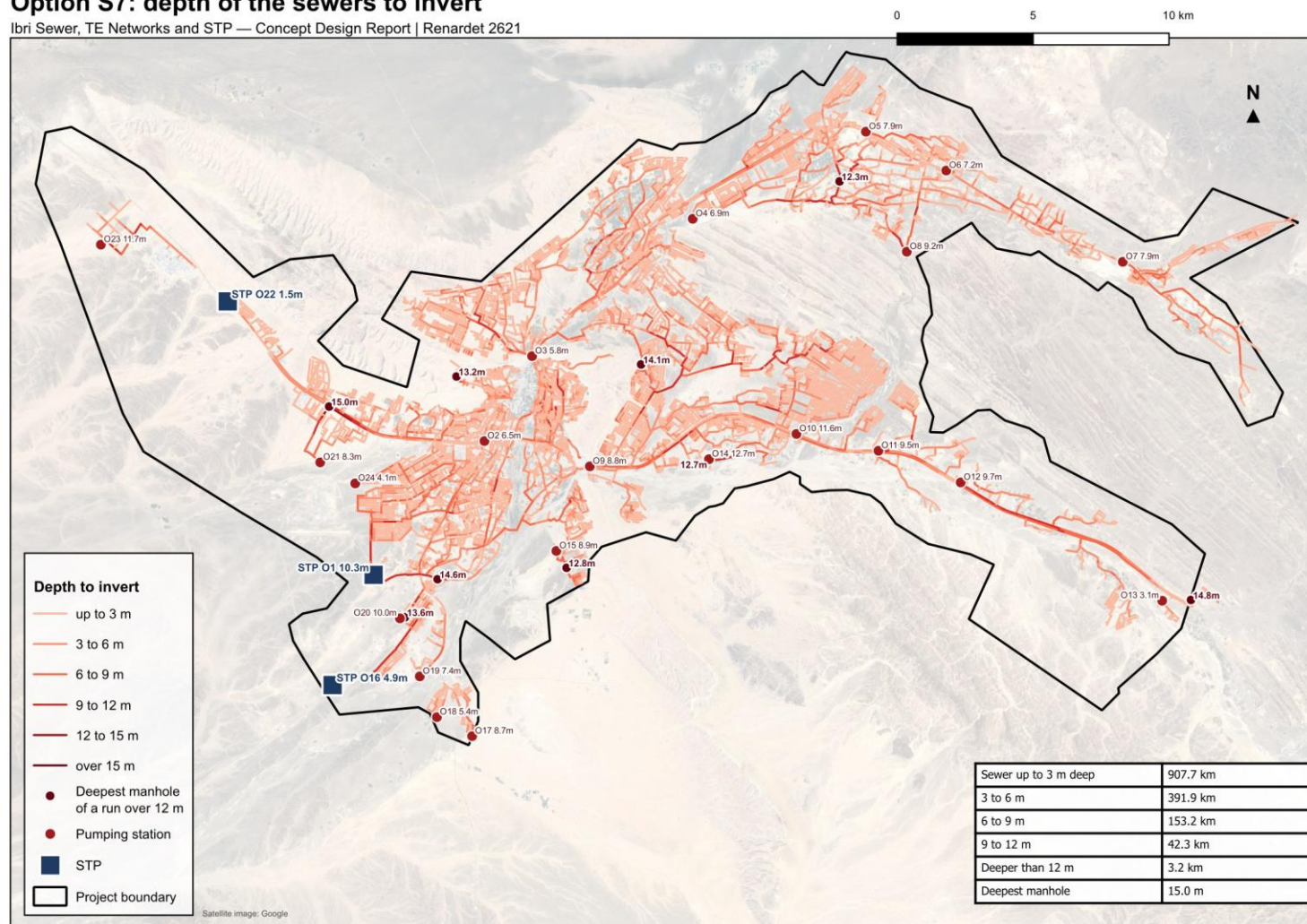
Figure 86. Option S7: depth of the sewers to invert in the 2070 design, the depth of each pumping station's outfall, and the deepest manhole of every run deeper than 12 m.
