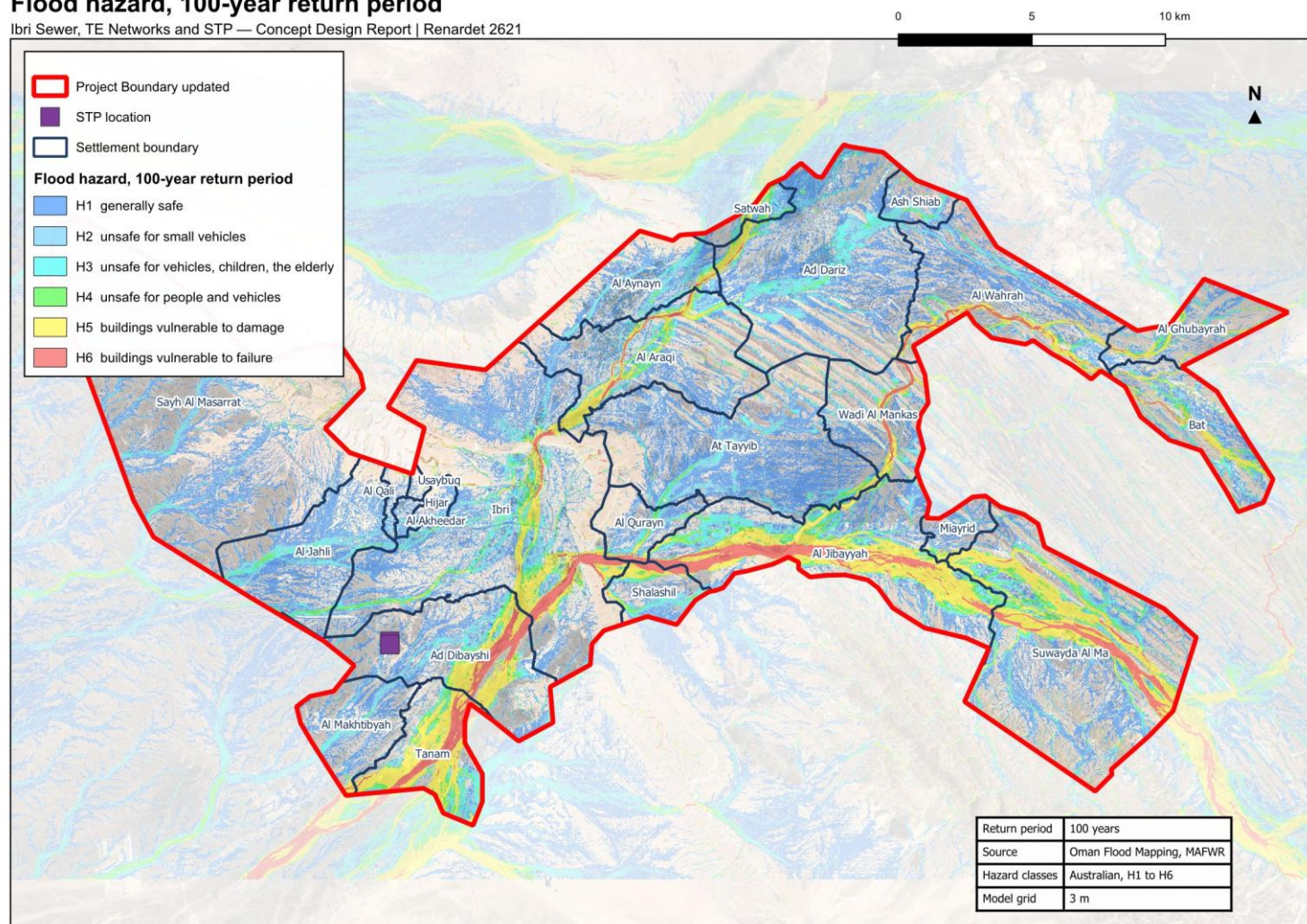
Figure 12. Flood hazard in the study area, 100-year return period. Oman Flood Mapping project, MAFWR; Australian hazard classes.
