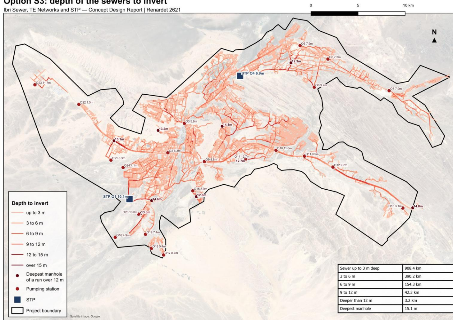
Figure 82. Option S3: depth of the sewers to invert in the 2070 design, the depth of each pumping station's outfall, and the deepest manhole of every run deeper than 12 m.
