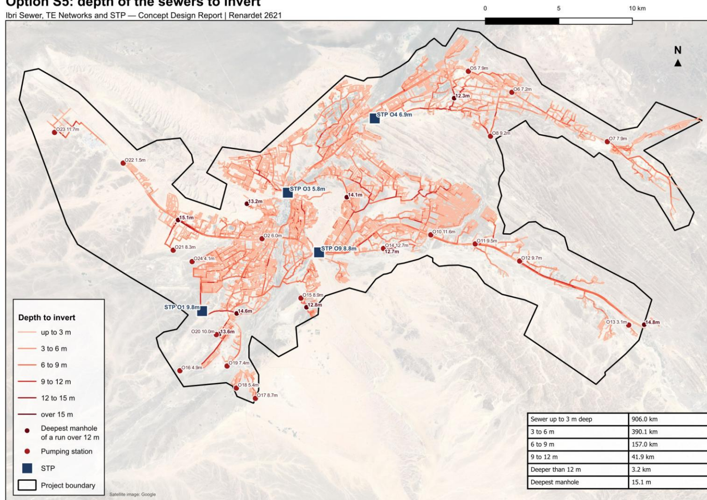
Figure 84. Option S5: depth of the sewers to invert in the 2070 design, the depth of each pumping station's outfall, and the deepest manhole of every run deeper than 12 m.
