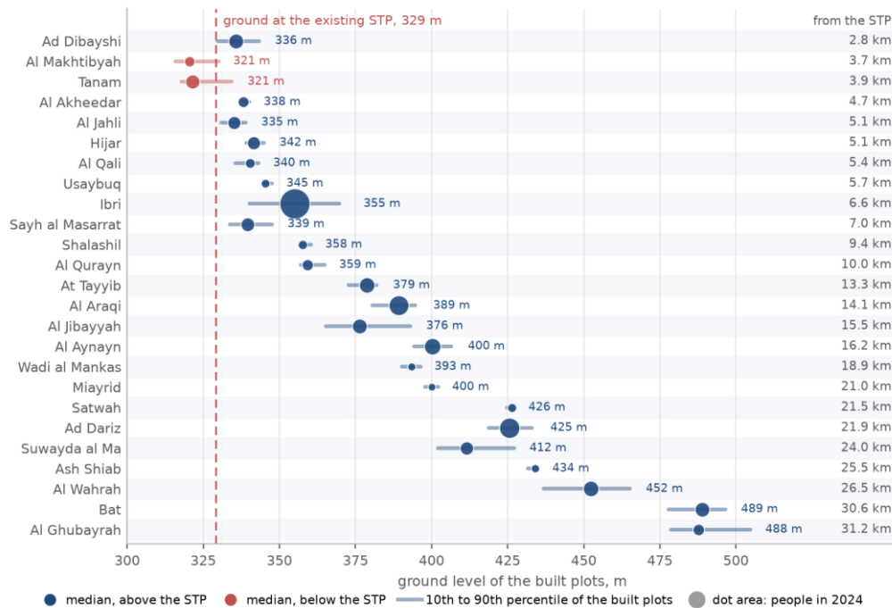
Figure 4. Ground level of the built plots of each settlement, in order of distance from the existing STP. The bar spans the 10th to the 90th percentile of the built plots.
