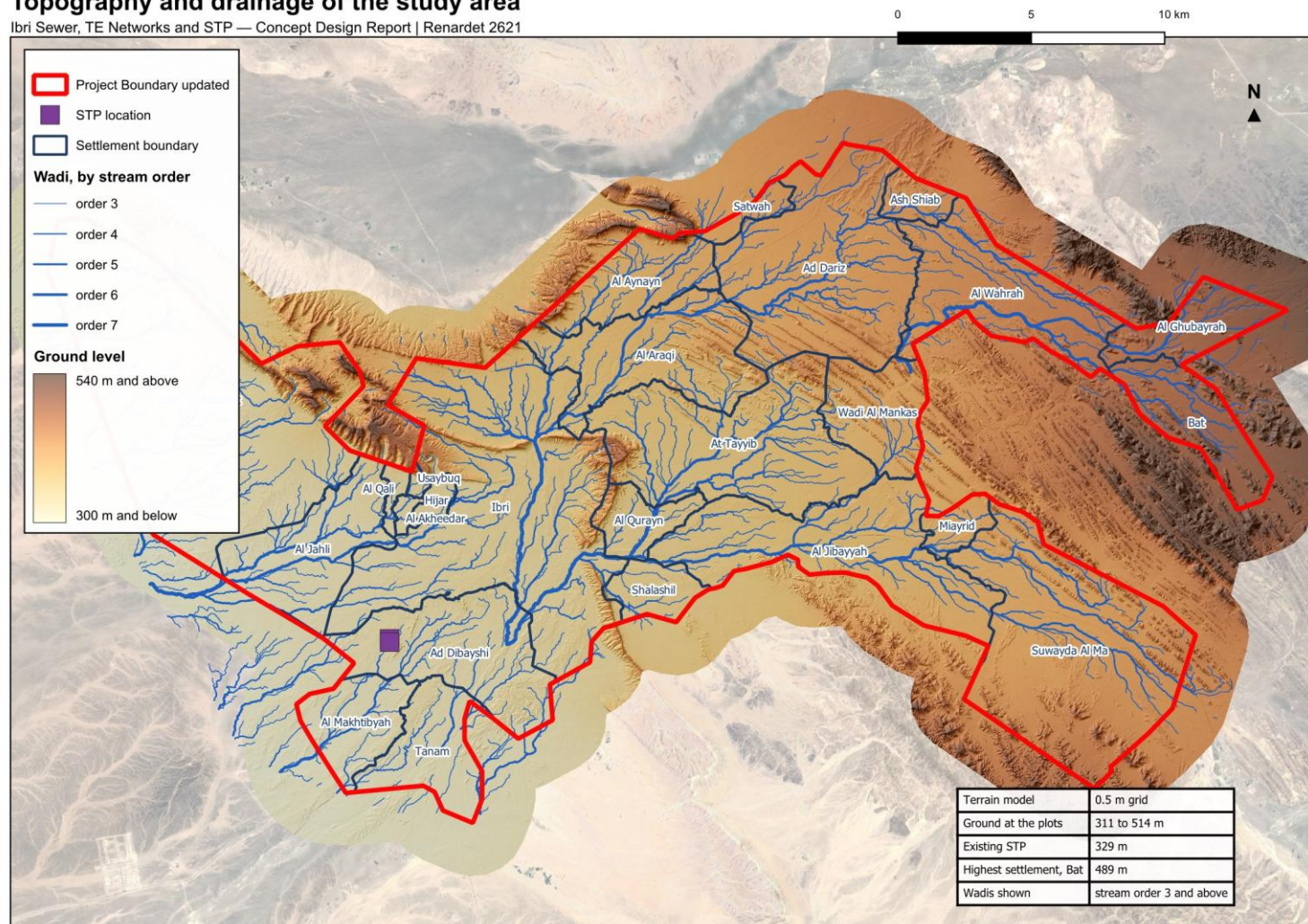
Figure 3. Topography and drainage of the study area: ground level from the 0.5 m terrain model, the wadis of stream order three and above, and the existing STP at the low end of the study area.
