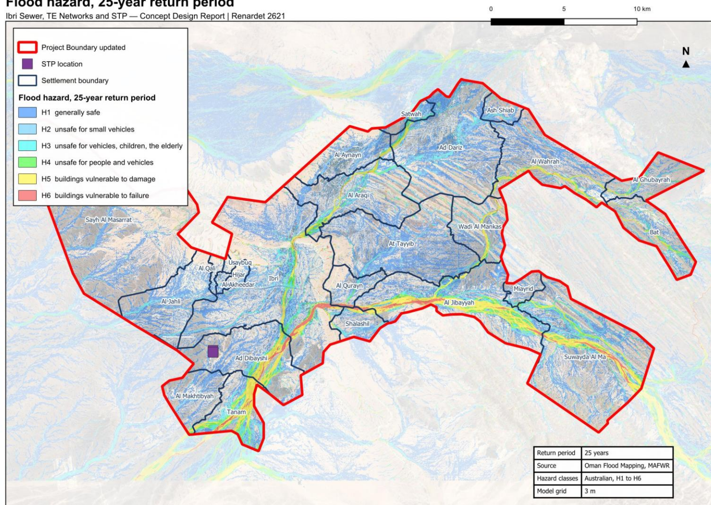
Figure 10. Flood hazard in the study area, 25-year return period. Oman Flood Mapping project, MAFWR; Australian hazard classes.
