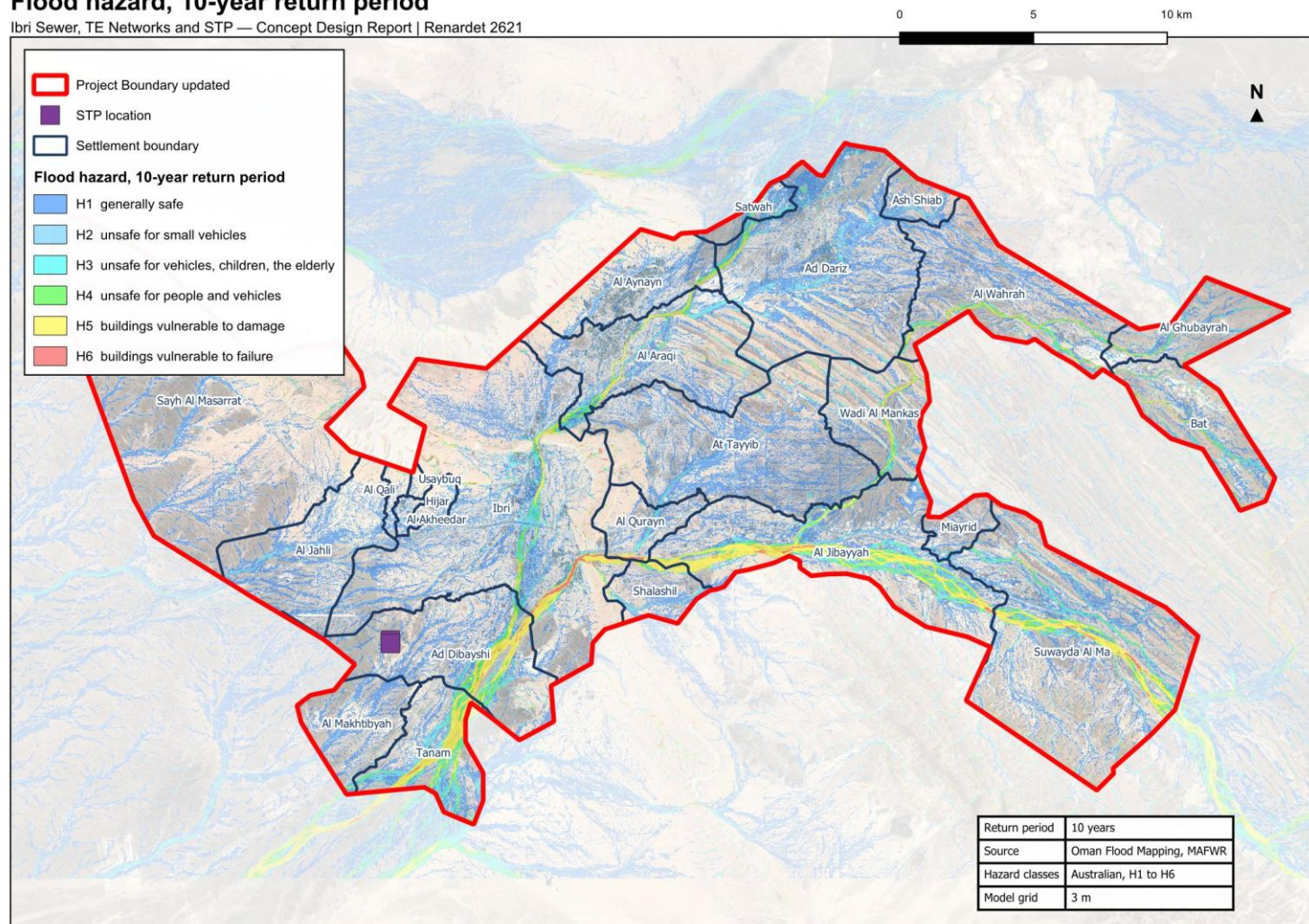
Figure 9. Flood hazard in the study area, 10-year return period. Oman Flood Mapping project, MAFWR; Australian hazard classes.
