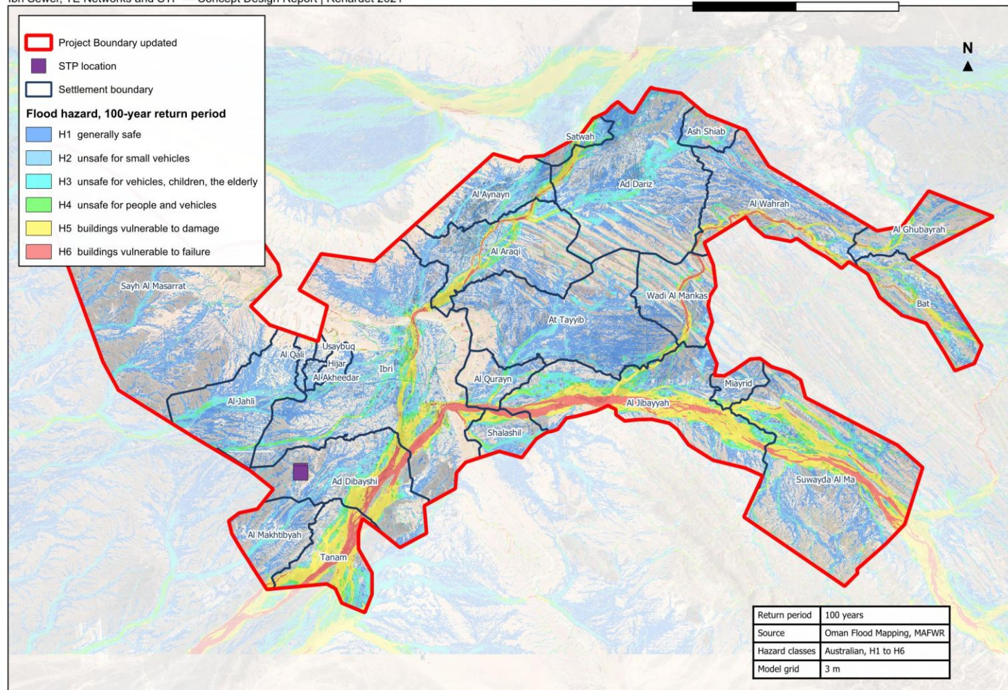
Figure 12. Flood hazard in the study area, 100-year return period. Oman Flood Mapping project, MAFWR; Australian hazard classes.
