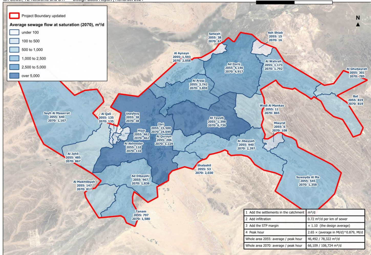
Figure 47. Average sewage flow of each settlement in 2055 and at saturation, and the four steps from the settlements in a catchment to the flow of their STP.
