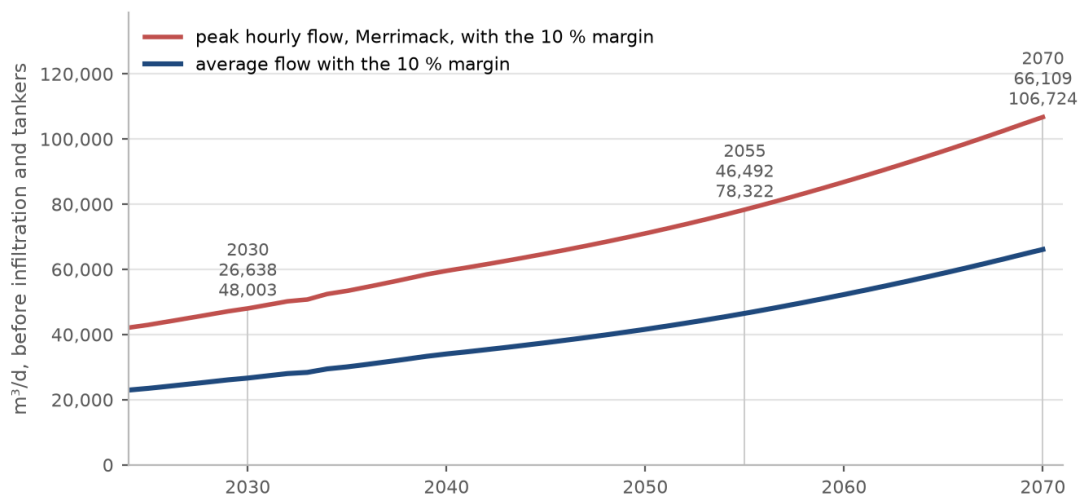
Figure 48. Average and peak-hour flow at one STP for the whole area, by year, with the margin.
