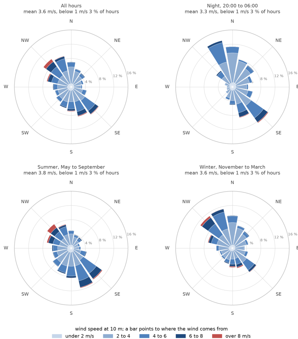
Figure 6. Wind roses at 10 m at the existing STP, 2015 to 2024: the direction the wind blows from and the share of hours in each speed class, for all hours, the night, the summer and the winter.
