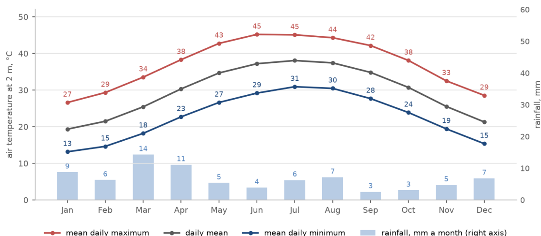
Figure 5. Monthly temperature and rainfall at the existing STP, 2001 to 2020, from the NASA POWER record.
