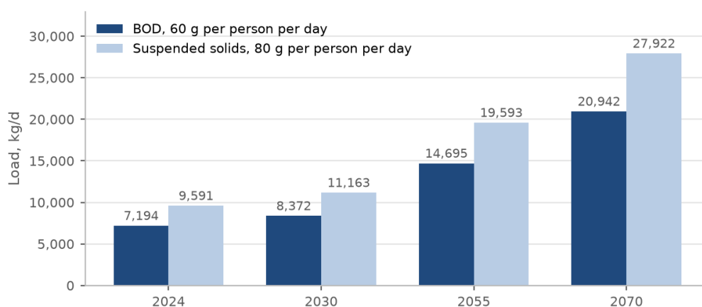
Figure 49. BOD and suspended solids reaching one STP for the whole area, by year, at the guideline's minimum loads per person.
