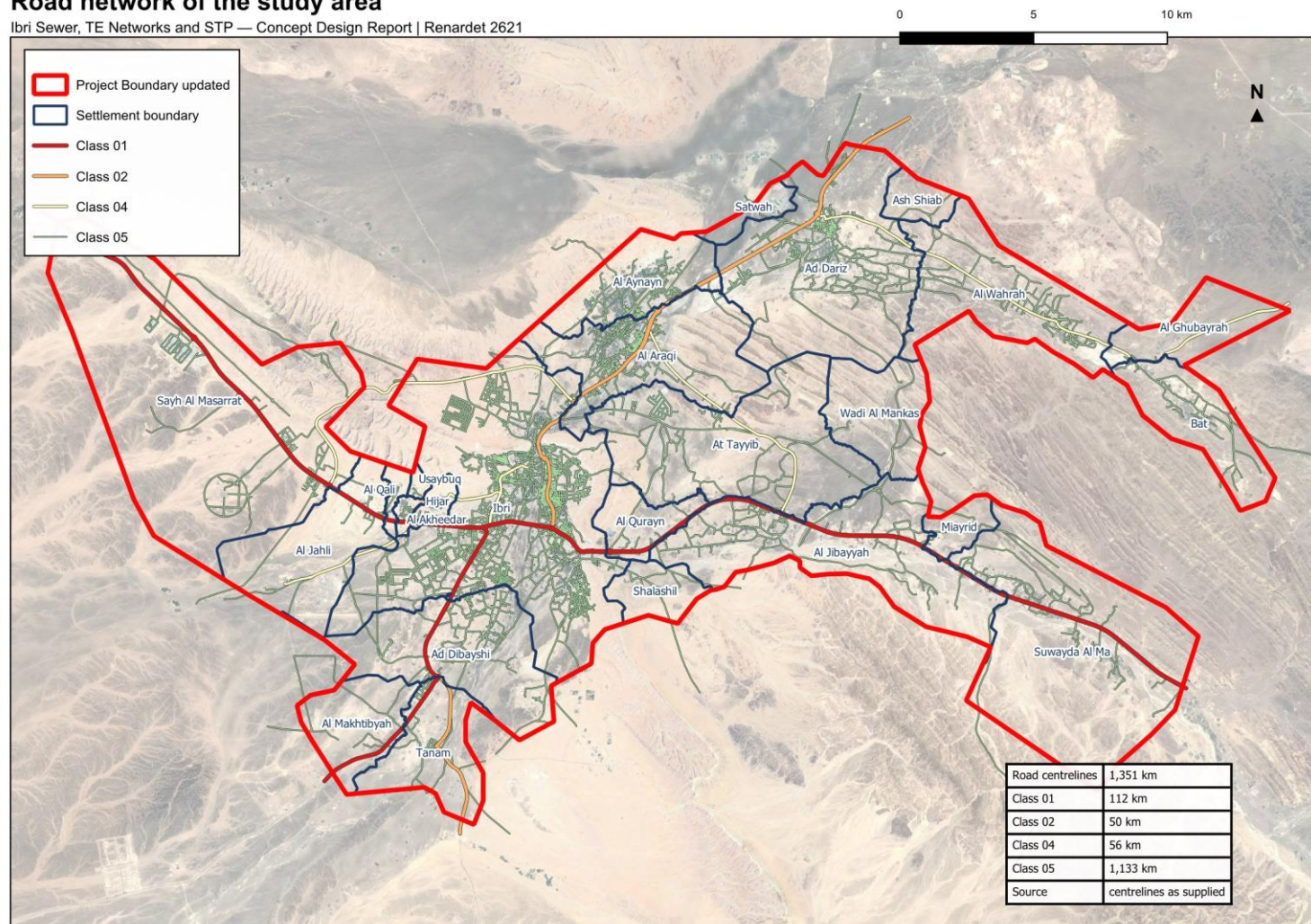
Figure 7. Road network of the study area, by the class code of the centrelines as supplied.
