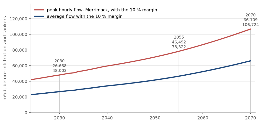
Figure 32 Average and peak-hour flow at one STP for the whole area, by year, with the margin.
