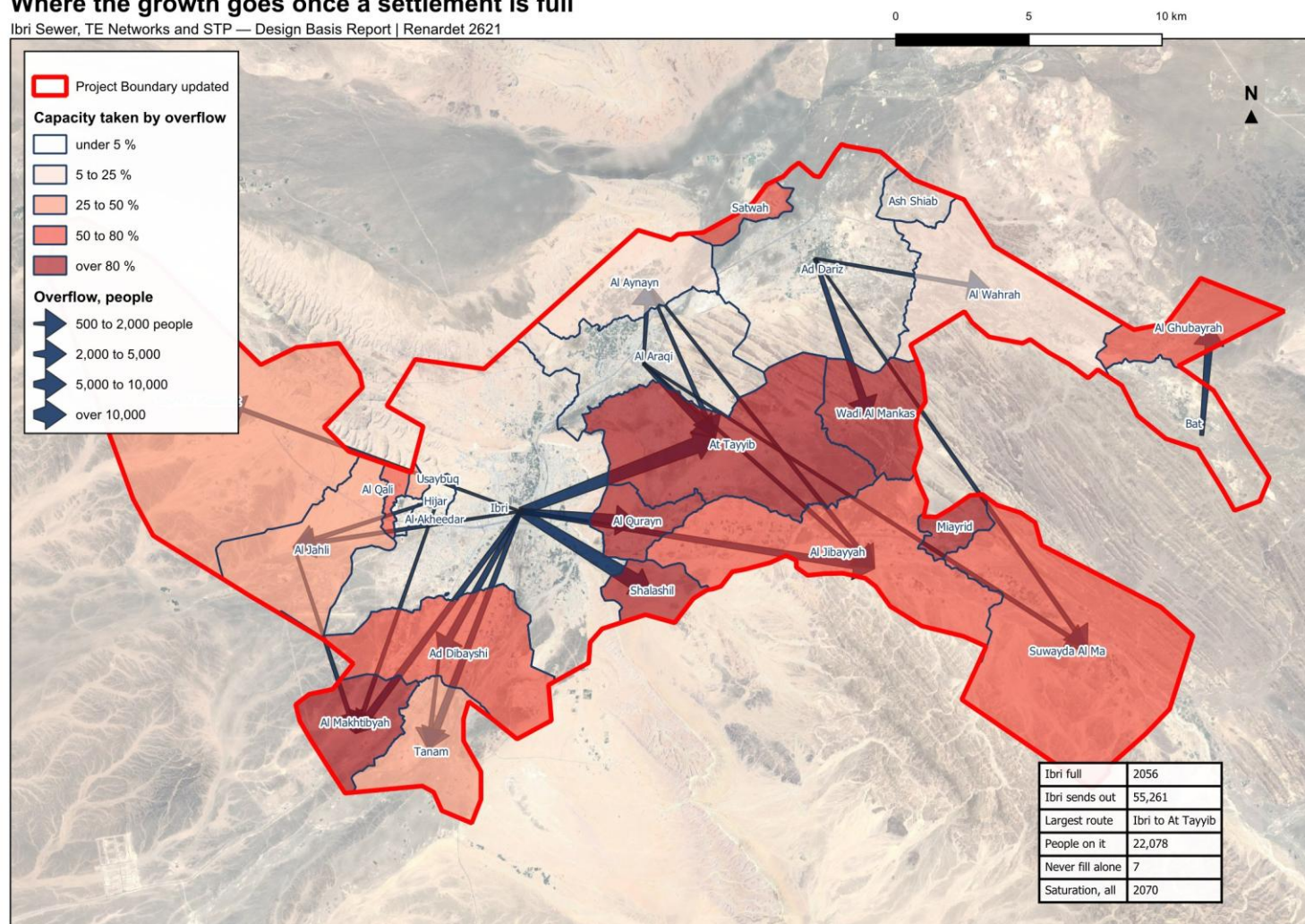
Figure 24 Where the growth goes once a settlement is full. Arrows show the routes carrying five hundred people or more at saturation; the shading shows how much of each settlement's capacity is taken by its neighbours' overflow.
