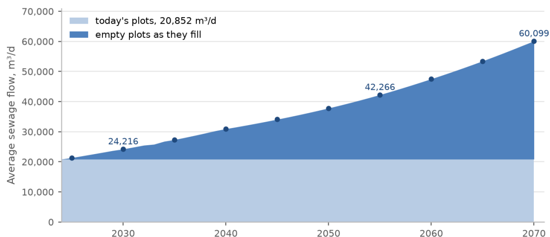
Figure 29 Average sewage flow of the study area by year, from today's plots and from the empty plots as they fill. The points mark the five-year reporting intervals.
