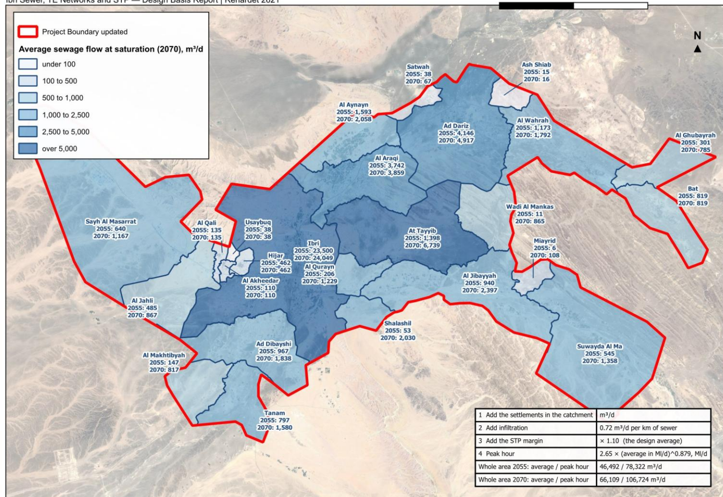
Figure 31 Average sewage flow of each settlement in 2055 and at saturation, and the four steps from the settlements in a catchment to the flow of their STP.
