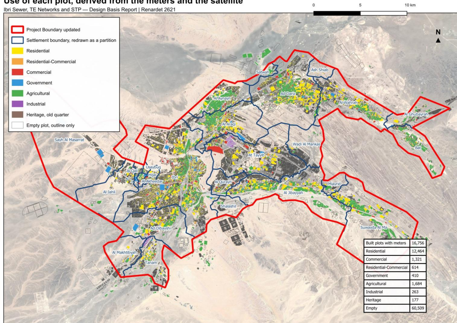
Figure 19 The use of each plot. Coloured plots are built and metered; empty plots are shown by their outline only.
