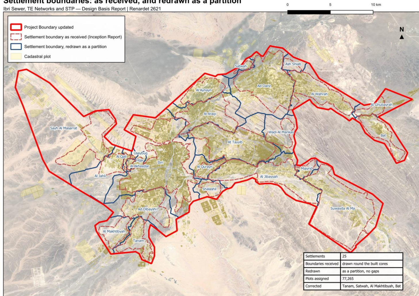
Figure 12 The settlement boundaries as received (red, dashed) and as redrawn for the design (blue). Every plot lies in one settlement and the boundaries meet without gaps.
