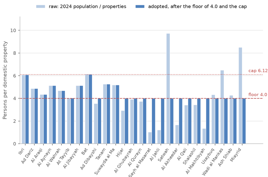
Figure 15 Occupancy rate by settlement: the value calculated from the census and the meters, and the value adopted after the floor and the cap.
