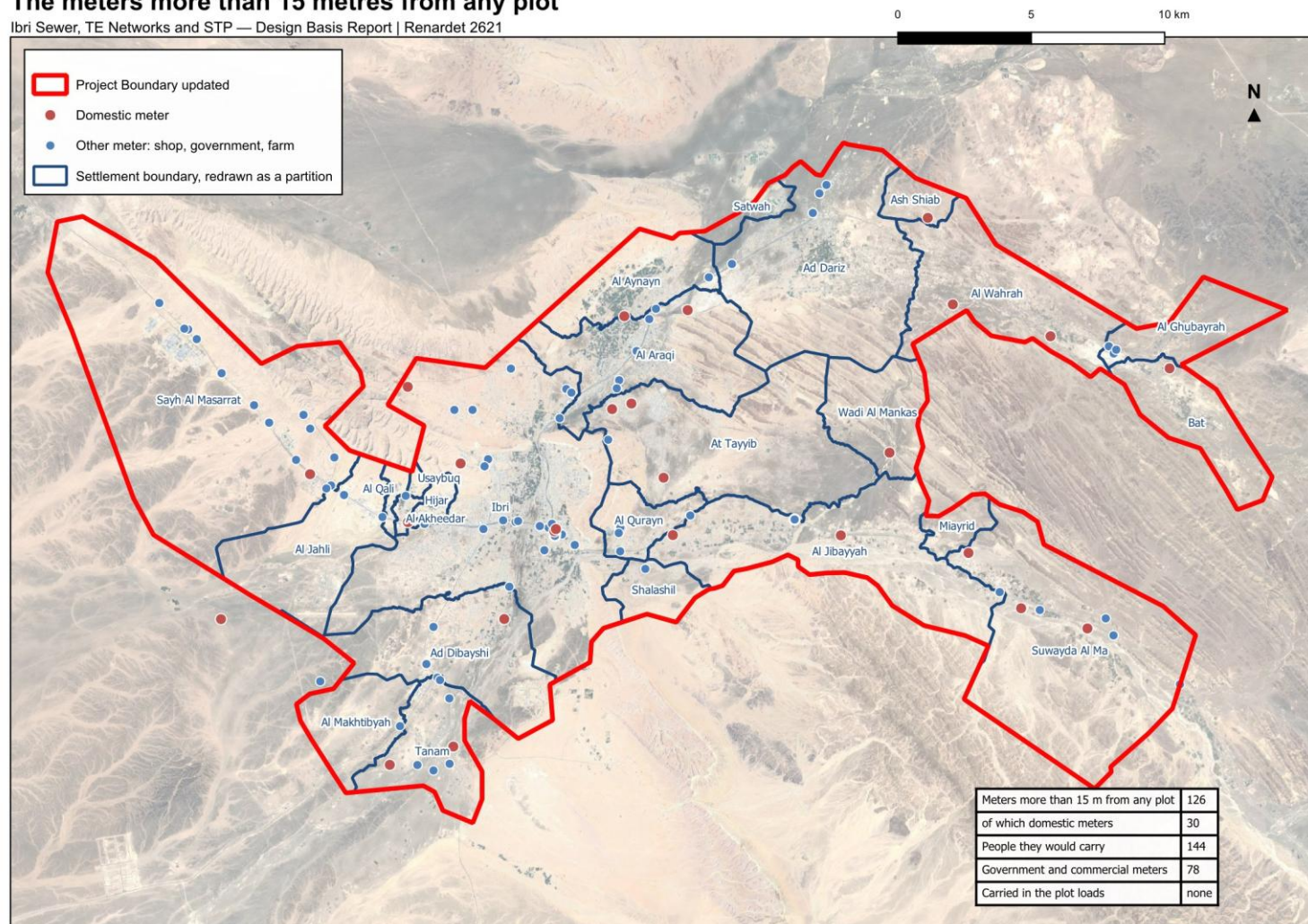
Figure 13 The 126 meters more than fifteen metres from any plot. Red: a domestic meter; blue: any other meter.
