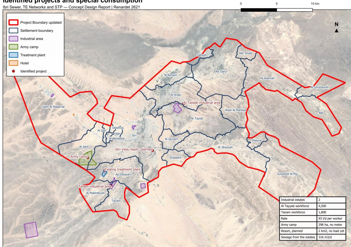
Figure 33 The identified projects and special consumers: the industrial areas, the army camp, the treatment plant and the hotel sites recorded in OpenStreetMap, the two estates among them.
