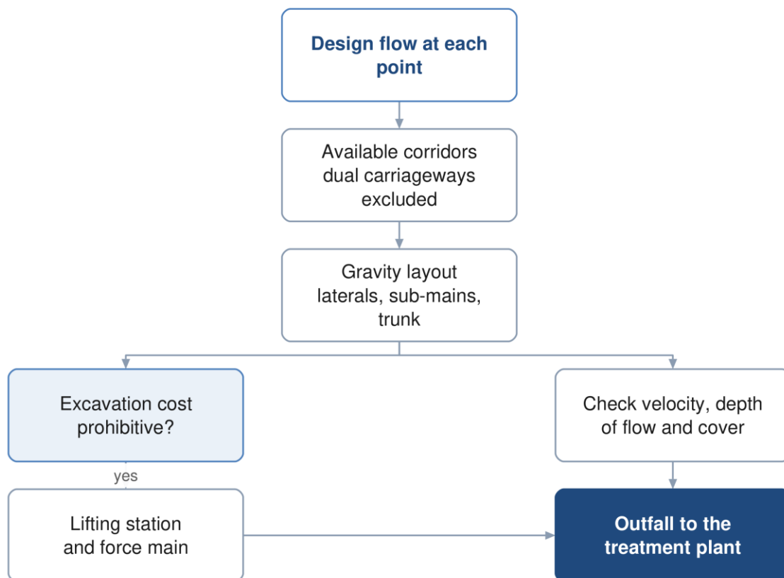
Figure 36 The network design approach, and the point at which a lifting station becomes necessary.
