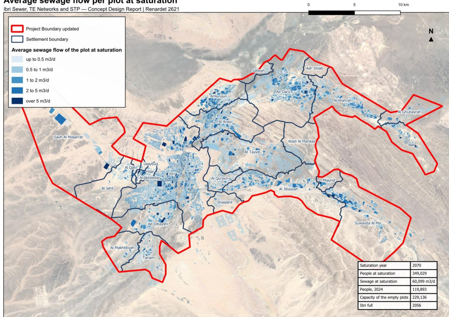
Figure 30 Average sewage flow of every plot at saturation.
