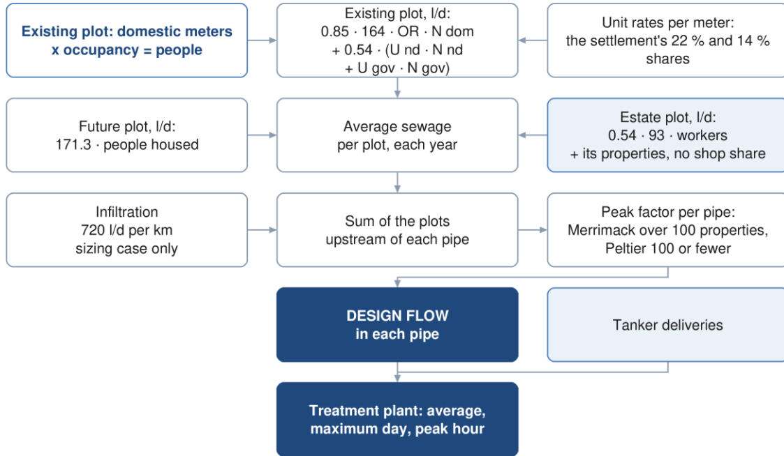
Figure 27 Derivation of the design flow, from the plot to the pipe and the STP.
