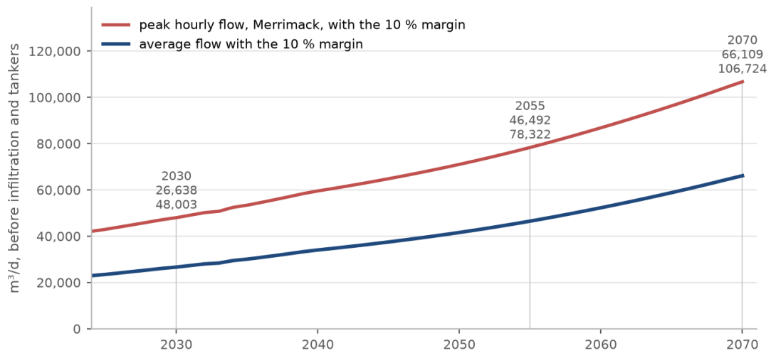
Figure 13 Average and peak-hour flow at one works for the whole area, by year, with the margin.
