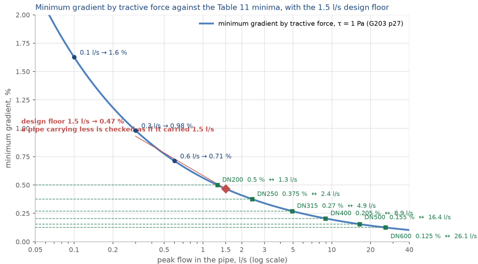
Figure 23 The minimum gradient by tractive force at one pascal, the Table 11 minima of every size, and the proposed 1.5 litres a second floor.
