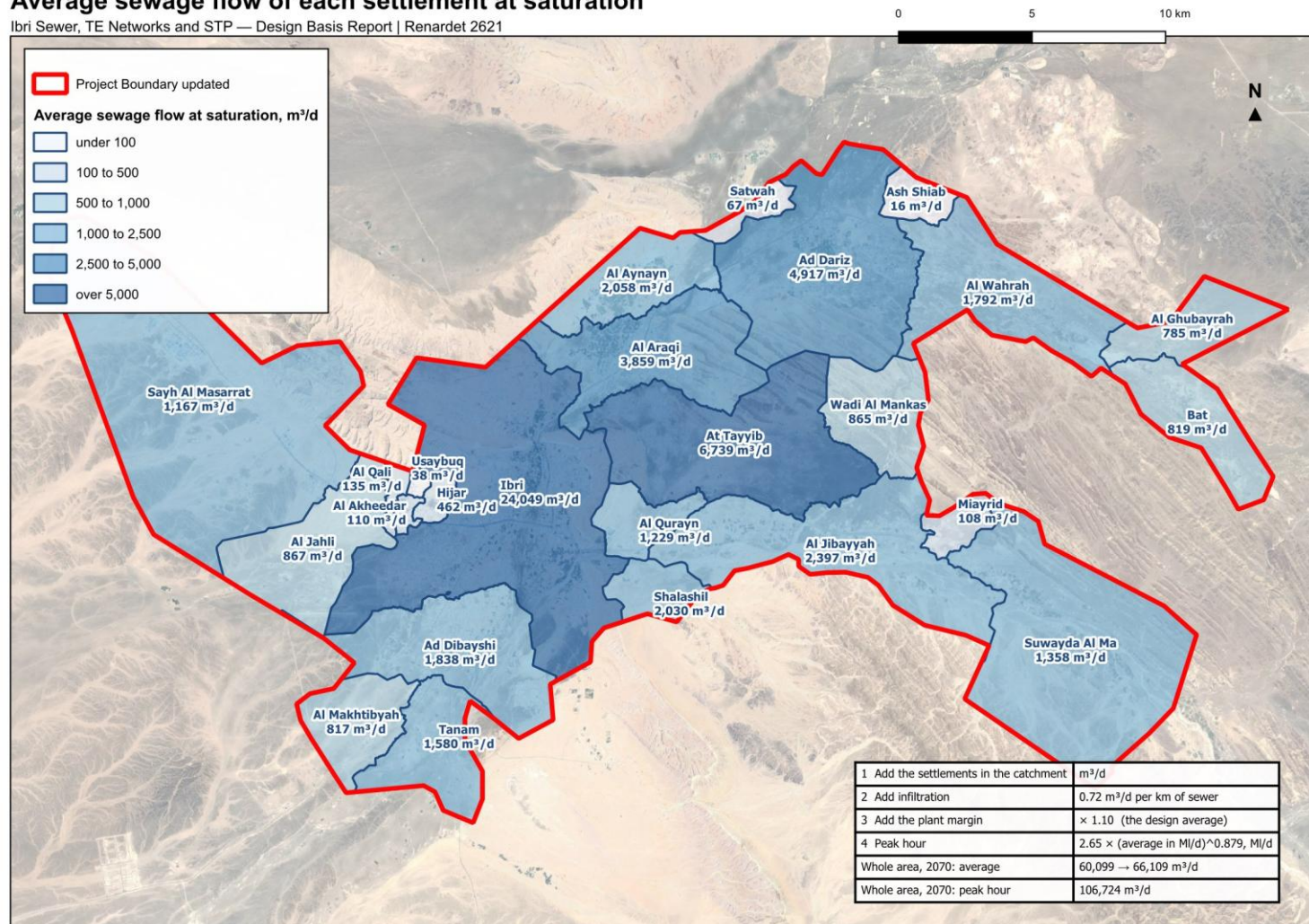
Figure 14 Average sewage flow of each settlement at saturation, and the four steps from the settlements in a catchment to the flow of its plant.
