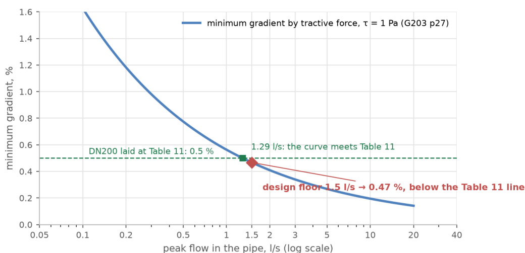
Figure 12 The minimum gradient the tractive-force test asks for, against the flow in the pipe, with the 200 mm line and the proposed 1.5 litres a second floor.
