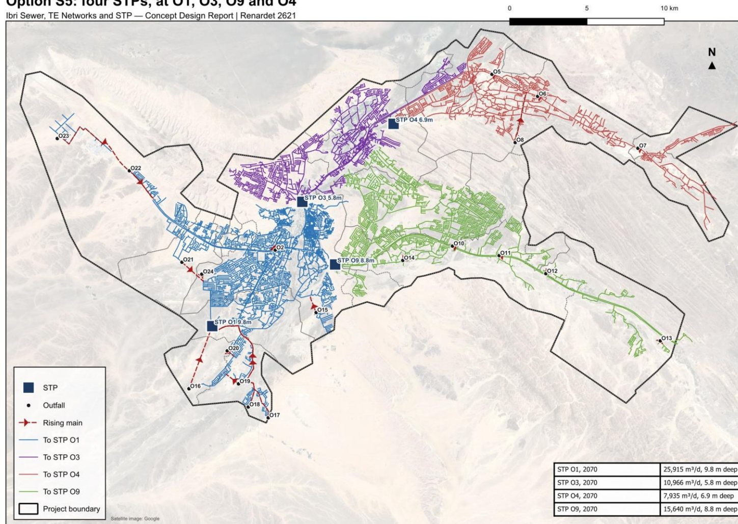
Figure 70. Option S5: the sewers by the plant they drain to, the outfalls, and the depth of the sewer arriving at each plant.
