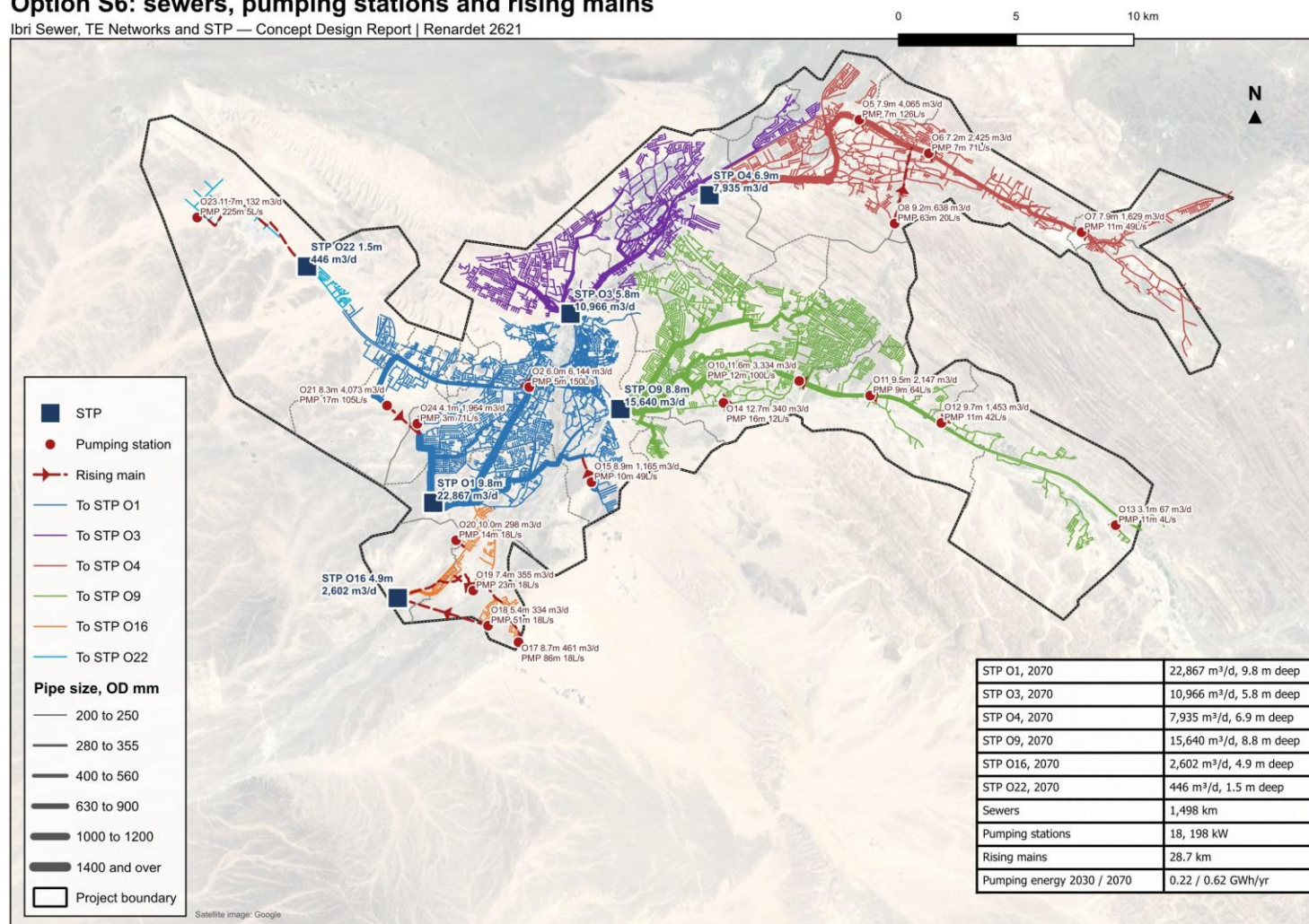
Figure 74. Option S6: the sewers by plant and size, the pumping stations and the rising mains. A station label gives the outfall, its depth and the average flow in 2070, then the pump head and the duty.
