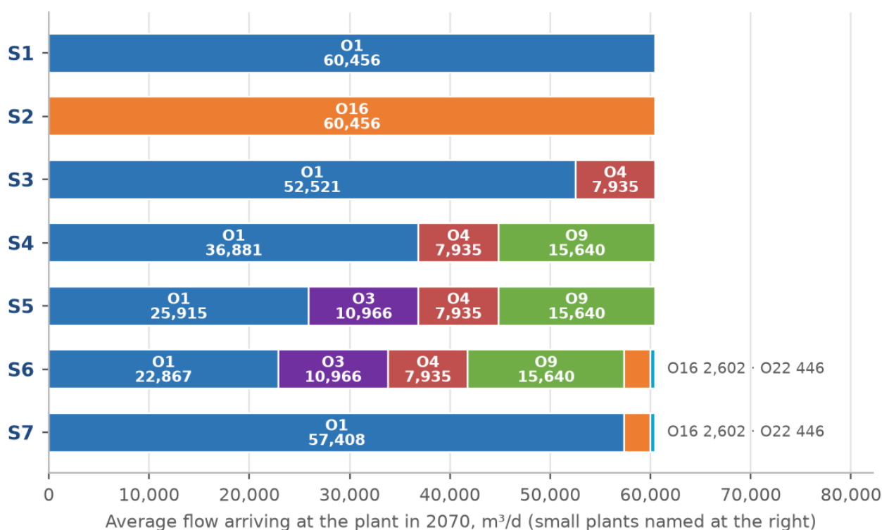
Figure 78. The average flow arriving at each plant in 2070, by option. Colours as on the maps and diagrams.
