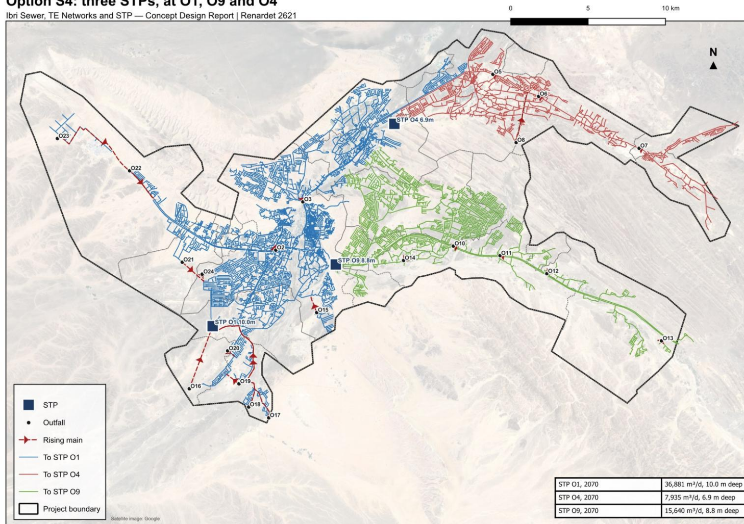
Figure 67. Option S4: the sewers by the plant they drain to, the outfalls, and the depth of the sewer arriving at each plant.
