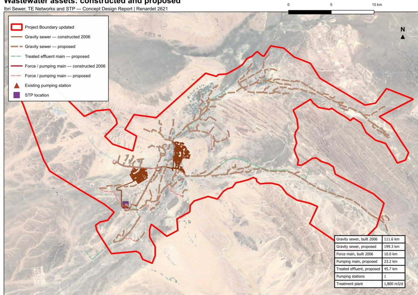
Figure 17. Wastewater assets within the study area. The constructed network, dated 2006, is shown distinctly from the alignments recorded in the dataset as proposed.
