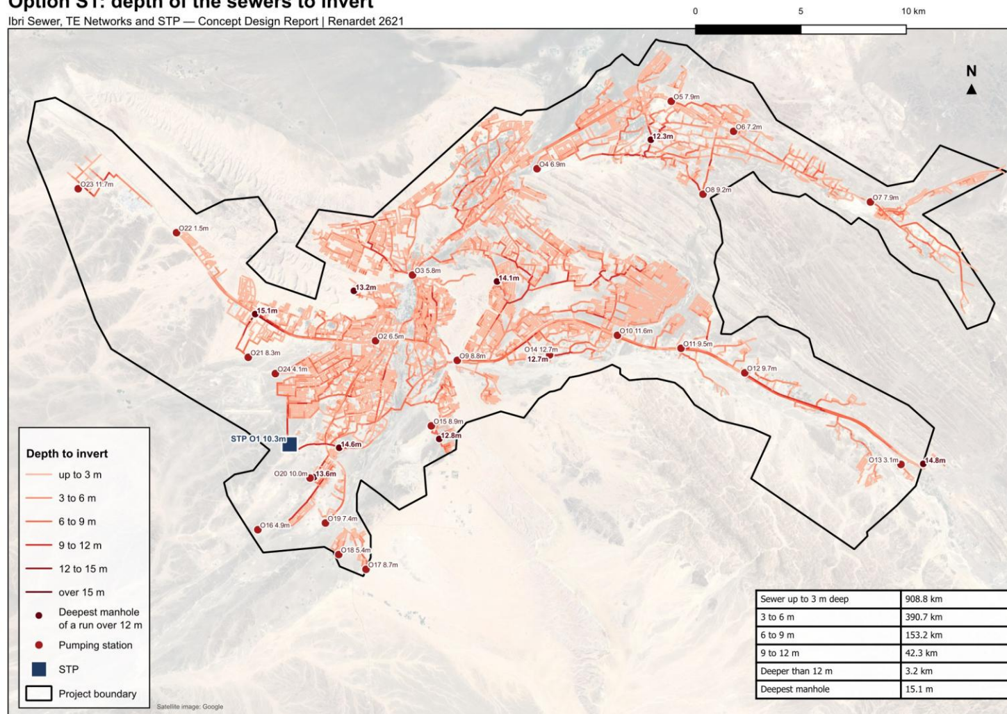
Figure 82. Option S1: depth of the sewers to invert in the 2070 design, the depth of each pumping station's outfall, and the deepest manhole of every run deeper than 12 m.
