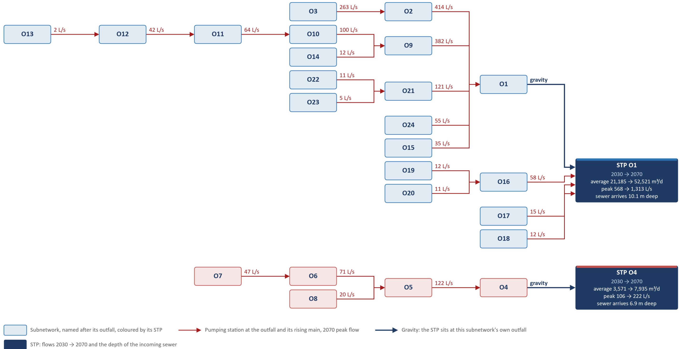
Figure 63. Option S3, two STPs, at O1 and O4: where the flow of every subnetwork goes, with the peak flow of each transfer in 2070.
