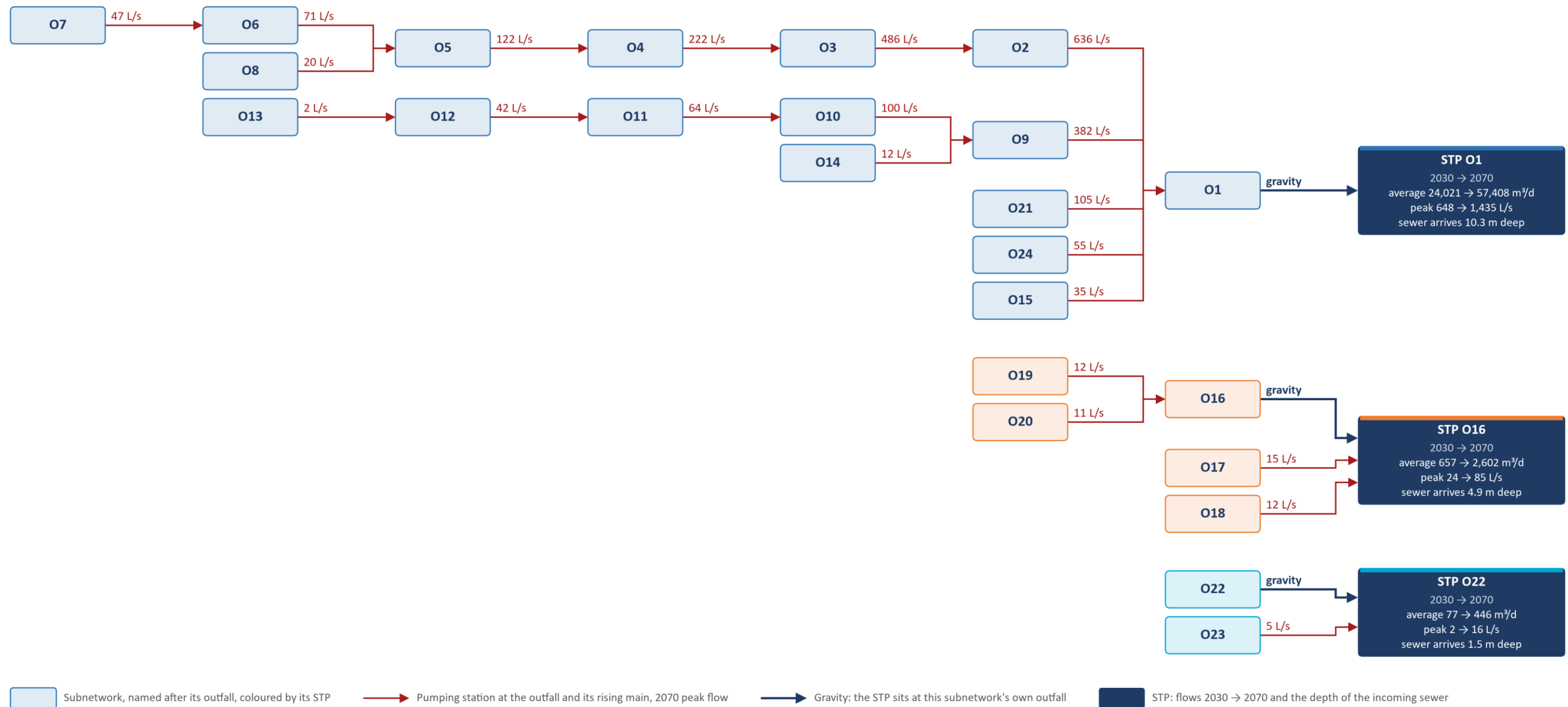
Figure 75. Option S7, three STPs, at O1, O16 and O22: where the flow of every subnetwork goes, with the peak flow of each transfer in 2070.
