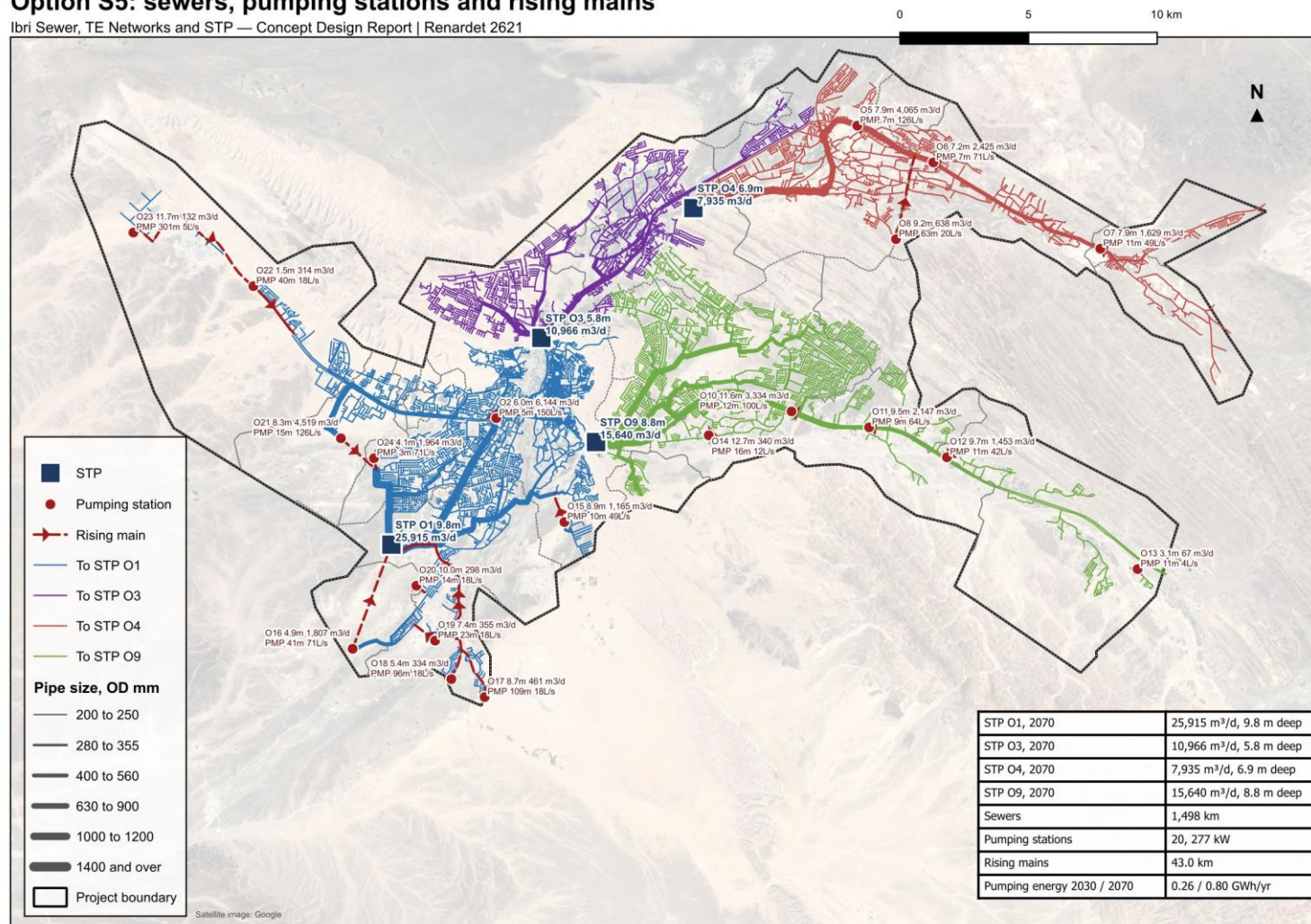
Figure 71. Option S5: the sewers by plant and size, the pumping stations and the rising mains. A station label gives the outfall, its depth and the average flow in 2070, then the pump head and the duty.
