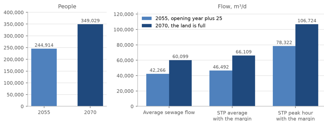
Figure 40. The two horizons side by side: people, average sewage flow, and the STP's average and peak-hour flow with the margin.
