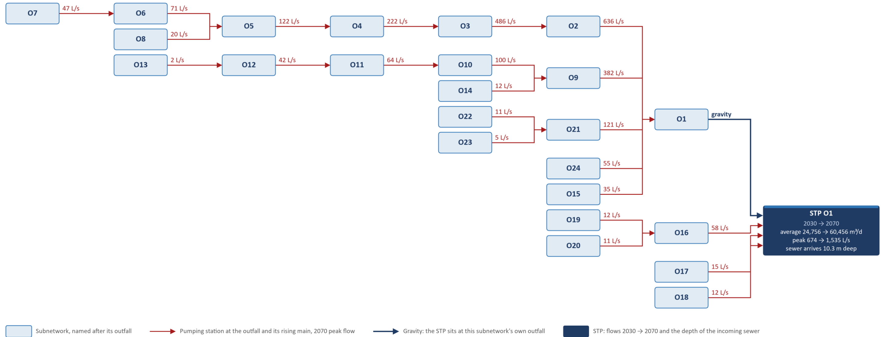
Figure 57. Option S1, one STP for the whole area, at O1: where the flow of every subnetwork goes, with the peak flow of each transfer in 2070.
