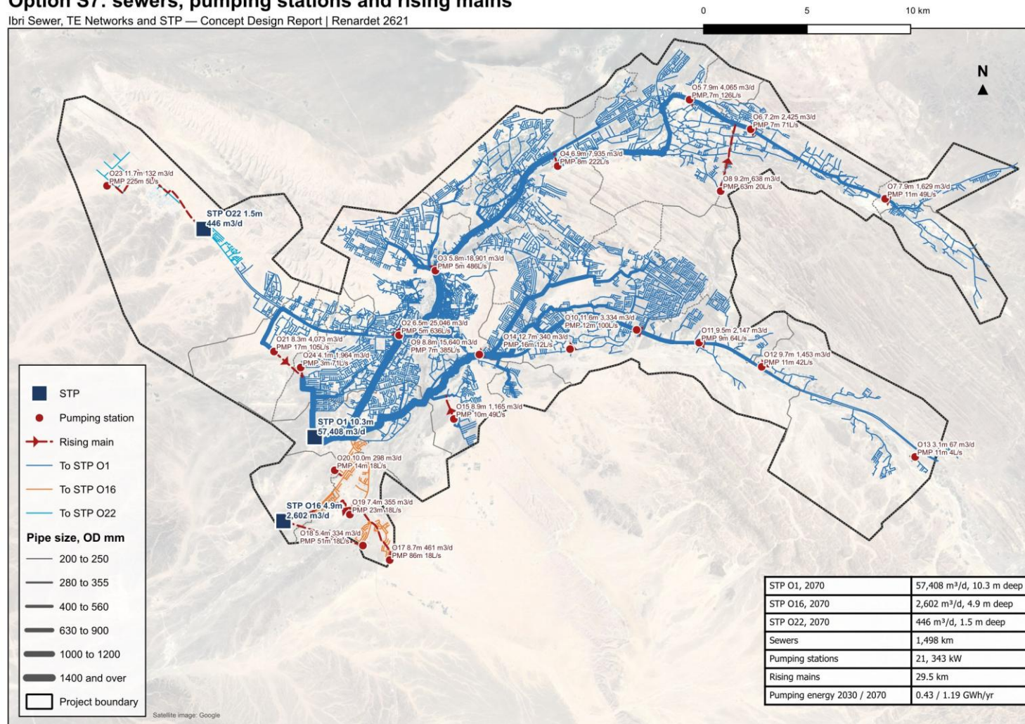
Figure 77. Option S7: the sewers by plant and size, the pumping stations and the rising mains. A station label gives the outfall, its depth and the average flow in 2070, then the pump head and the duty.
