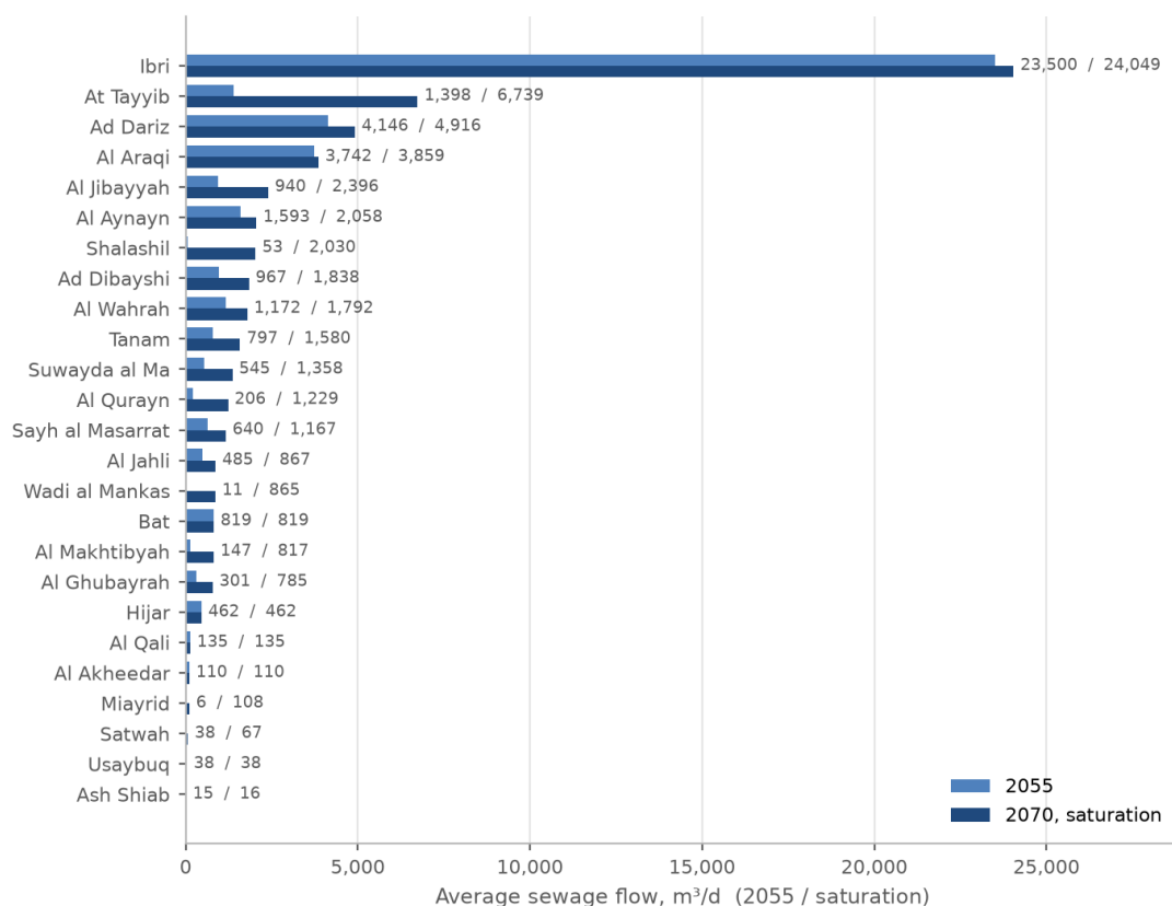
Figure 46. Average sewage flow of every settlement in 2055 and at saturation. Ibri is full before 2055; the growth after it lands on its neighbours.
