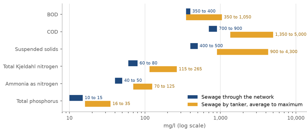
Figure 23. The strength of raw sewage the guideline gives: through the network, and by tanker. The tanker ranges run from the average to the maximum.
