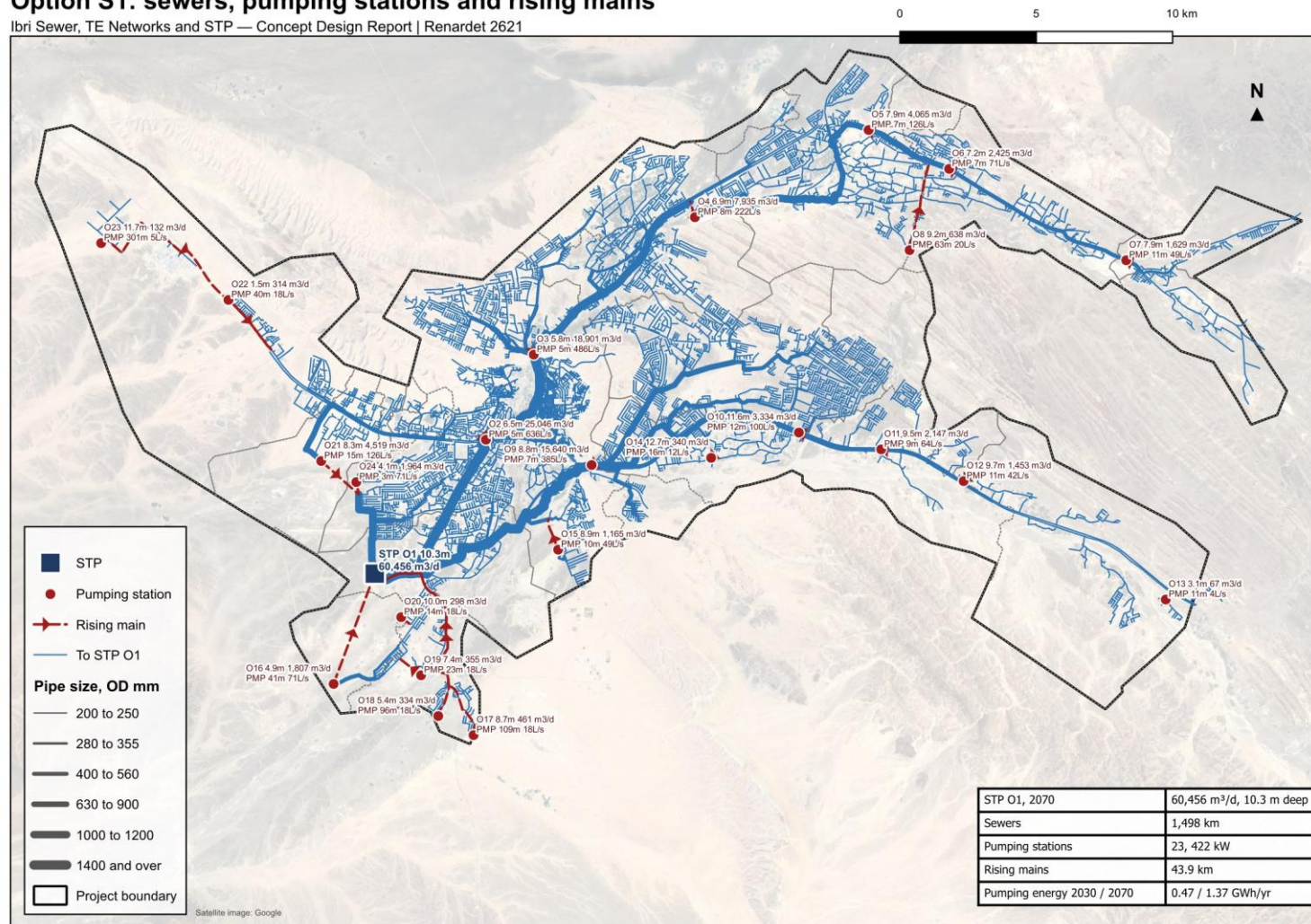
Figure 59. Option S1: the sewers by plant and size, the pumping stations and the rising mains. A station label gives the outfall, its depth and the average flow in 2070, then the pump head and the duty.
