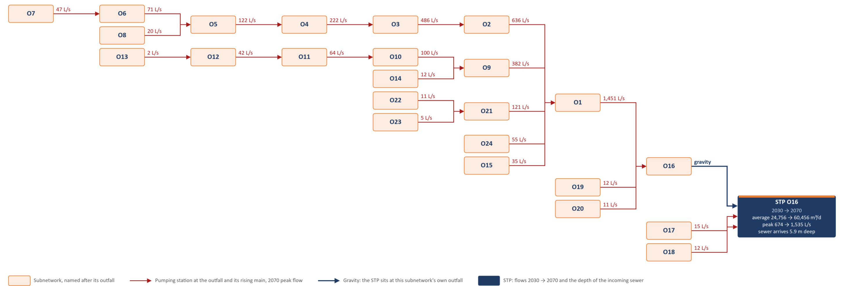
Figure 60. Option S2, one STP for the whole area, at O16: where the flow of every subnetwork goes, with the peak flow of each transfer in 2070.
