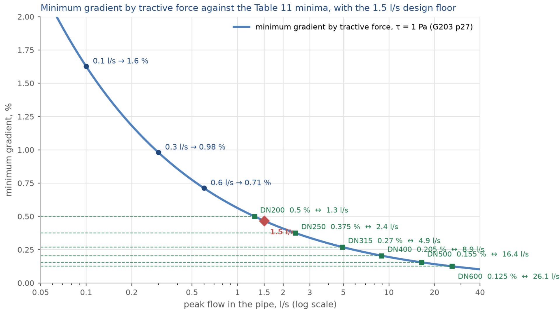
Figure 22. The minimum gradient by tractive force at one pascal against the flow in the pipe, with the Table 11 minimum of every size marked where it meets the curve, and the 1.5 l/s floor.
