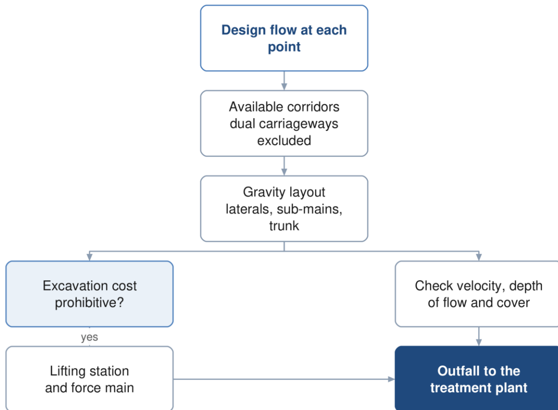
Figure 55. The network design approach, and the point at which a lifting station becomes necessary.
