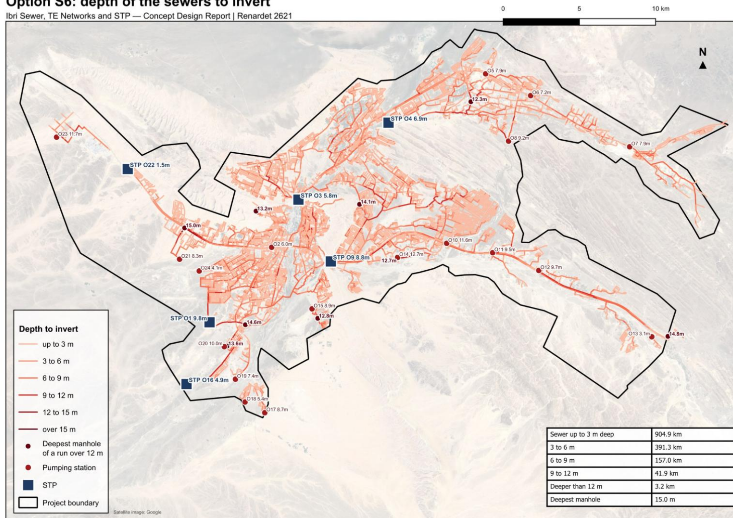
Figure 87. Option S6: depth of the sewers to invert in the 2070 design, the depth of each pumping station's outfall, and the deepest manhole of every run deeper than 12 m.
