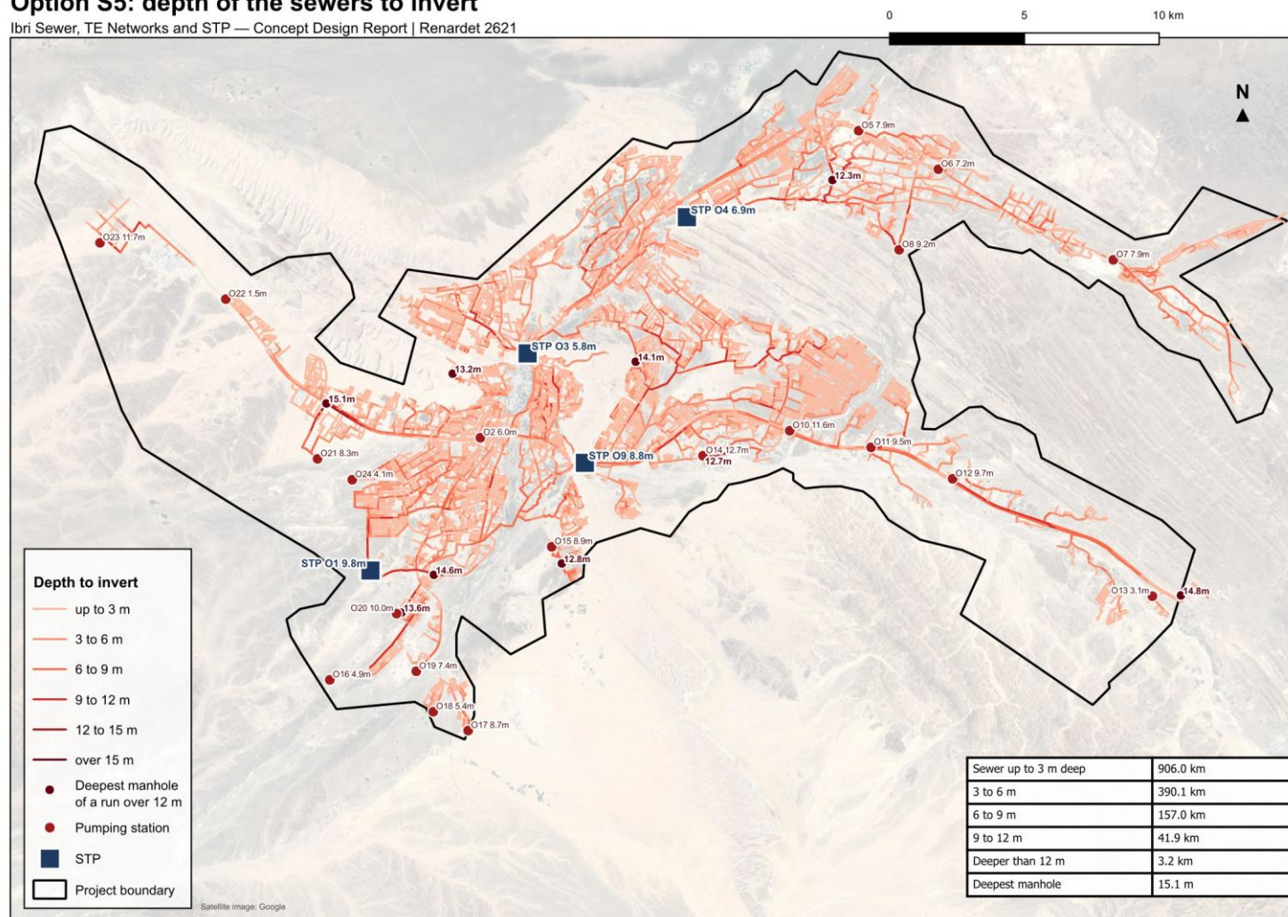
Figure 86. Option S5: depth of the sewers to invert in the 2070 design, the depth of each pumping station's outfall, and the deepest manhole of every run deeper than 12 m.
