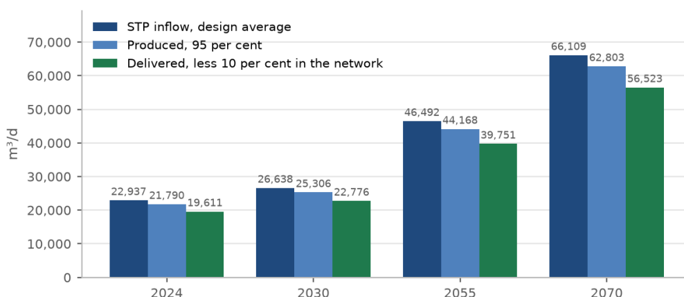
Figure 52. STP inflow, treated effluent produced and treated effluent delivered to customers, by year.
