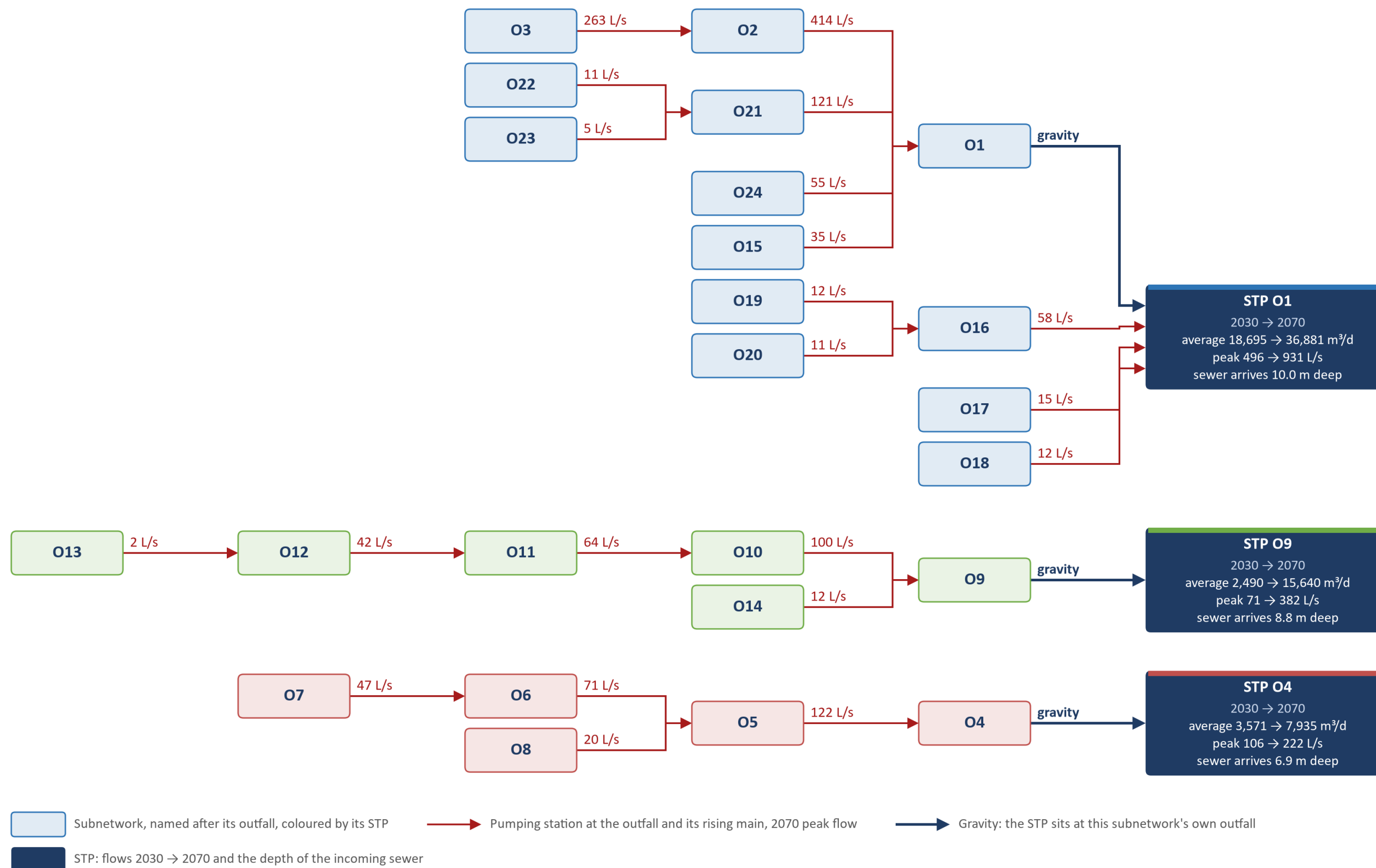
Figure 66. Option S4, three STPs, at O1, O9 and O4: where the flow of every subnetwork goes, with the peak flow of each transfer in 2070.
