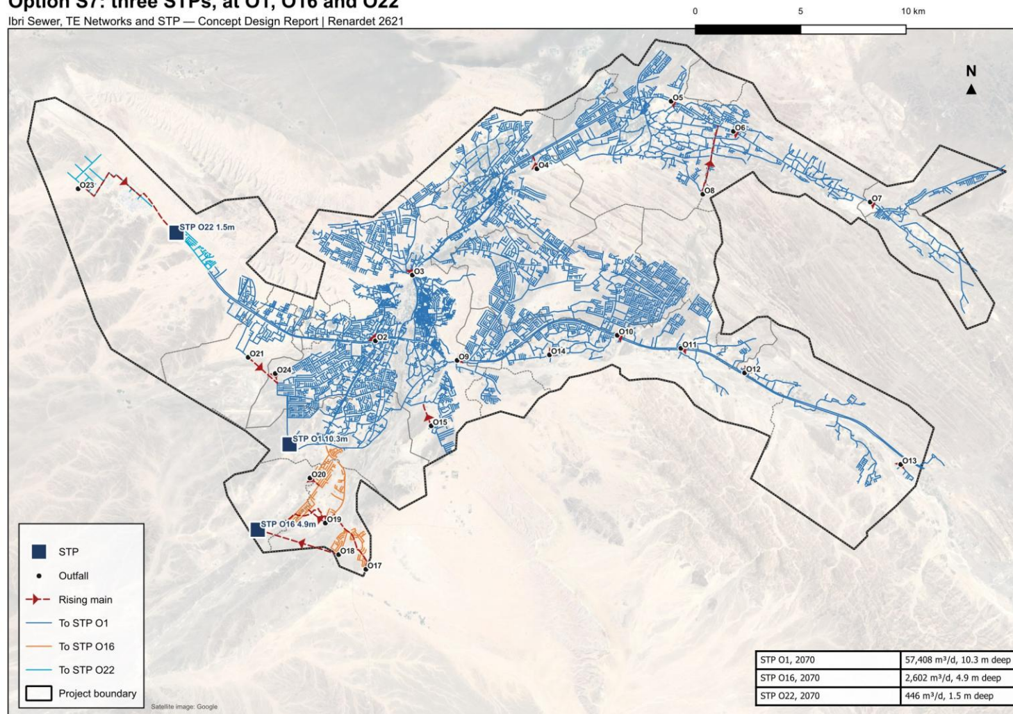
Figure 76. Option S7: the sewers by the plant they drain to, the outfalls, and the depth of the sewer arriving at each plant.
