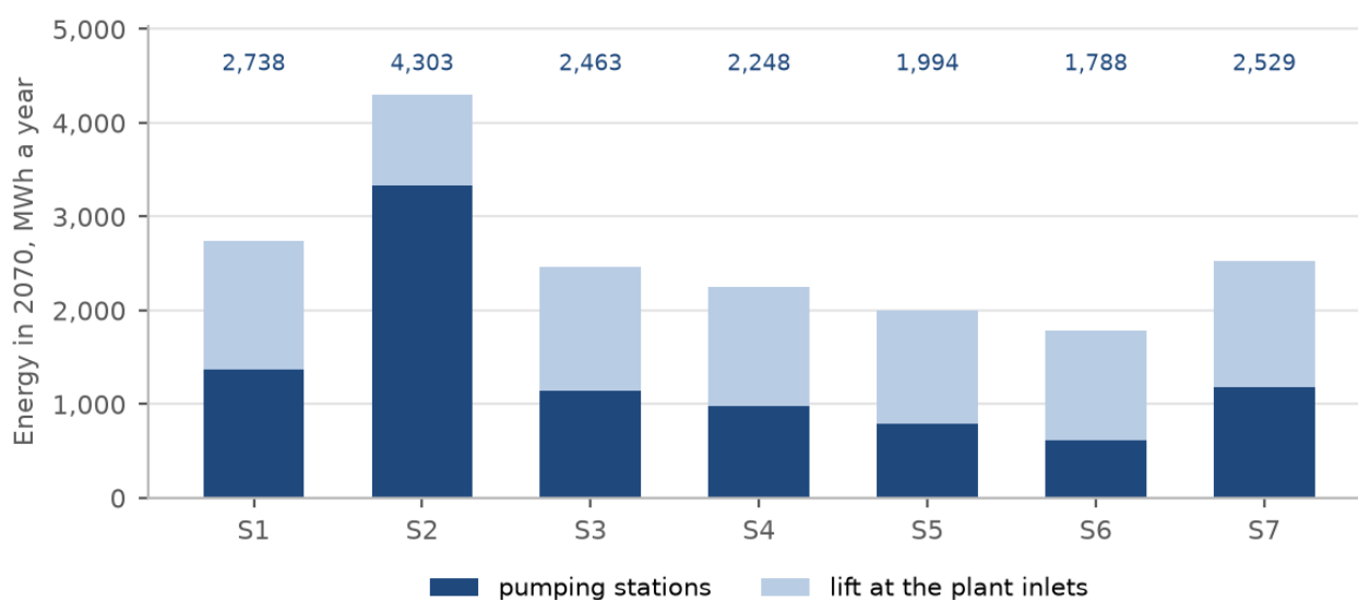
Figure 81. Pumping energy in 2070 by option: the network's pumping stations and the lift at the plant inlets.
