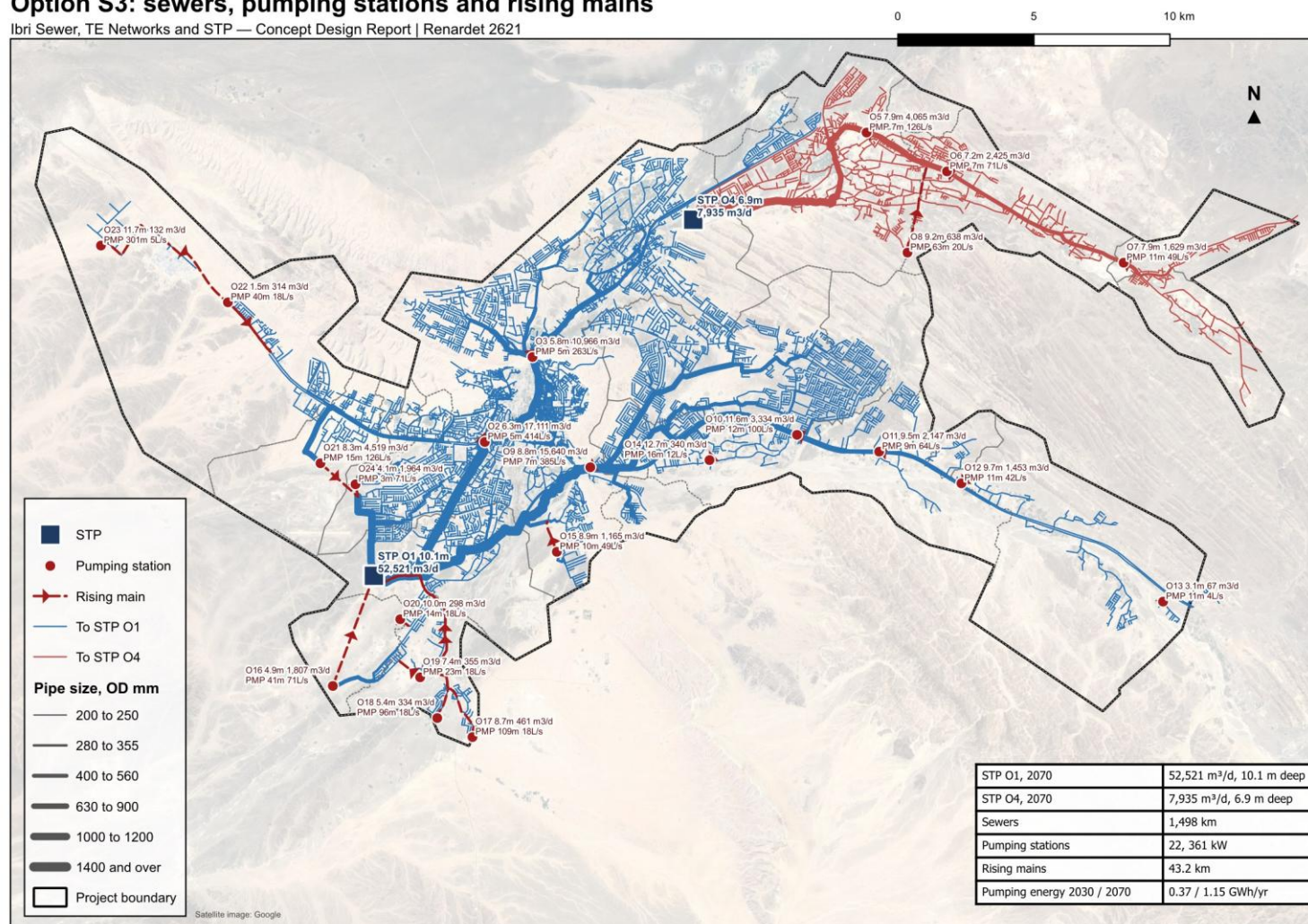
Figure 65. Option S3: the sewers by plant and size, the pumping stations and the rising mains. A station label gives the outfall, its depth and the average flow in 2070, then the pump head and the duty.
