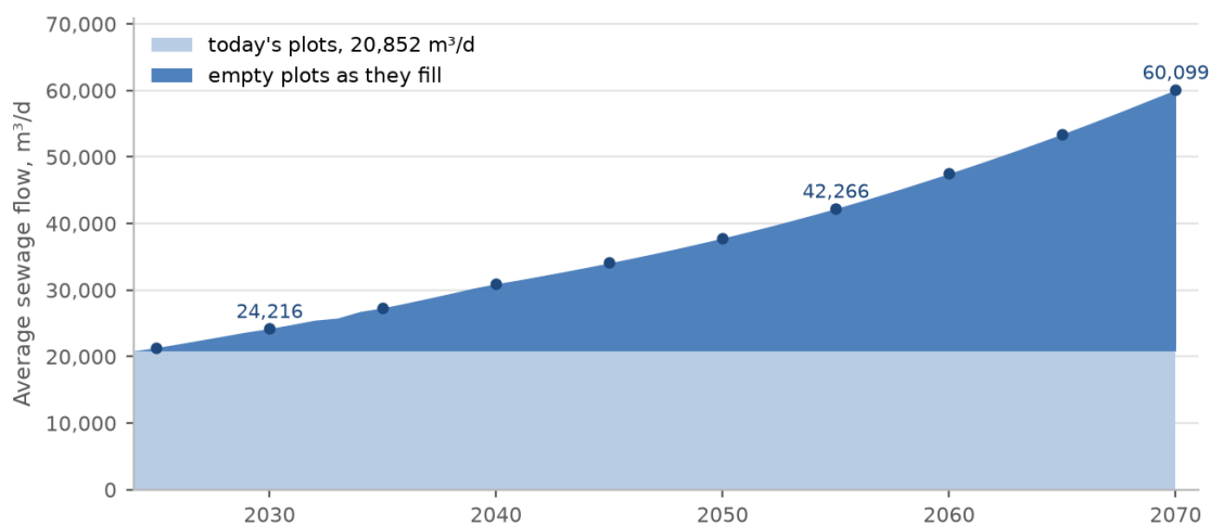
Figure 45. Average sewage flow of the study area by year, from today's plots and from the empty plots as they fill. The points mark the five-year reporting intervals.
