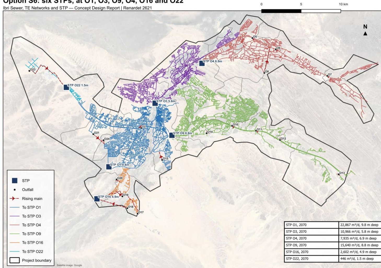
Figure 73. Option S6: the sewers by the plant they drain to, the outfalls, and the depth of the sewer arriving at each plant.
