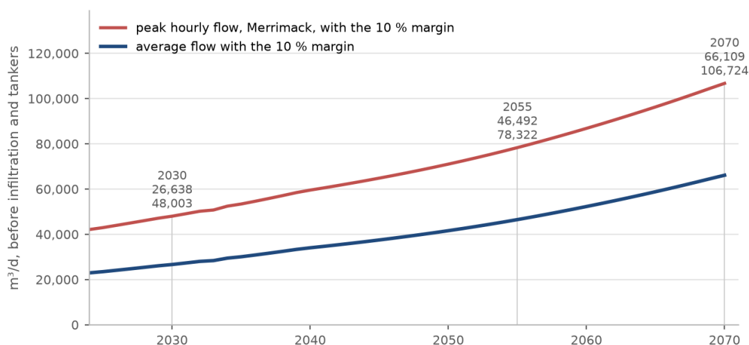
Figure 49. Average and peak-hour flow at one STP for the whole area, by year, with the margin.
