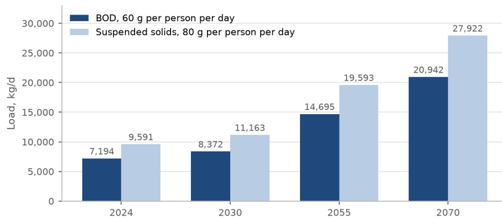
Figure 50. BOD and suspended solids reaching one STP for the whole area, by year, at the guideline's minimum loads per person.
