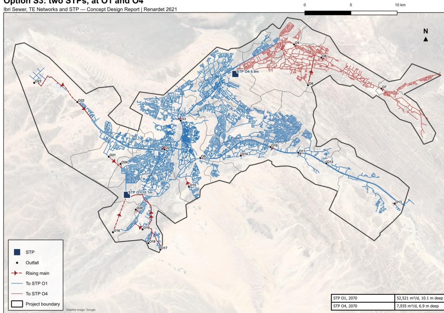
Figure 64. Option S3: the sewers by the plant they drain to, the outfalls, and the depth of the sewer arriving at each plant.
