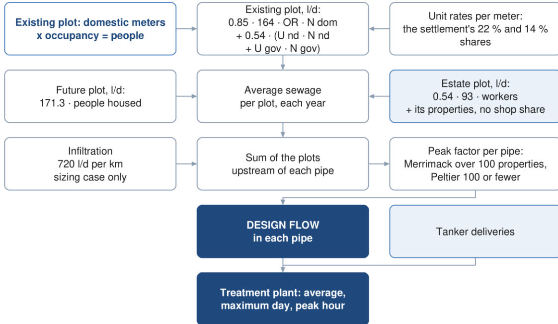
Figure 42. Derivation of the design flow, from the plot to the pipe and the STP.
