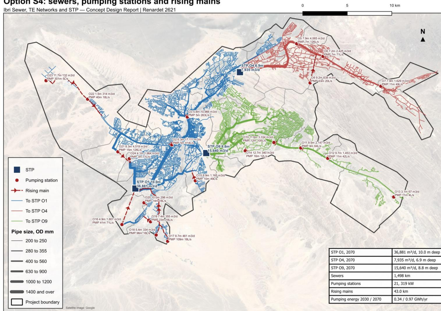
Figure 68. Option S4: the sewers by plant and size, the pumping stations and the rising mains. A station label gives the outfall, its depth and the average flow in 2070, then the pump head and the duty.
