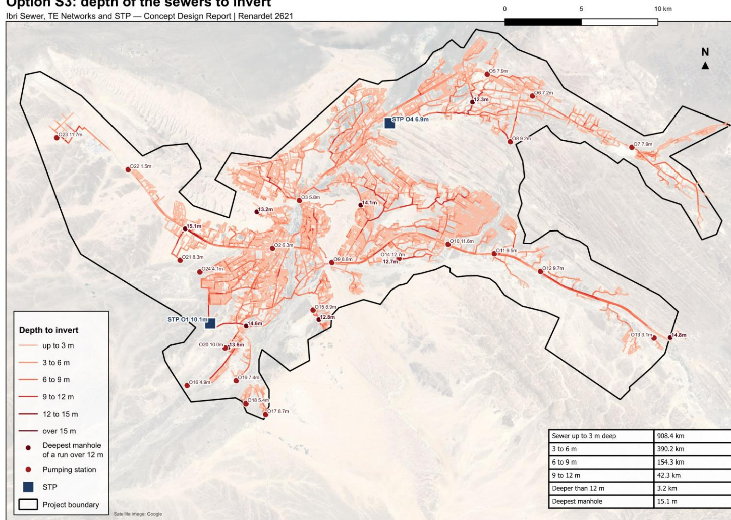
Figure 84. Option S3: depth of the sewers to invert in the 2070 design, the depth of each pumping station's outfall, and the deepest manhole of every run deeper than 12 m.
