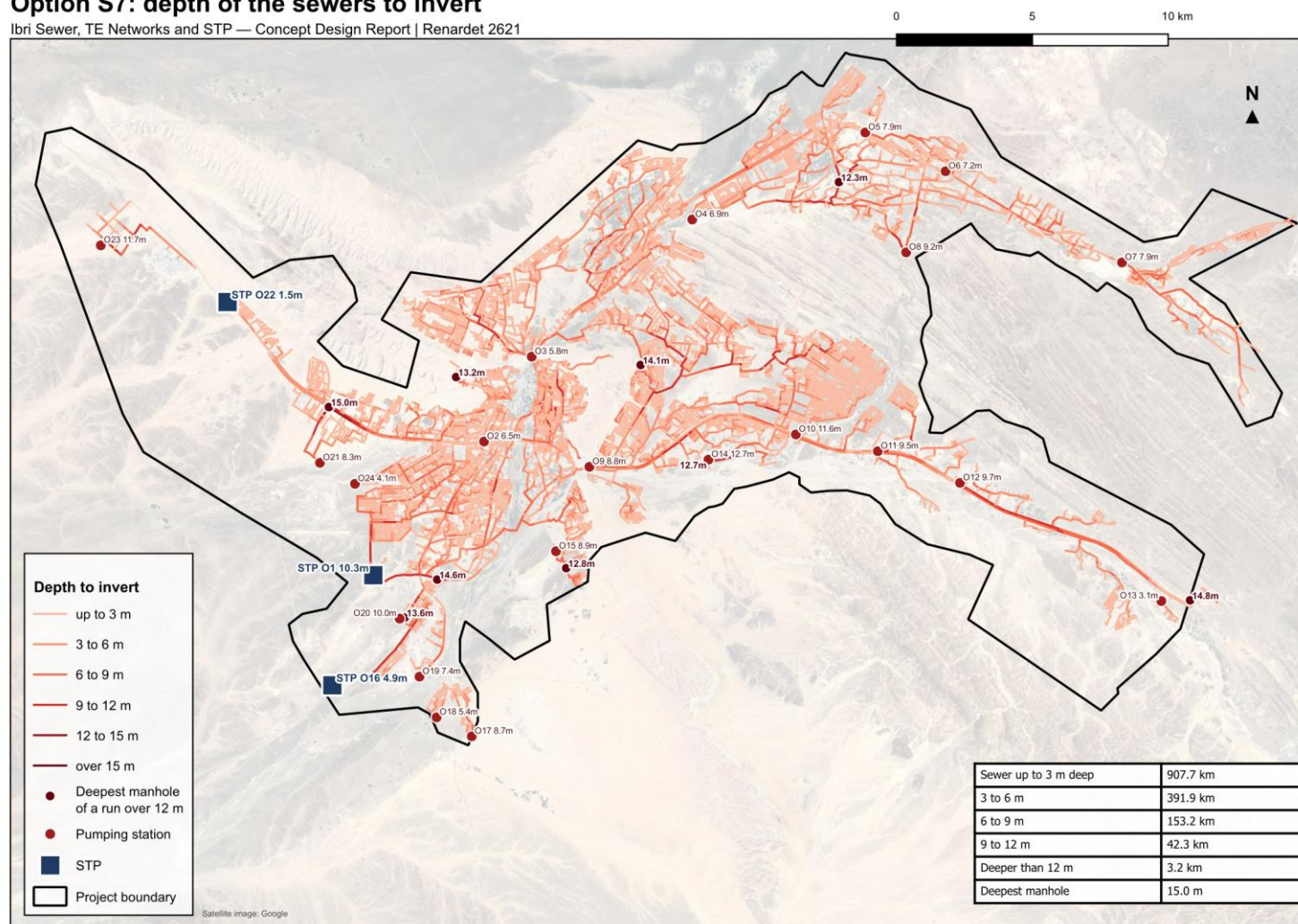
Figure 88. Option S7: depth of the sewers to invert in the 2070 design, the depth of each pumping station's outfall, and the deepest manhole of every run deeper than 12 m.
