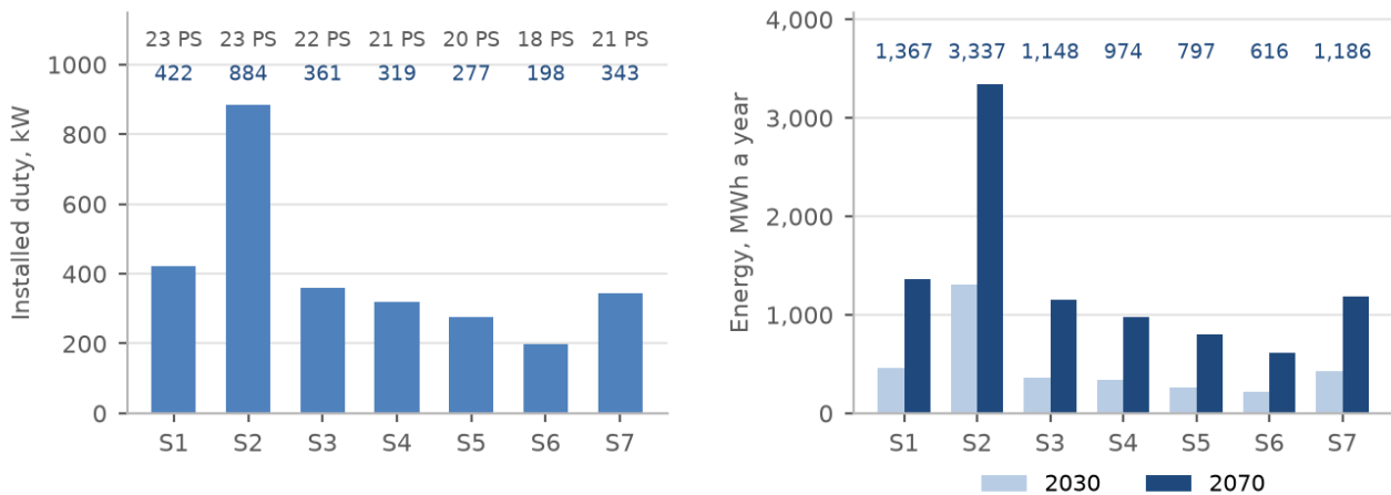
Figure 80. Pumping stations by option: the pumps in duty, and the energy they use in 2030 and 2070. The count of stations is above each bar.
