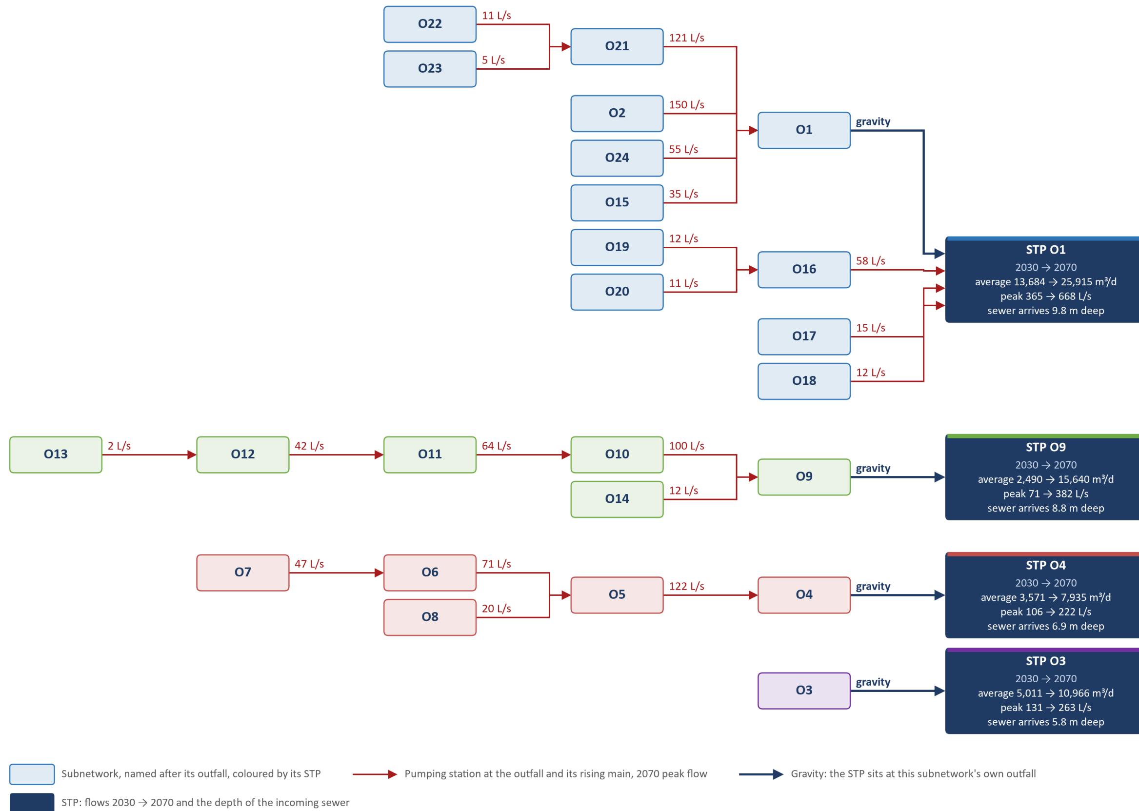
Figure 69. Option S5, four STPs, at O1, O3, O9 and O4: where the flow of every subnetwork goes, with the peak flow of each transfer in 2070.
