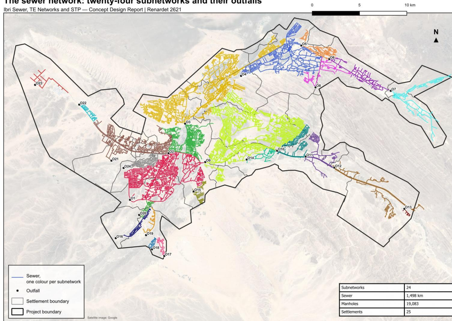
Figure 56. The twenty-four subnetworks of the sewer network, each with its outfall, and the settlement boundaries.
