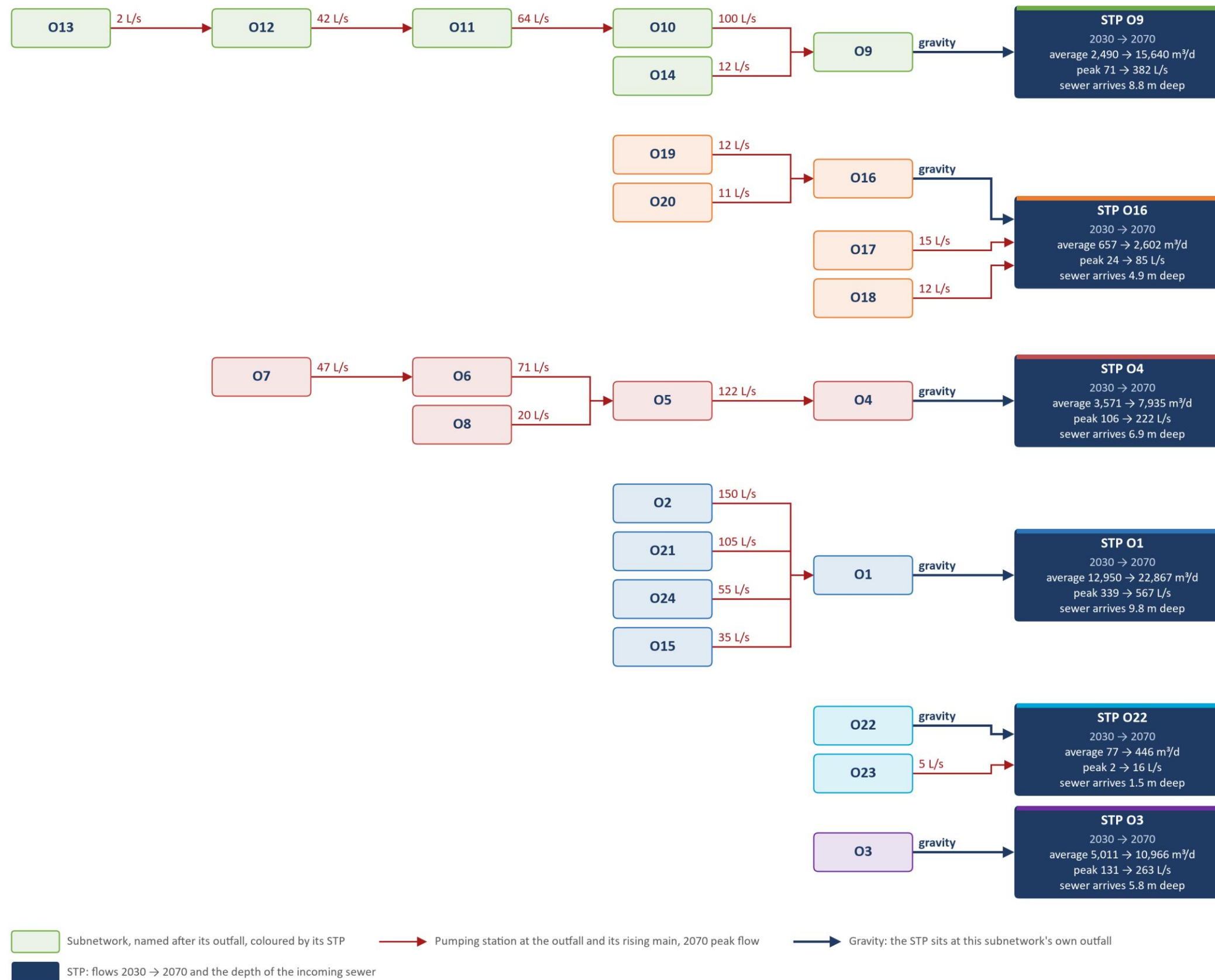
Figure 72. Option S6, six STPs, at O1, O3, O9, O4, O16 and O22: where the flow of every subnetwork goes, with the peak flow of each transfer in 2070.
