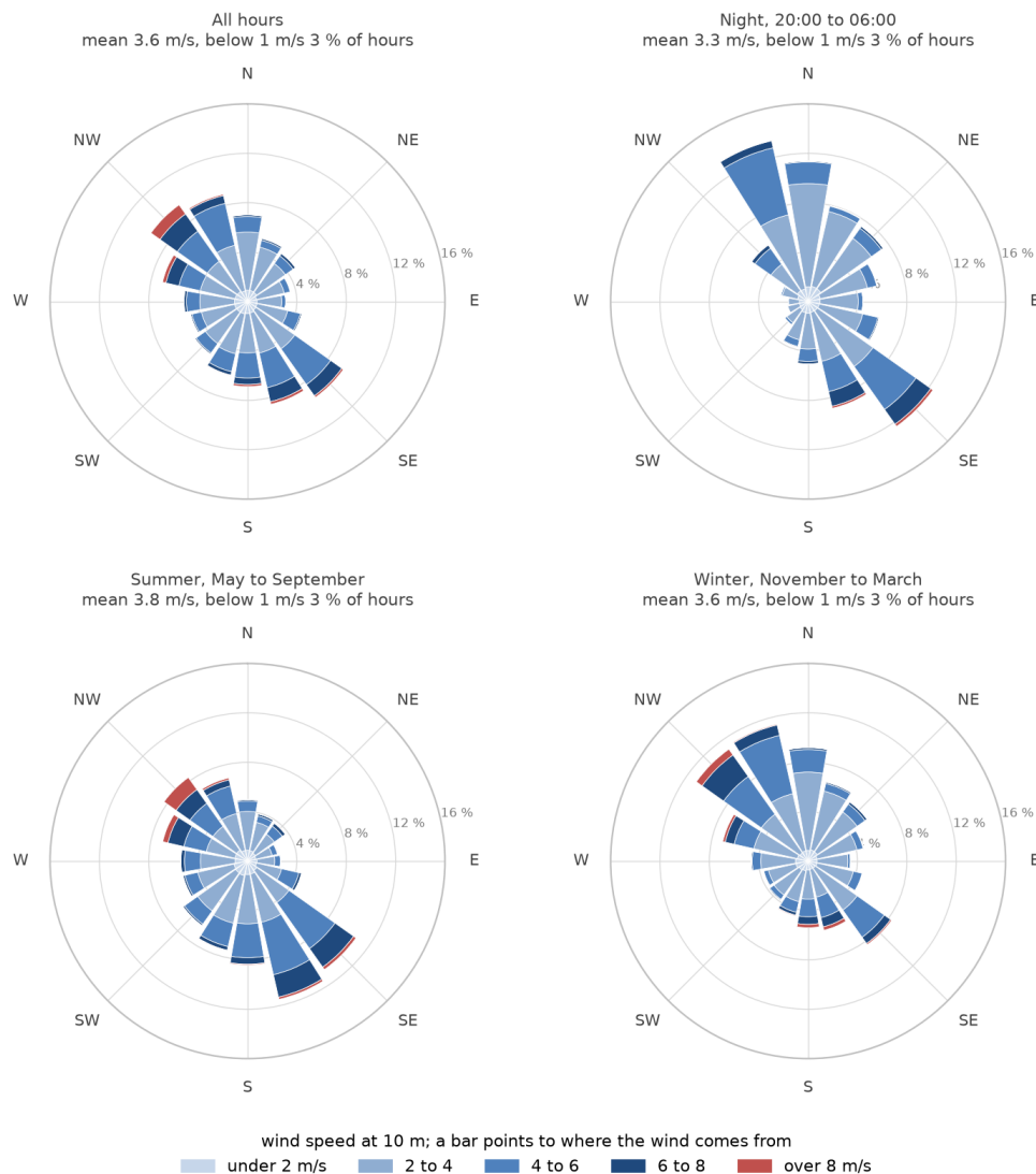
Figure 7. Wind roses at 10 m at the existing STP, 2015 to 2024: the direction the wind blows from and the share of hours in each speed class, for all hours, the night, the summer and the winter.
