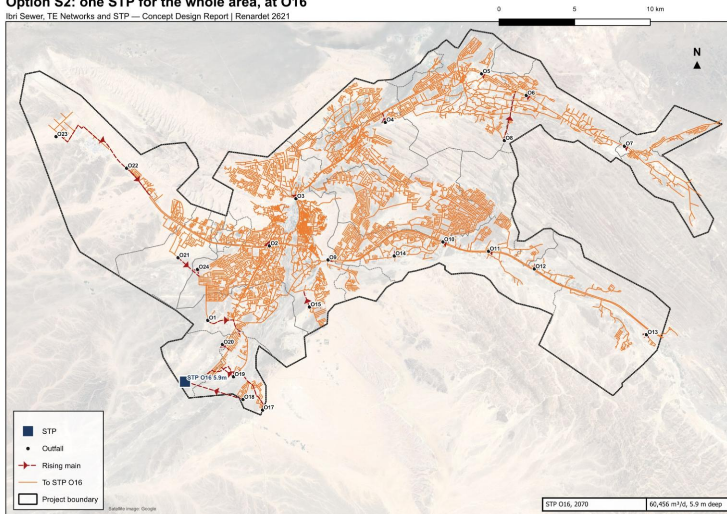
Figure 61. Option S2: the sewers by the plant they drain to, the outfalls, and the depth of the sewer arriving at each plant.
