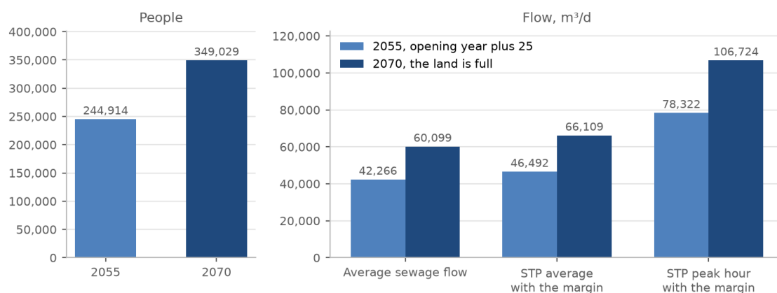
Figure 40. The two horizons side by side: people, average sewage flow, and the STP's average and peak-hour flow with the margin.
