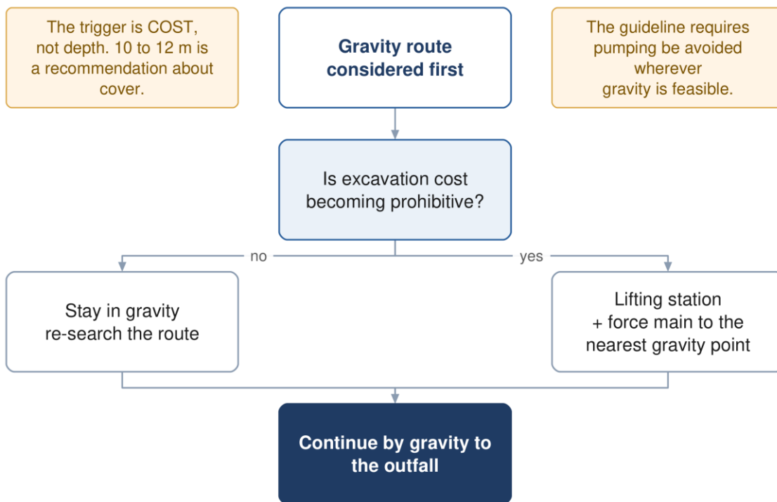
Figure 7 When a lifting station is required. The trigger is excavation cost, not depth.
