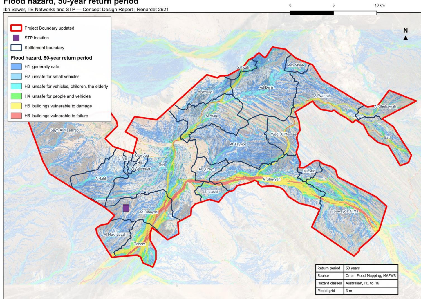
Figure 12. Flood hazard in the study area, 50-year return period. Oman Flood Mapping project, MAFWR; Australian hazard classes.
