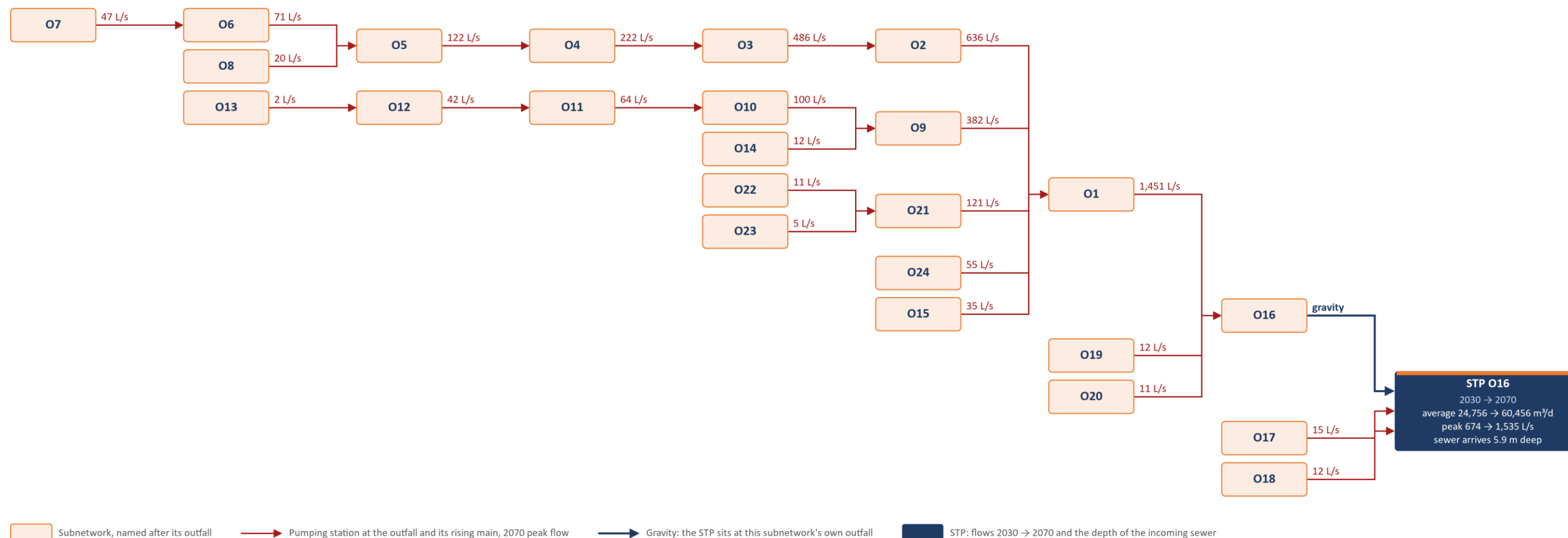
Figure 59. Option S2, one STP for the whole area, at O16: where the flow of every subnetwork goes, with the peak flow of each transfer in 2070.
