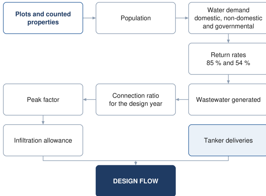
Figure 15 Derivation of the design flow, from counted properties to the flow the network is sized on.
