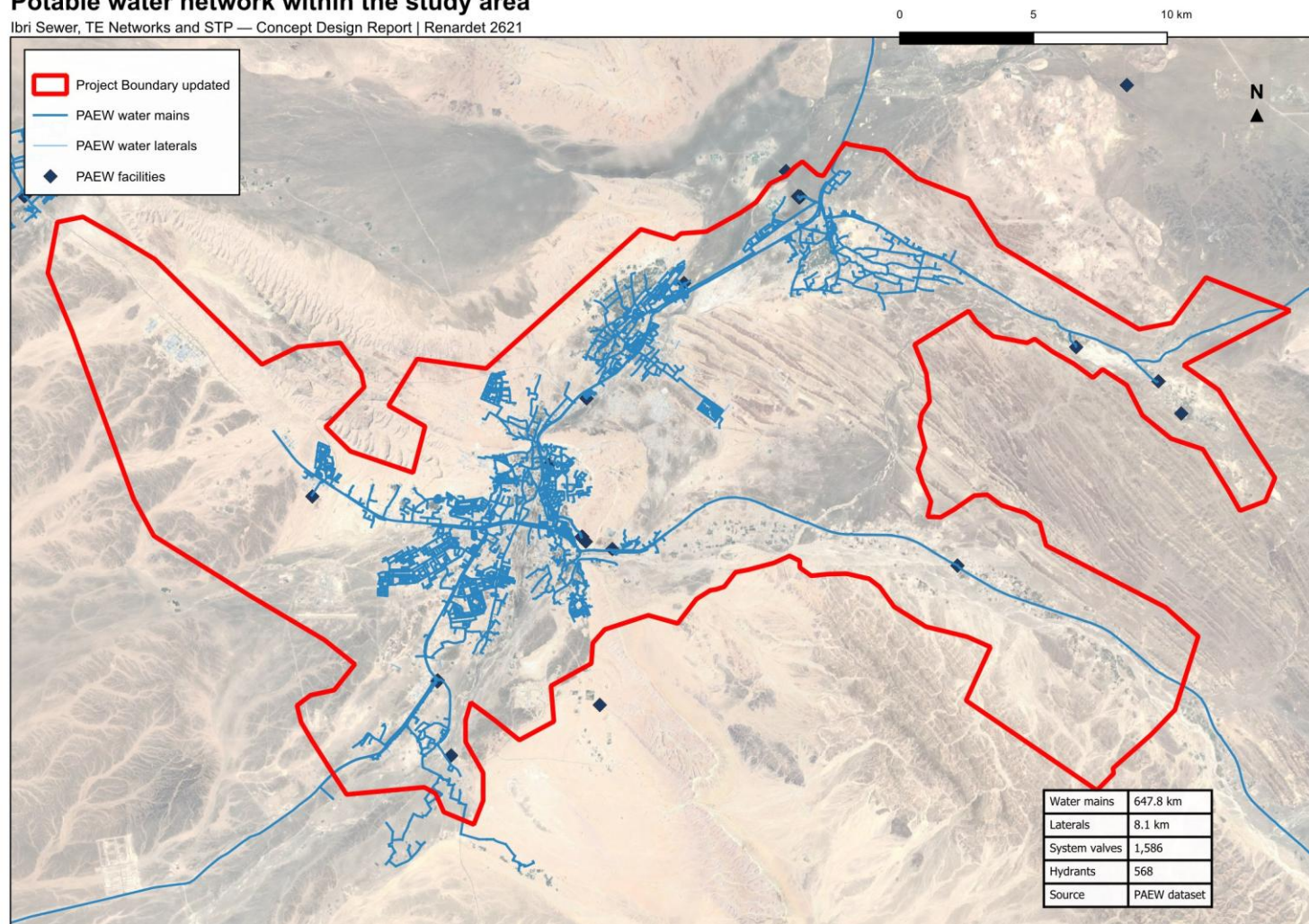
Figure 8. Potable water network within the study area, from the PAEW dataset.
