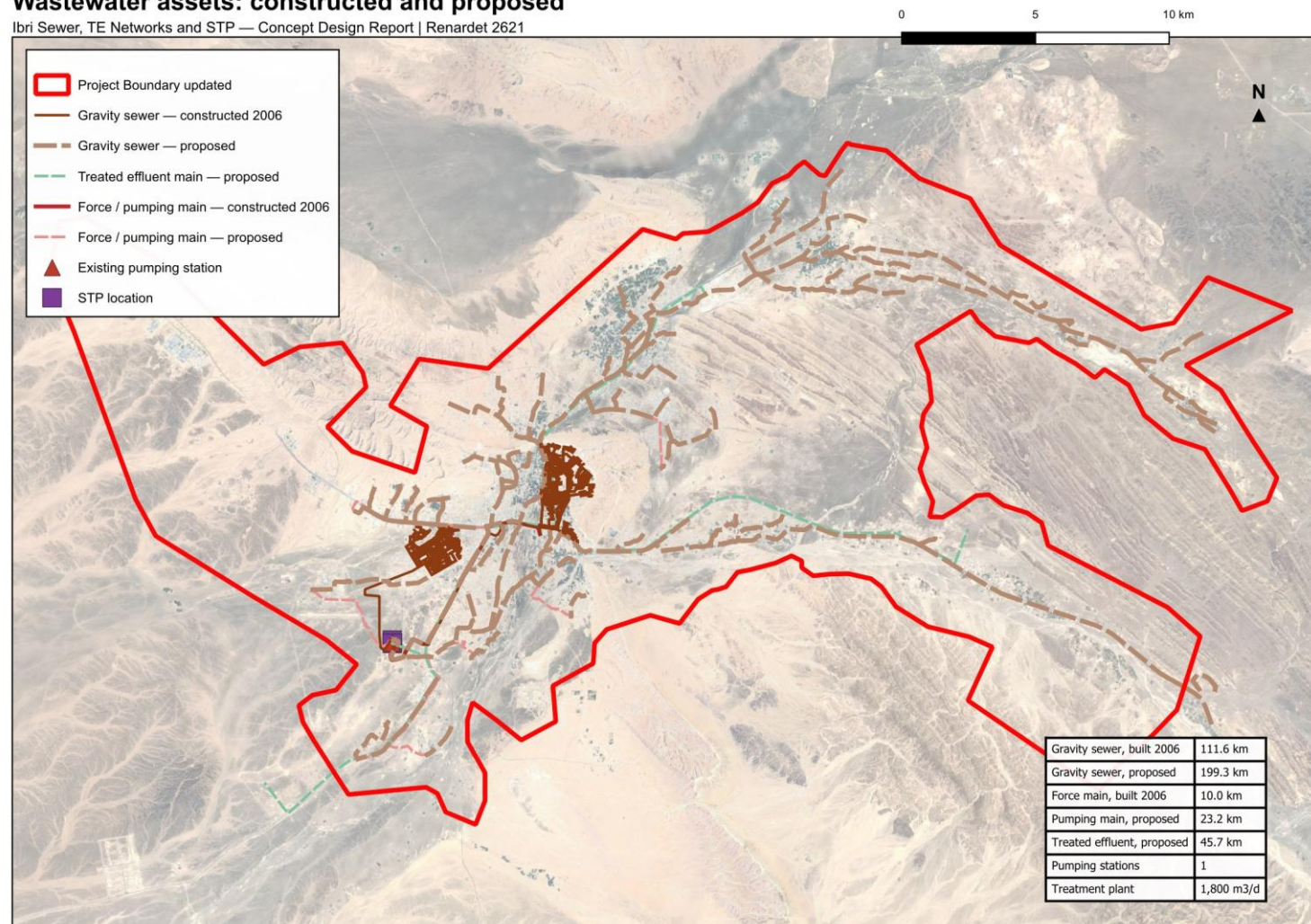
Figure 6. Wastewater assets within the study area. The constructed network, dated 2006, is shown distinctly from the alignments recorded in the dataset as proposed.
