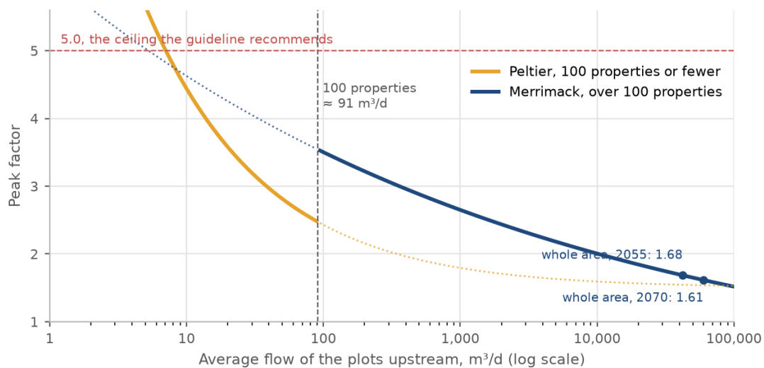
Figure 33. The peak factor against the average flow of the plots upstream. The Peltier formula applies to the head of a street, the Merrimack formula beyond 100 properties; for the whole study area the factor is about 1.6.
