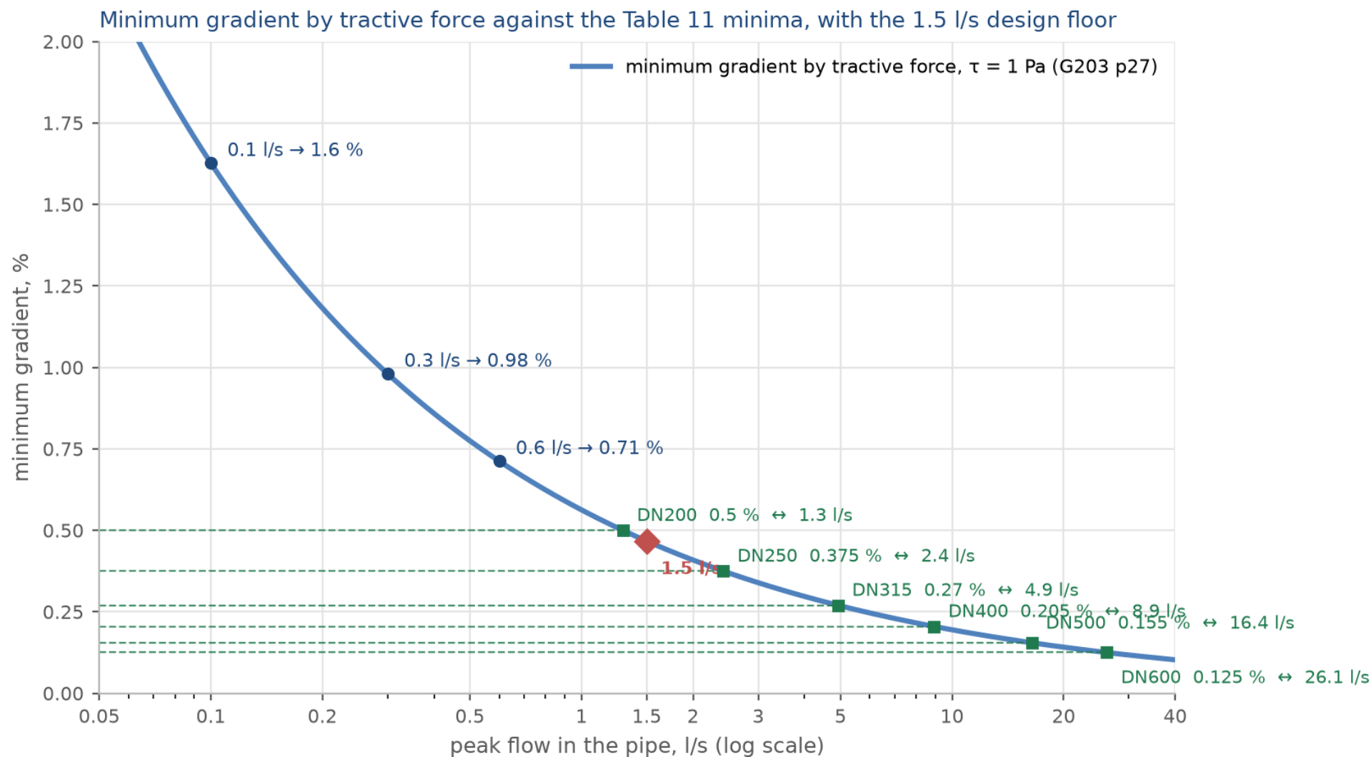
Figure 11. The minimum gradient by tractive force at one pascal against the flow in the pipe, with the Table 11 minimum of every size marked where it meets the curve, and the 1.5 l/s floor.
