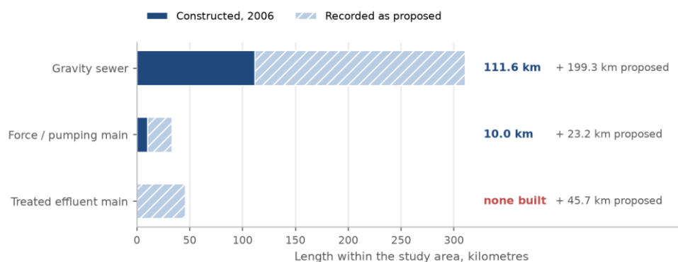
Figure 7. Length of wastewater asset within the study area, separated into constructed and proposed.
