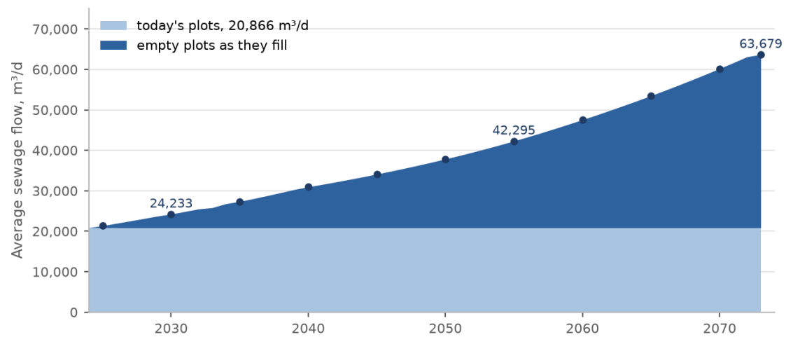
Figure 22 Average sewage flow of the study area by year, from today's plots and from the empty plots as they fill. The points mark the five-year reporting intervals.
