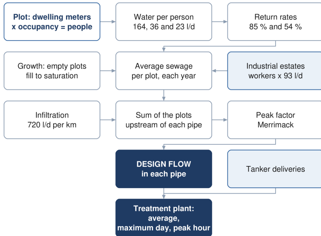
Figure 20 Derivation of the design flow, from the plot to the pipe and the treatment plant.
