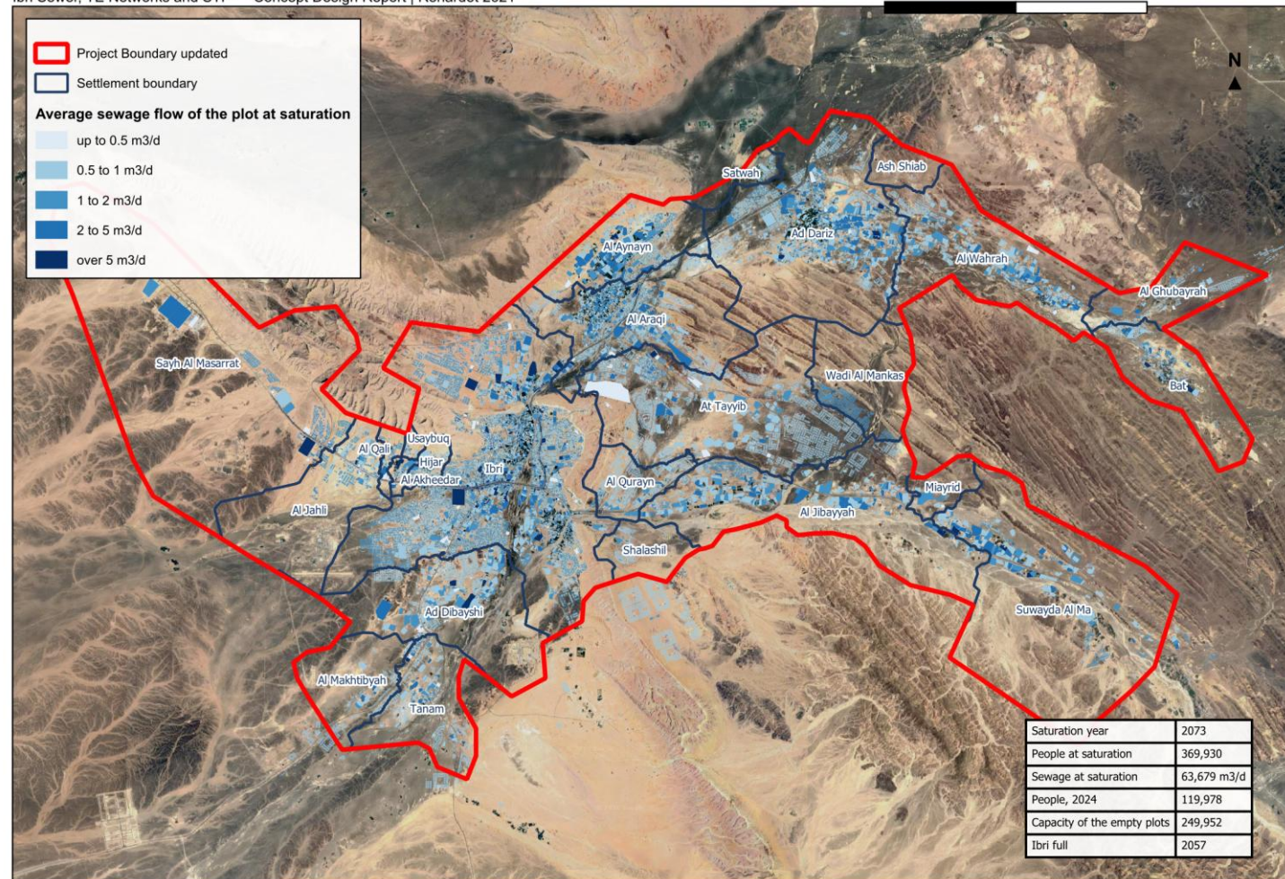
Figure 23 Average sewage flow of every plot at saturation. The network is sized on these flows, accumulated pipe by pipe.
