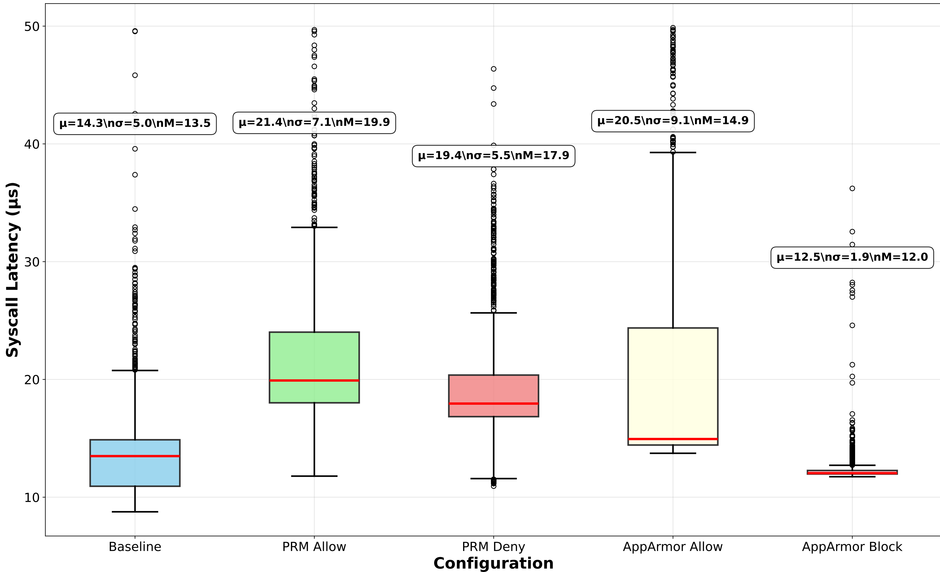
PRM eBPF LSM call / AppArmor LSM call (outliers >50μs filtered)
