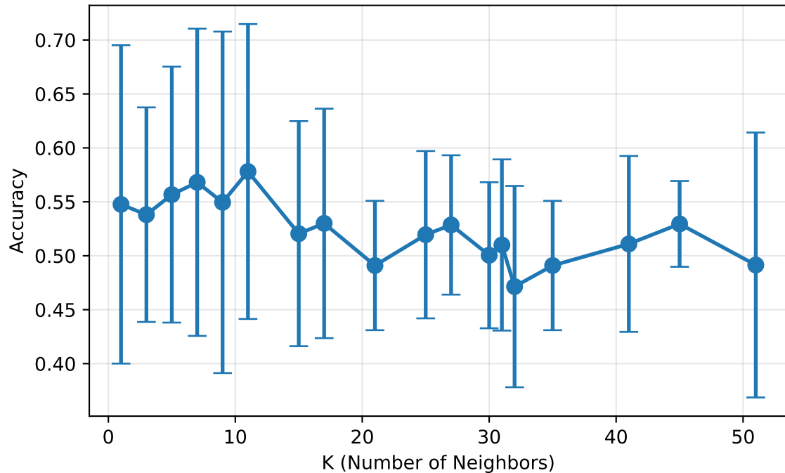
Accuracy vs K (mean \pm std across folds)
