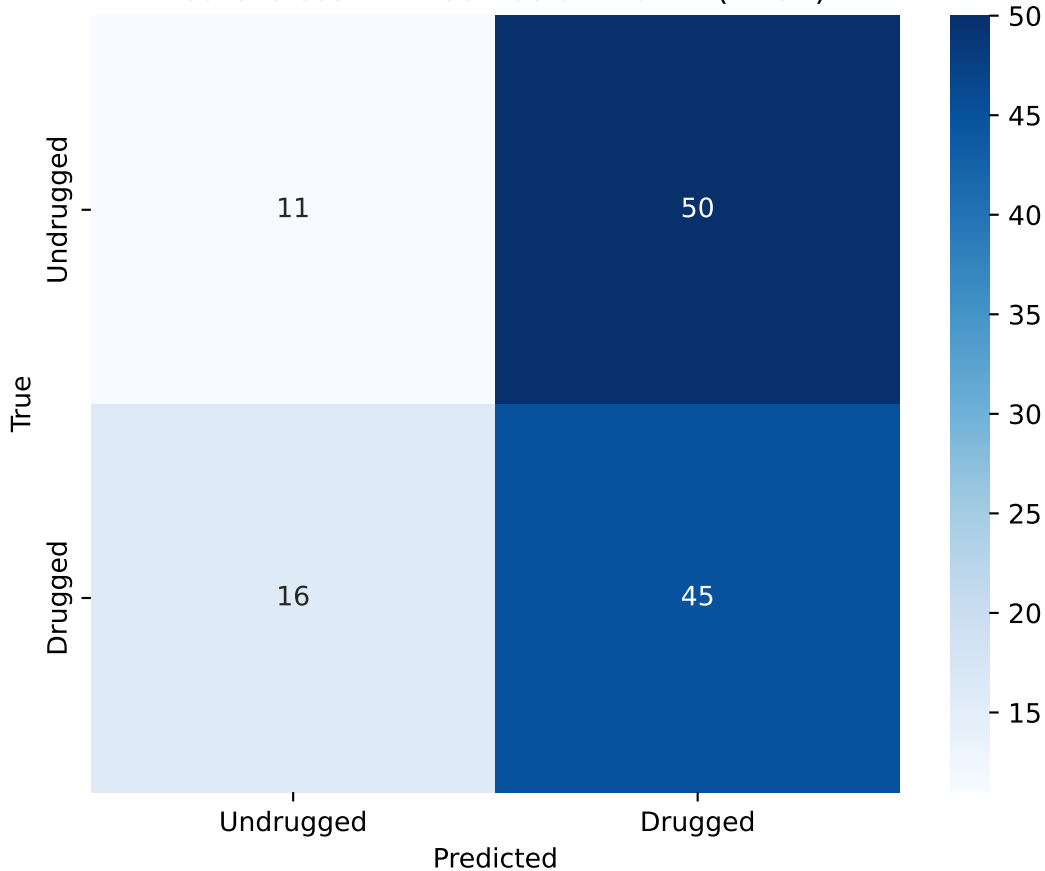
Featureless KNN Confusion Matrix (k=31)
