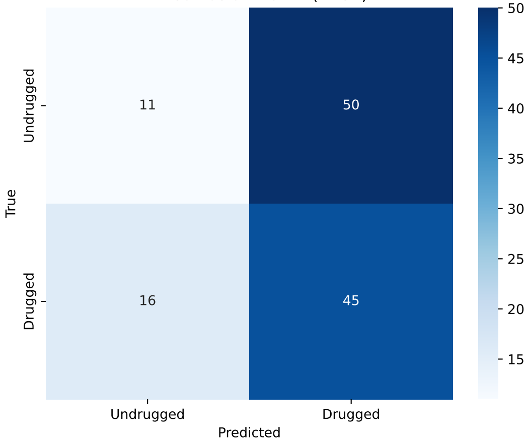
KNN Confusion Matrix (k=31)
