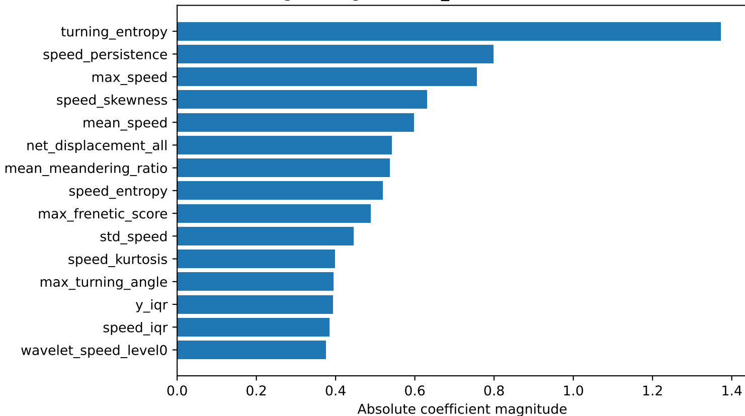
Top 15 feature importances (Logistic Regression, N_SEGMENTS=9, mode=last)
