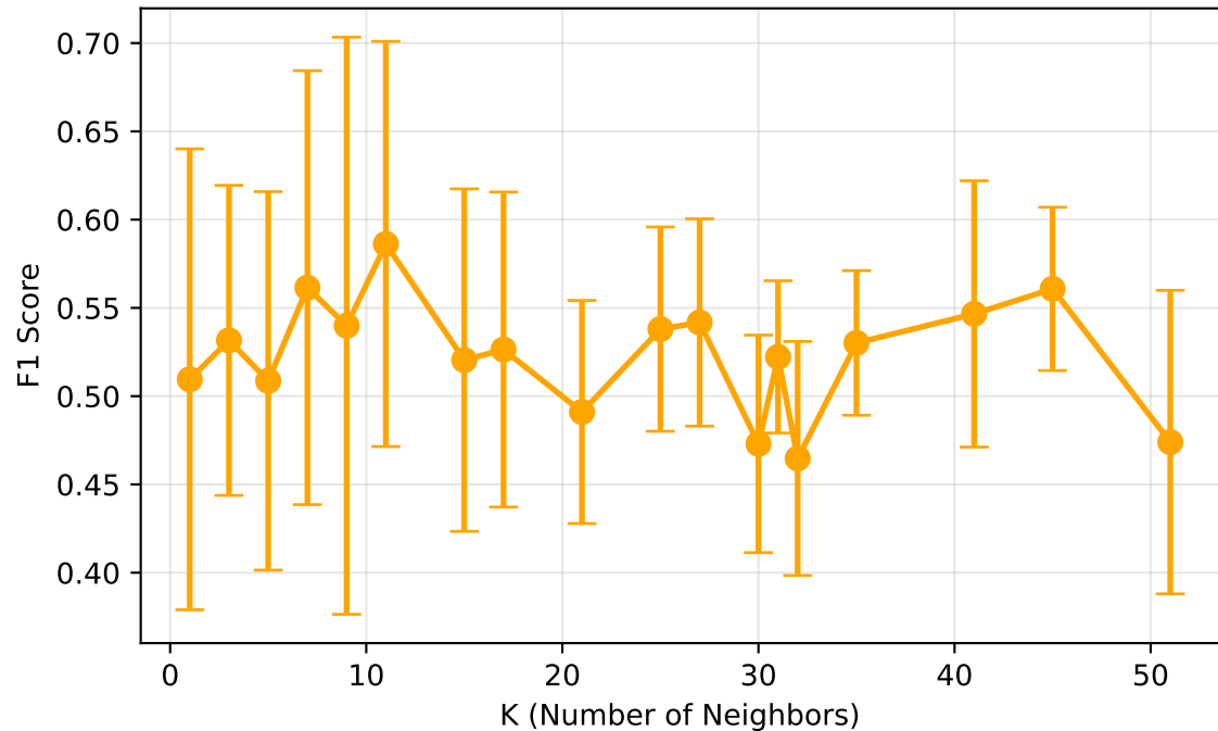
F1 Score vs K (mean \pm std across folds)
