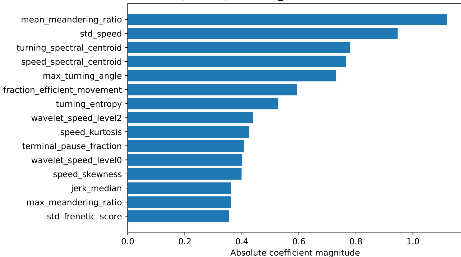
Top 15 feature importances (Logistic Regression, N_SEGMENTS=12, mode=first)
