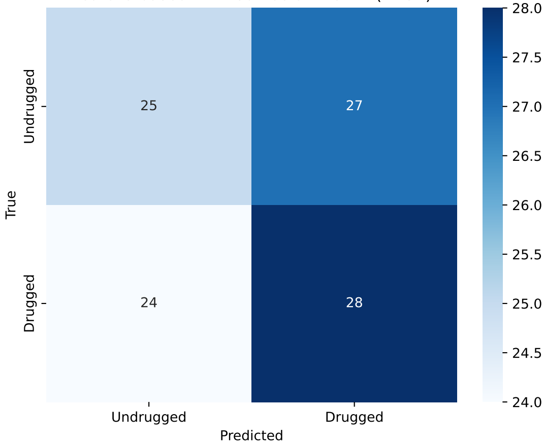
Feature-based KNN Confusion Matrix (k=31)
