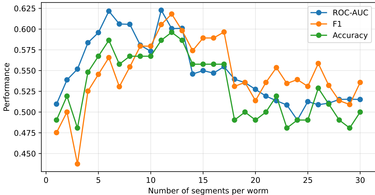
SVM performance vs segments (first)
