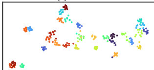
(a) Teacher
