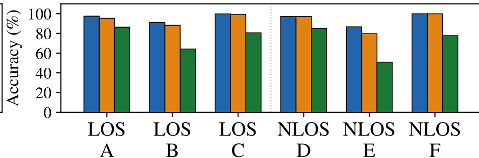
(b) SCSKNet
