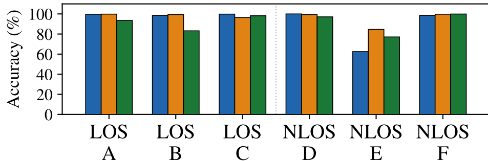
(a) ResNet18
