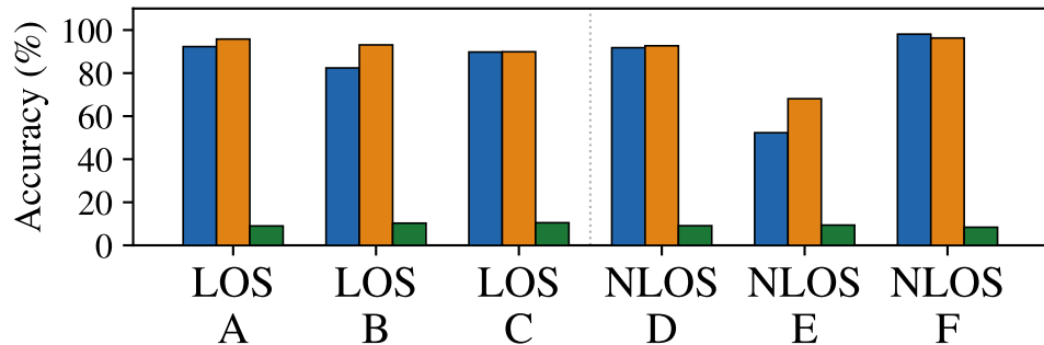
(c) ShuffleNet
