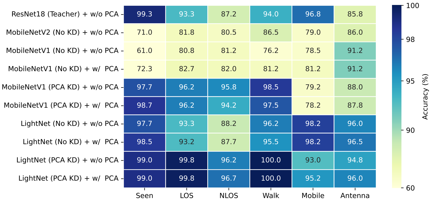
Ablation Study: Accuracy Comparison Across Scenarios
