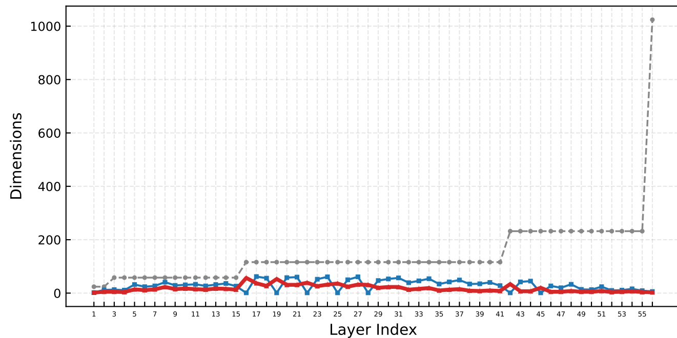
(c) ShuffleNetV2
