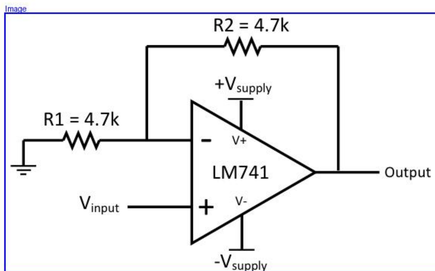
FigureCaption Figure 1. LM741 Noninverting Amplifier Circuit
