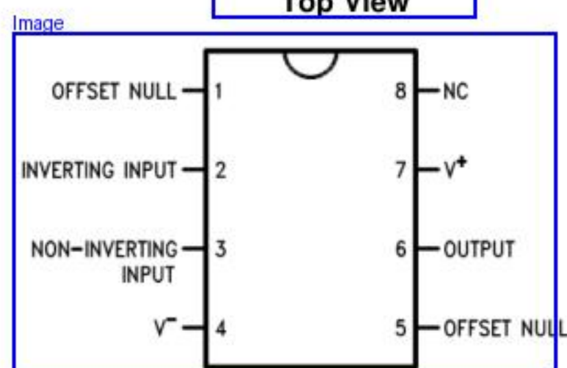
UncategorizedText NAB Package 8-Pin CDIP or PDIP Top View
