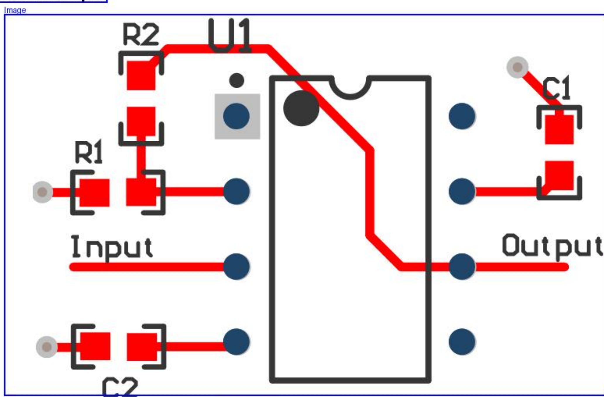
FigureCaption Figure 3. LM741 Layout
