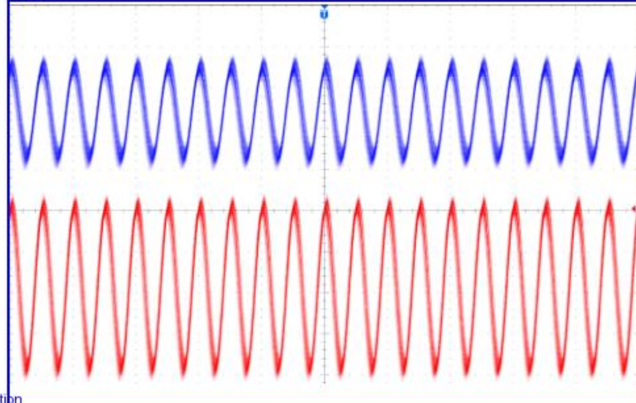
Figure 2. Waveforms for LM741 Noninverting Amplifier Circuit
