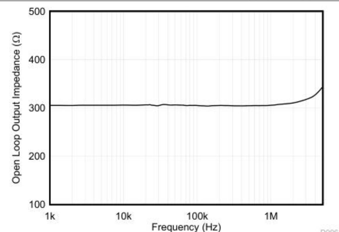
Figure 5-24. Open-Loop Output Impedance vs Frequency
