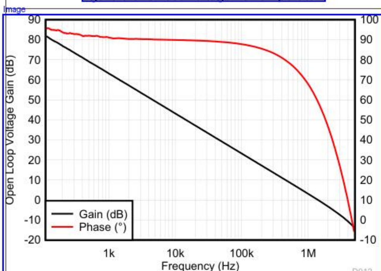
Figure 5-5. Open-Loop Gain and Phase vs Frequency
