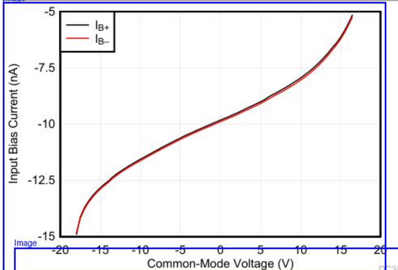
Figure 5-7. Input Bias Current vs Common-Mode Voltage
