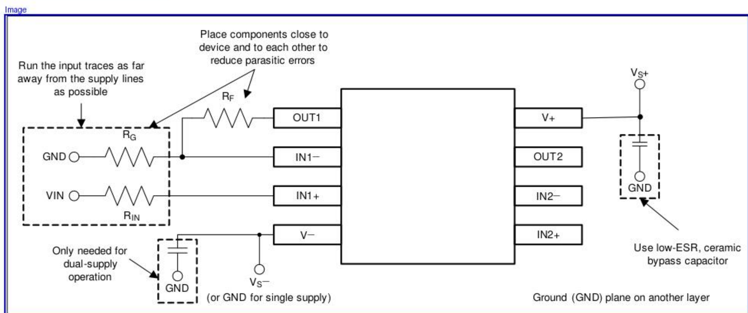
FigureCaption Figure 8-3. Operational Amplifier Board Layout for Noninverting Configuration
