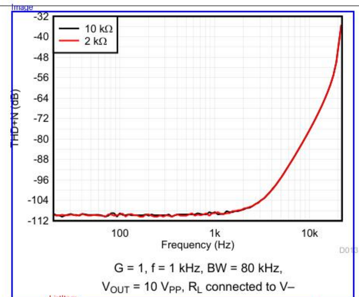
Figure 5-18. THD+N Ratio vs Frequency, G = 1
