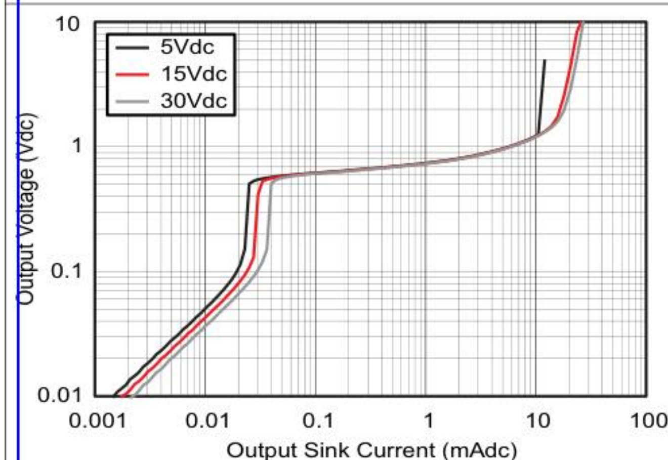
Figure 5-47. Output Sinking Characteristics
