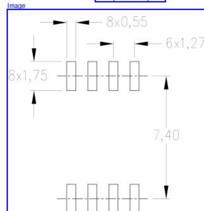
UncategorizedText Stencil Openings (Note D)
