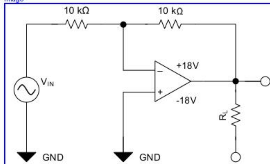
Figure 6-3. Test Circuit, G = -1 , for THD+N and Small-Signal Step Response
