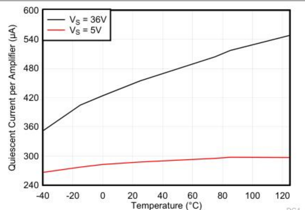
Figure 5-23. Quiescent Current vs Temperature
