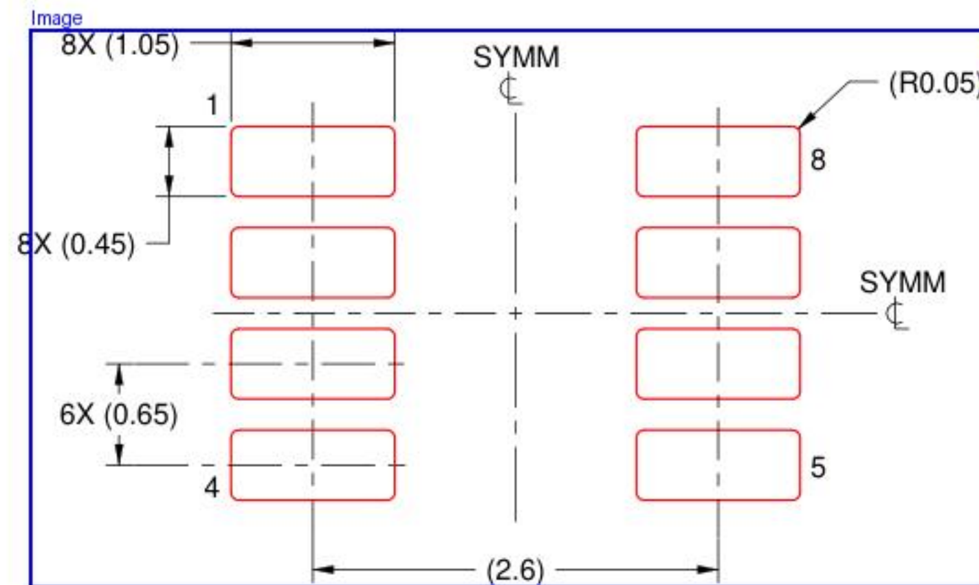
FigureCaption SOLDER PASTE EXAMPLE BASED ON 0.125 mm THICK STENCIL SCALE:15X
