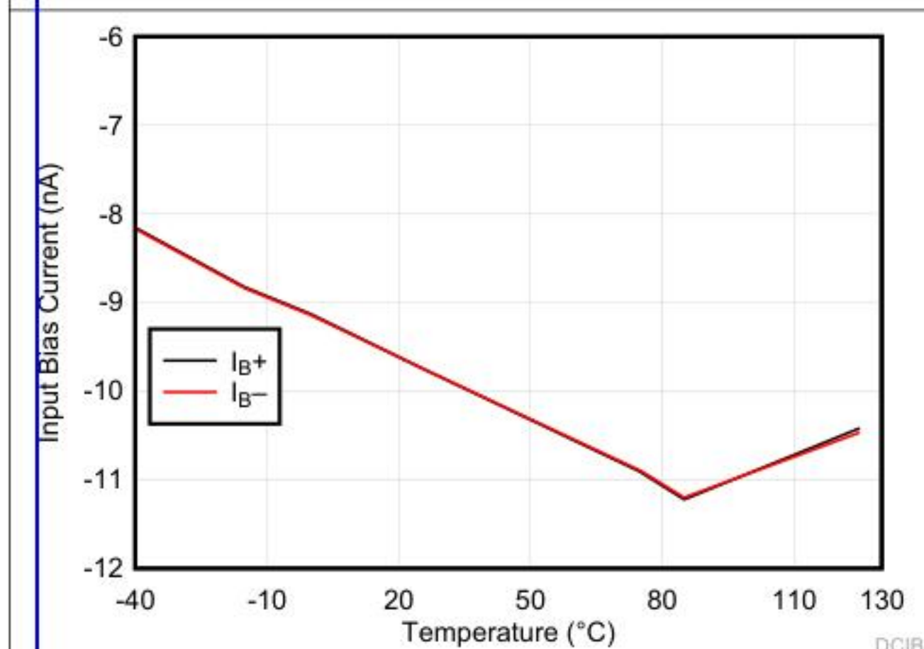
Figure 5-9. Input Bias Current vs Temperature
