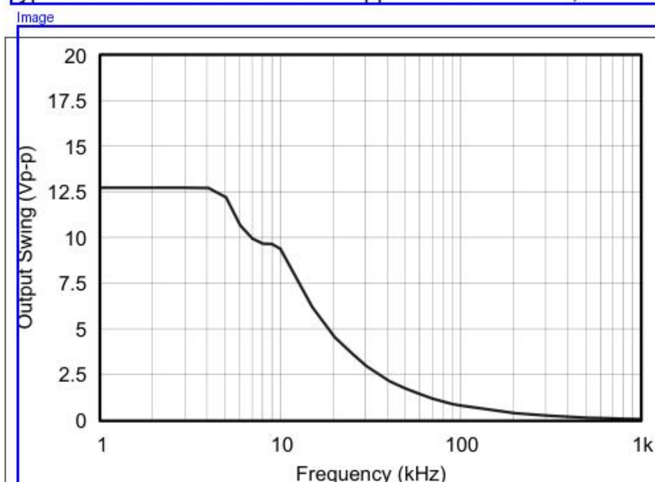
Figure 5-45. Maximum Output Swing vs Frequency ( V_{CC} = 15\text{ V} )
