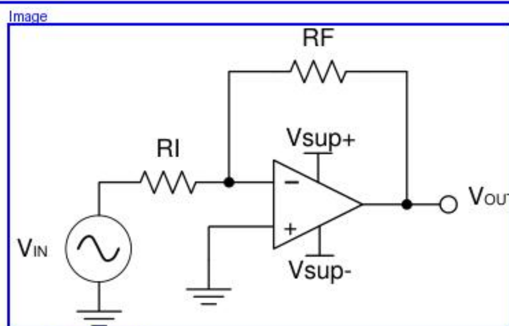
FigureCaption Figure 8-1. Application Schematic
