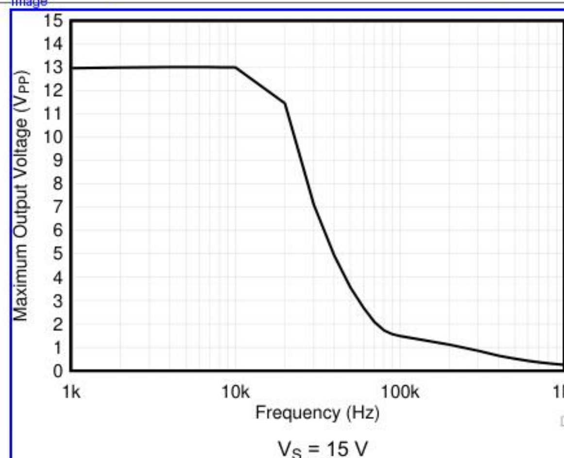
Figure 5-36. Maximum Output Voltage vs Frequency
