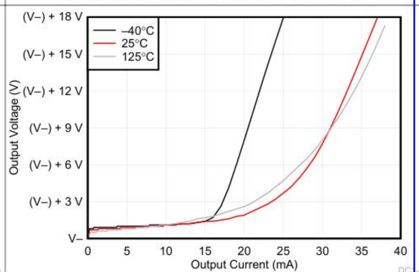
Figure 5-12. Output Voltage Swing vs Output Current (Sinking)
