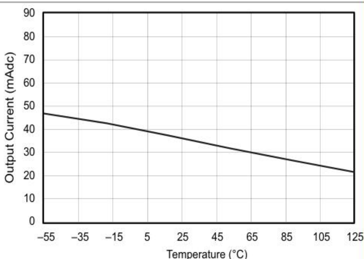
Figure 5-48. Source Current Limiting
