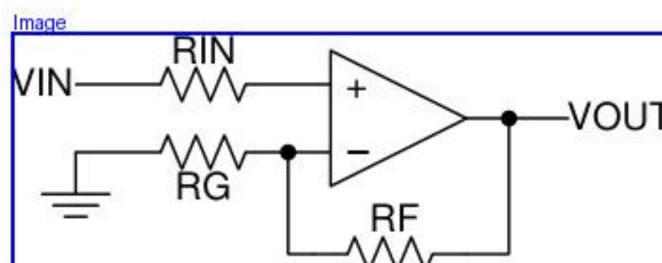
FigureCaption Figure 8-4. Operational Amplifier Schematic for Noninverting Configuration
