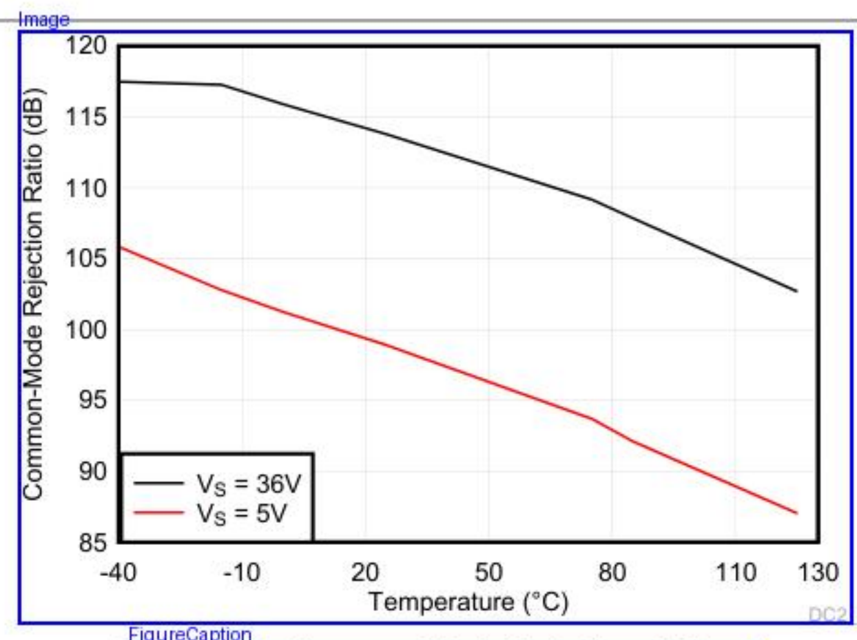
Figure 5-14. Common-Mode Rejection Ratio vs Temperature (dB)
