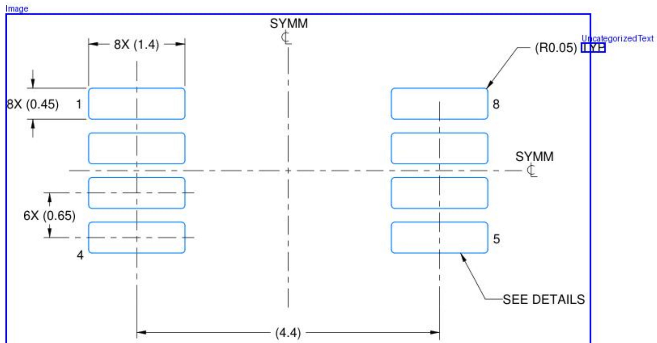
FigureCaption LAND PATTERN EXAMPLE EXPOSED METAL SHOWN SCALE: 15X
