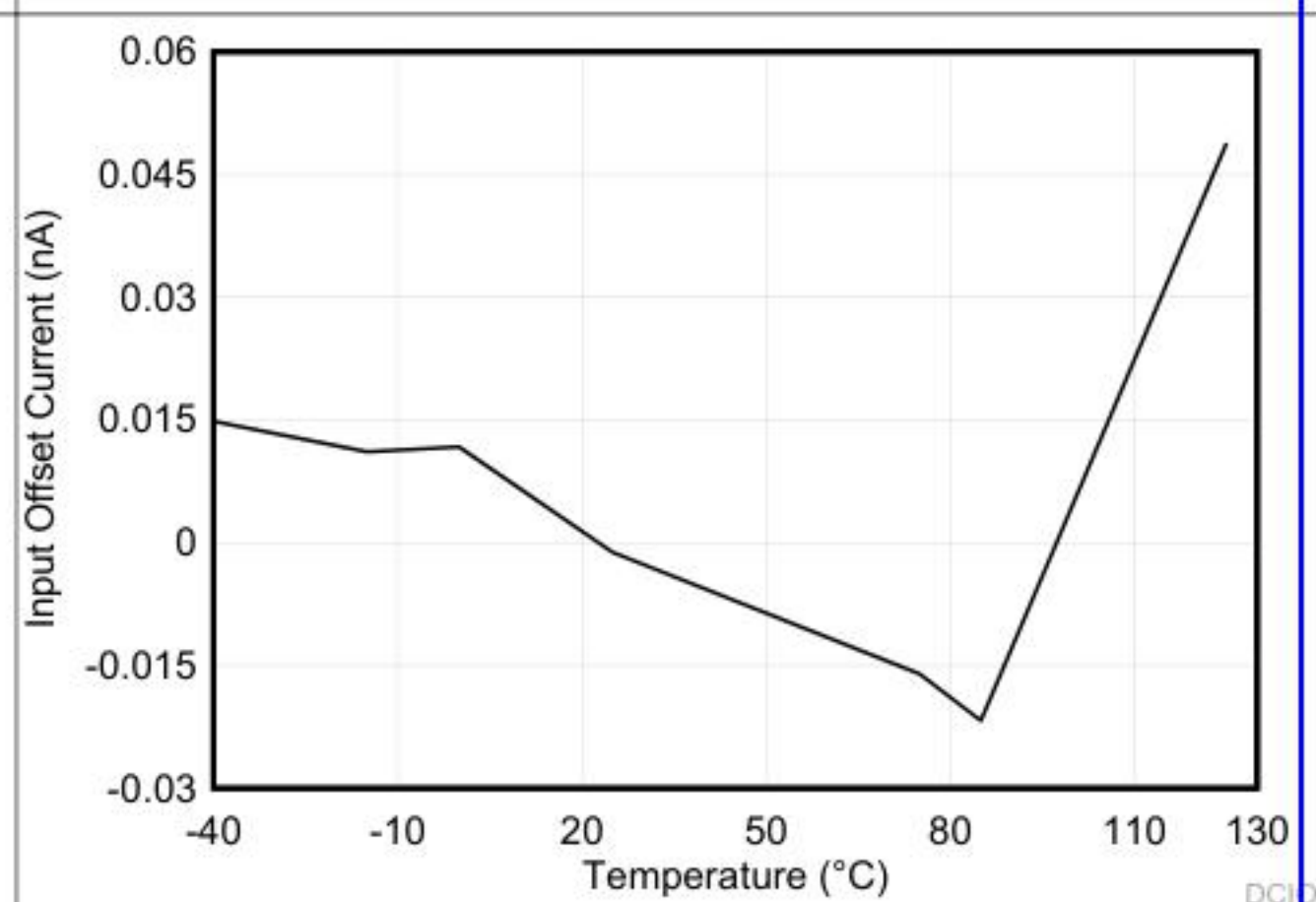
Figure 5-10. Input Offset Current vs Temperature
