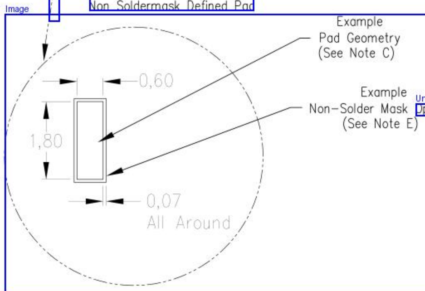
Example Non-Soldermask Defined Pad
