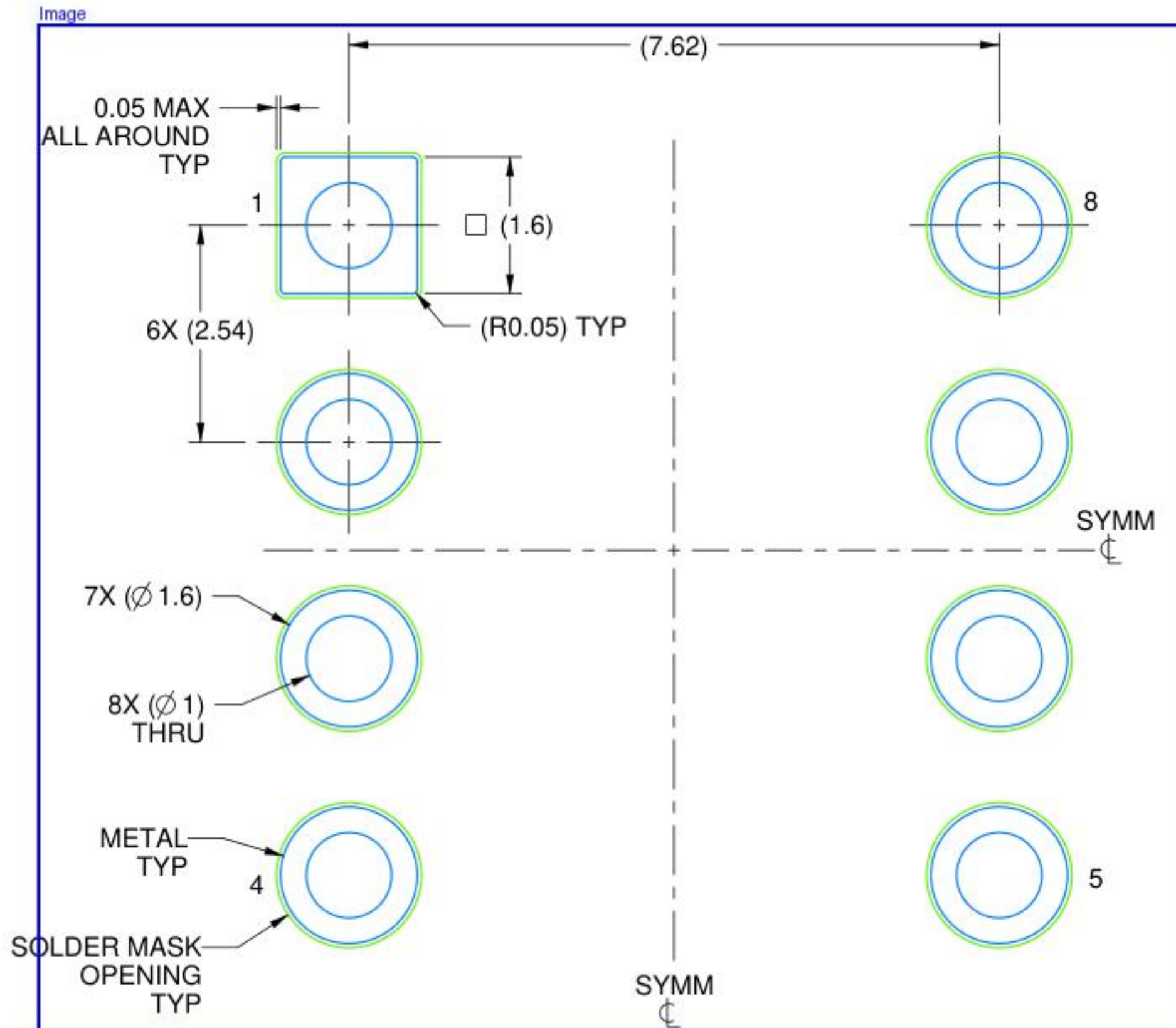
FigureCaption LAND PATTERN EXAMPLE NON SOLDER MASK DEFINED SCALE: 9X
