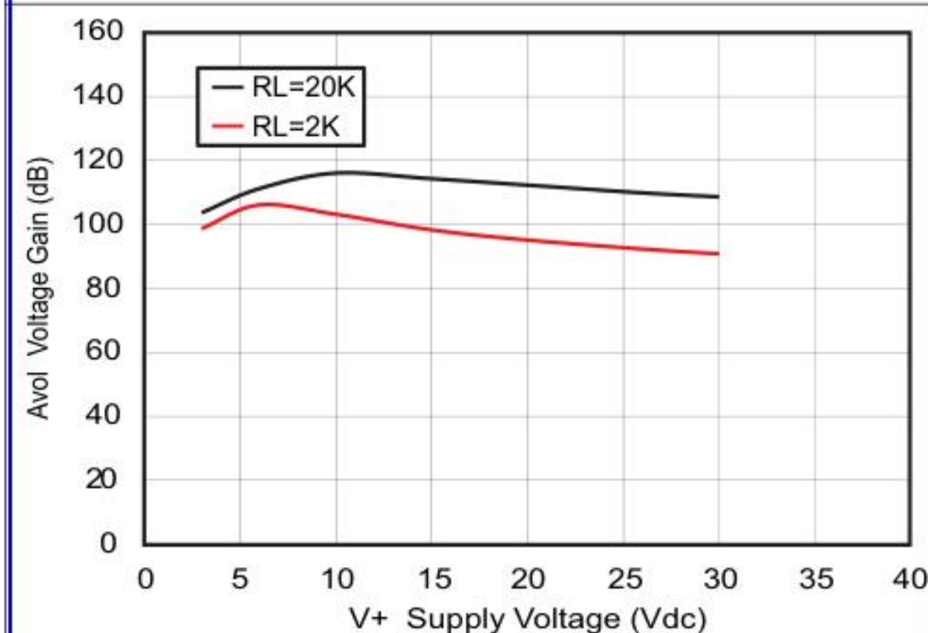
Figure 5-41. Voltage Gain vs Supply Voltage
