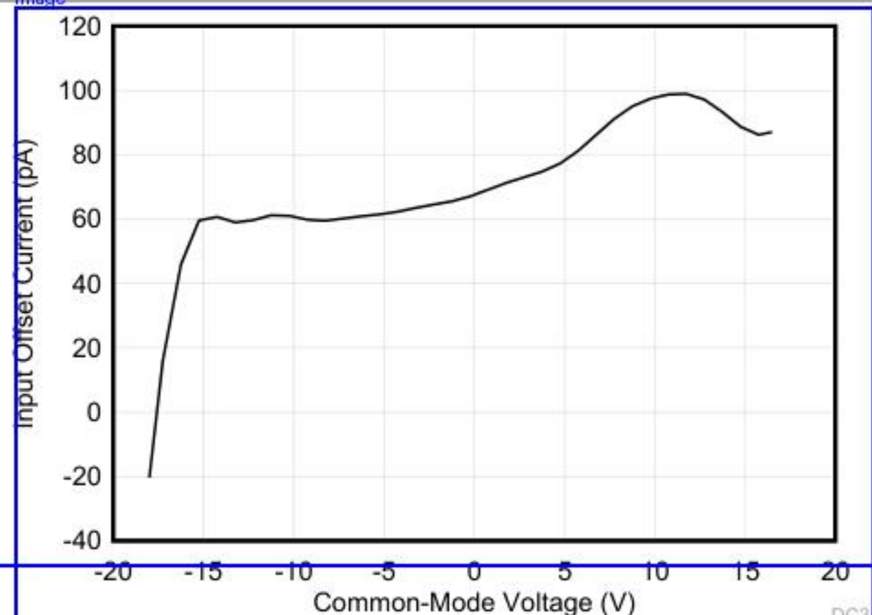
Figure 5-8. Input Offset Current vs Common-Mode Voltage
