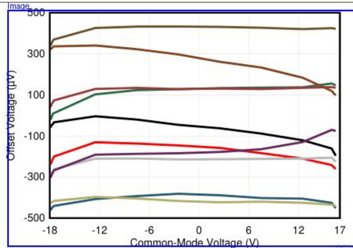
Figure 5-4. Offset Voltage vs Common-Mode Voltage
