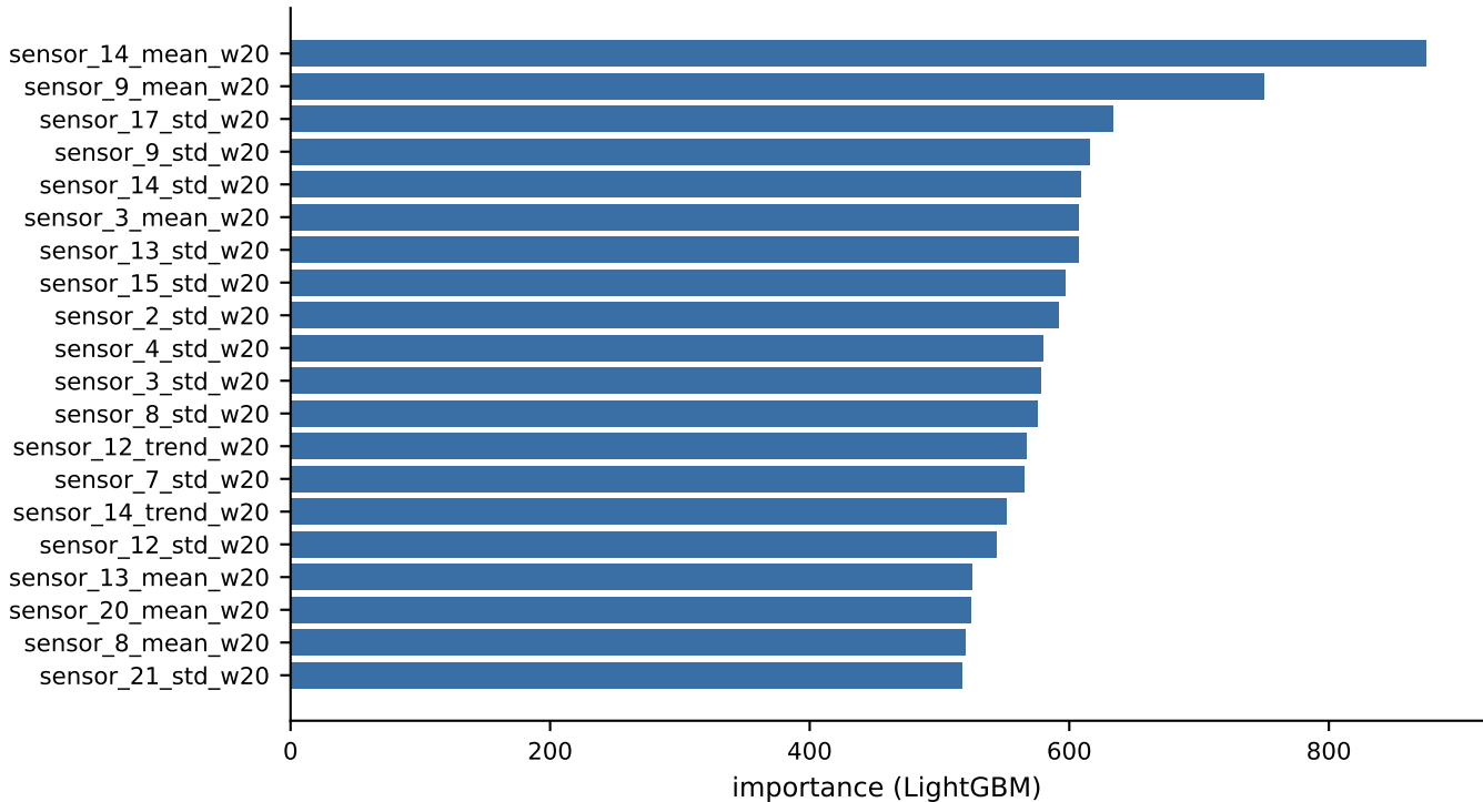
Top-20 features by importance, LightGBM on FD001
