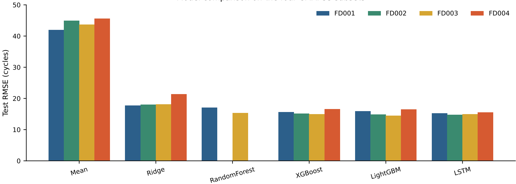
Model comparison on the four CMAPSS subsets
