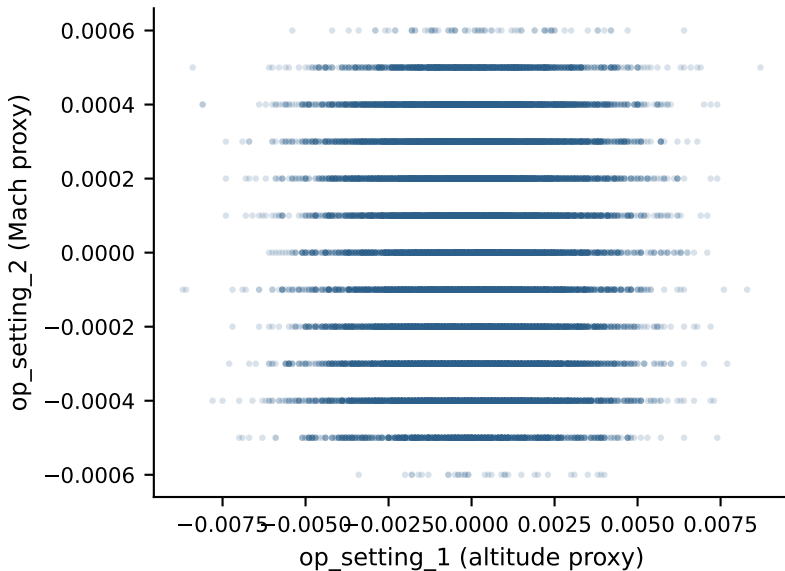
FD001 -- operational settings
