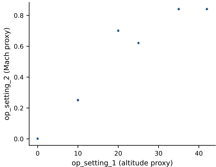
FD002 -- operational settings
